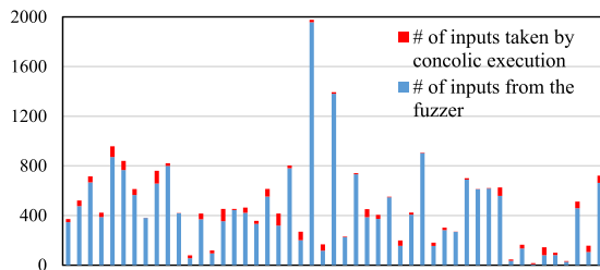
Fig. 3. The number of inputs retained by the fuzzer and the number of inputs processed by concolic execution.
