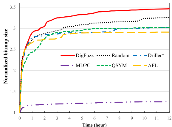
Fig. 7. Normalized bitmap size on CQE dataset.
