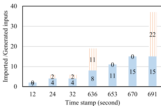
Fig. 13. Concolic executions by DigFuzz on NRFIN_00017 .
