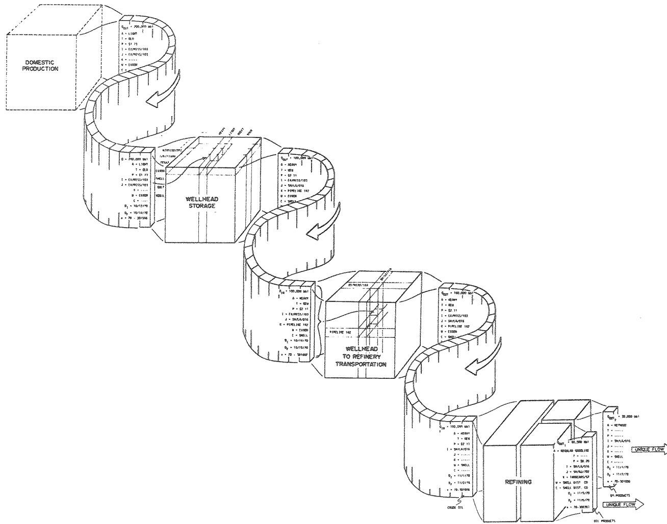
FIGURE 4. Sequential flow through connected blocks representing a portion of the Figure 2 model. Vectorial packets leaving one block flow through a sequential channel restricted to be one unit wide and impinge on the next block downstream. Such incrementation events, properly addressed to specific matrix elements within the blocks, are the only ones allowed to modify the block contents.
