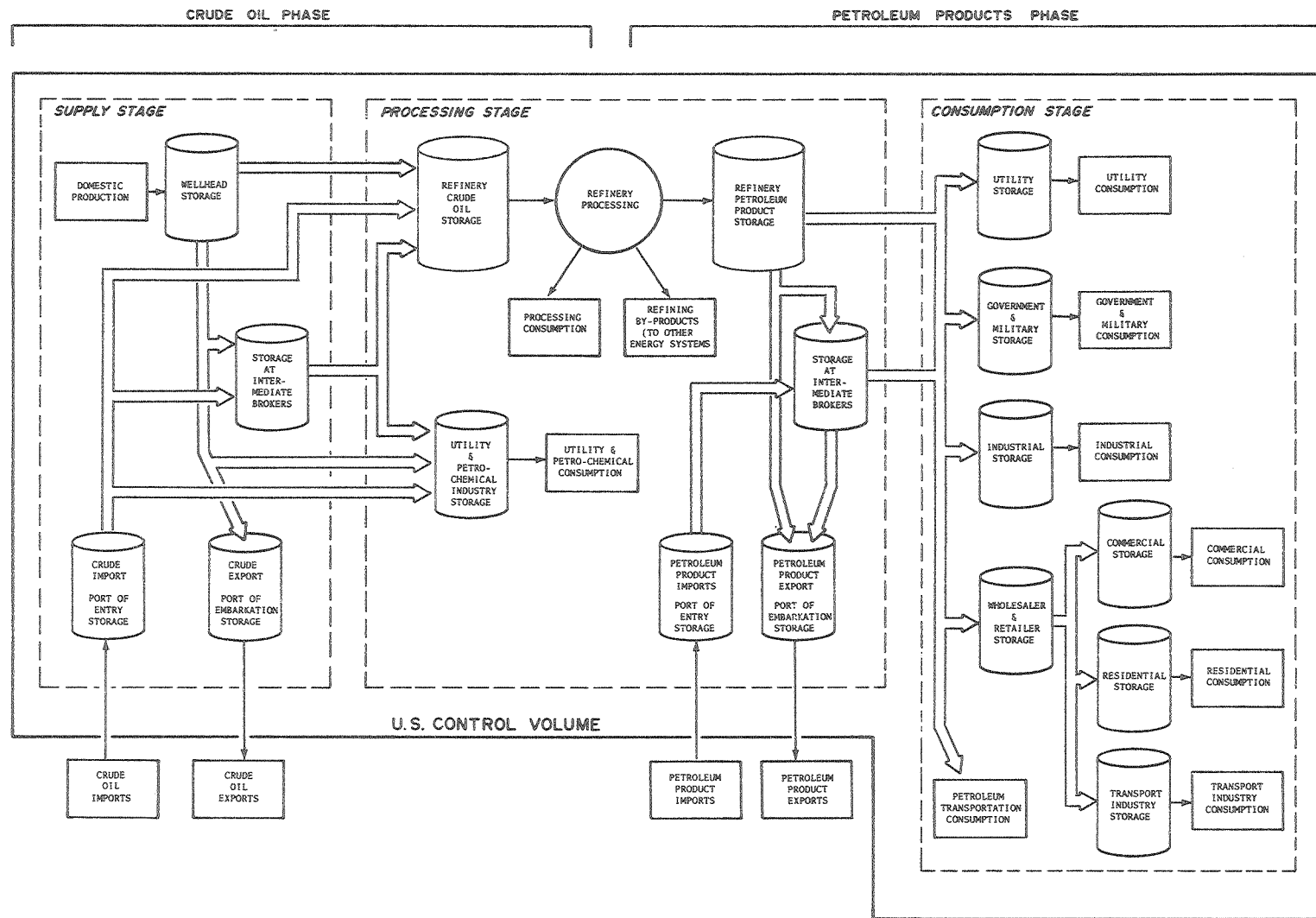
FIGURE 1. Major flows in the U.S. petroleum system. Cylinders denote matrices of storage facilities, rectangles denote material sources and sinks, circles denote material transformation sites, thick arrows denote physical transportation. Heavy boundary indicates control volume bound for U.S.; brackets and dotted lines denote material phases and processing stages as marked.
