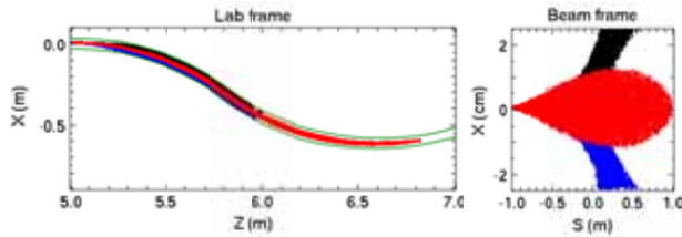
Figure 1: Particle distribution partway through the four-dipole chicane, and downstream of the stripper. Red: q=12 , blue: q>12 , black: q<12 . The initial current of the beam was reduced by a factor 10^{-6} from the nominal case to 11 \mu\text{A} . At this low current, only the q=12 ions pass through the aperture downstream of d2 and all other charge states are rejected.
