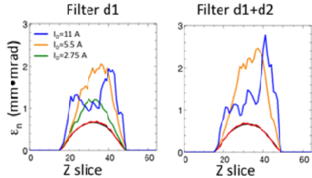
Figure 2: Emittance of the beam after the stripper, and partway through the four-dipole chicane. The left and right plots show the emittance after d1 and after d2 respectively. The green, orange and blue curves correspond to the downstream emittance for different initial currents, as indicated by the legend.
