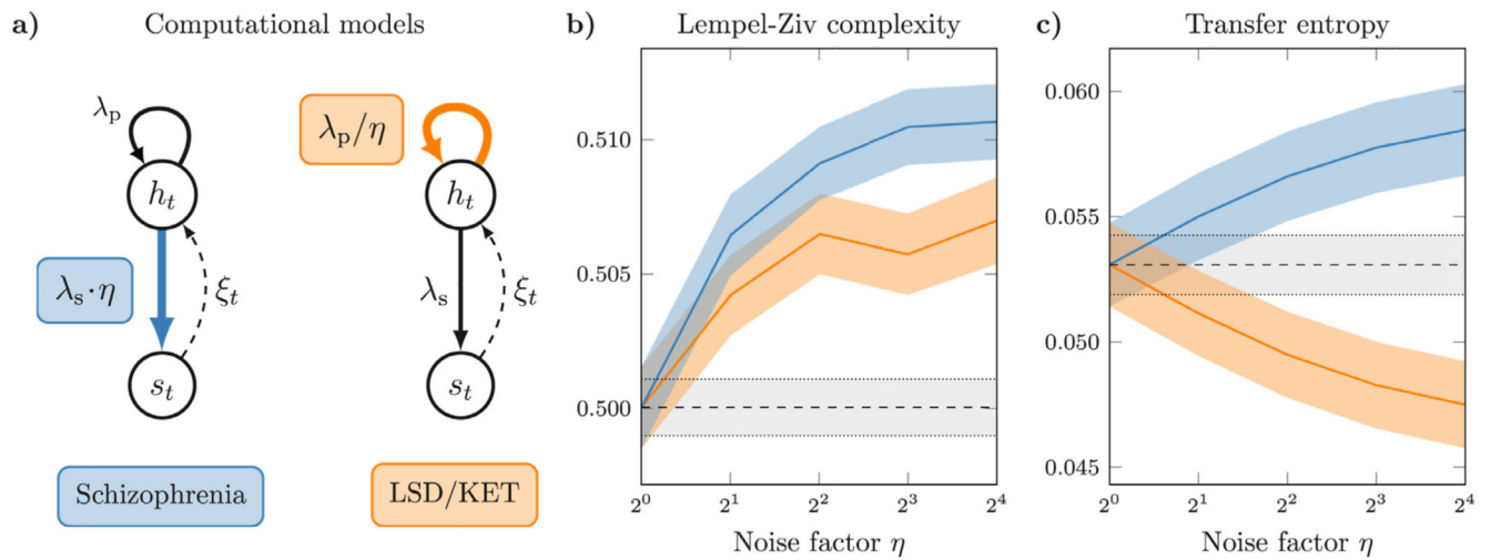
Fig. 5. A computational model based on predictive processing principles reproduces experimental findings in the LSD, ketamine and schizophrenia datasets
