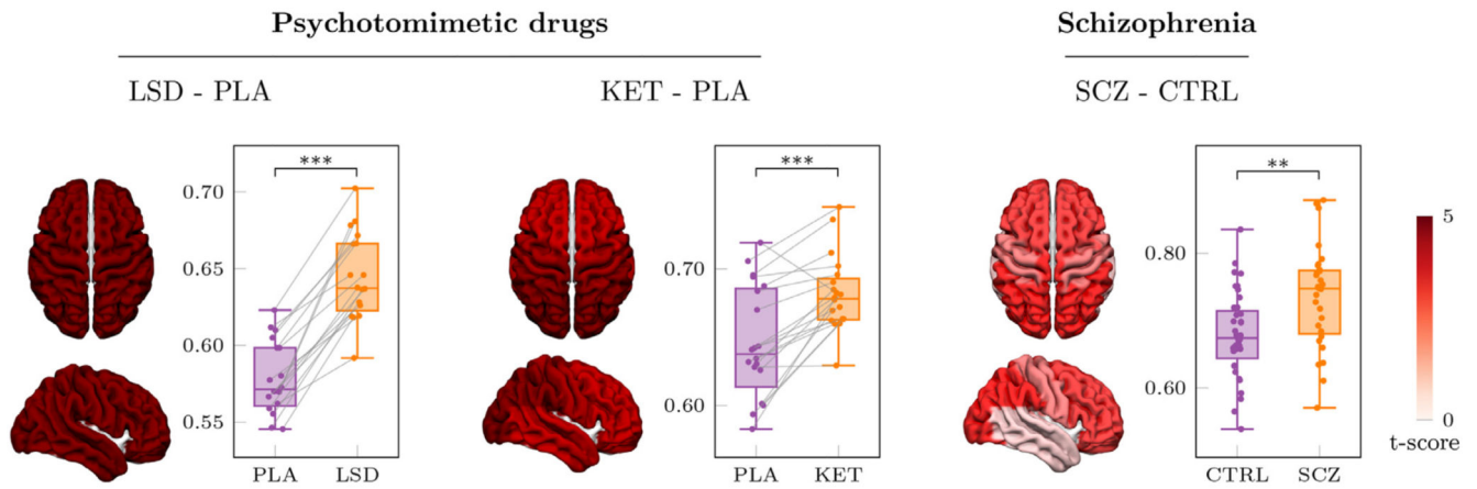
Fig. 3. Increased signal diversity in subjects under the effects of psychotomimetic drugs and in schizophrenia patients.
