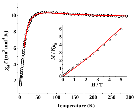
Fig. 3 \chi_{\text{M}}T vs. T and M vs. H (inset) plots for 1 ·2H 2 O. The red solid lines correspond to the fit of the experimental data using a complete 4- J spin Hamiltonian; see the text for the obtained fit parameters.
