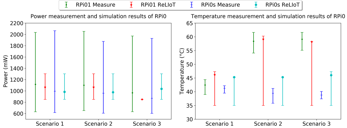
Figure 2.4. Collected and simulated statistics of RPi0s (average, max, and min values).
