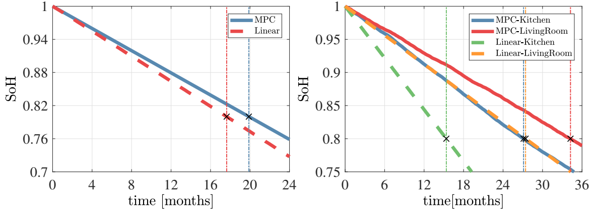
Figure 5.5. Minimum SoH in the network simulated until the end of battery life for HPWREN (left) and Smart Home (right)
