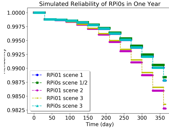
Figure 2.5. Reliability degradation of RPi0s in one year.
