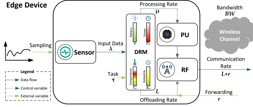
Figure 3.7. Structure of the edge device
