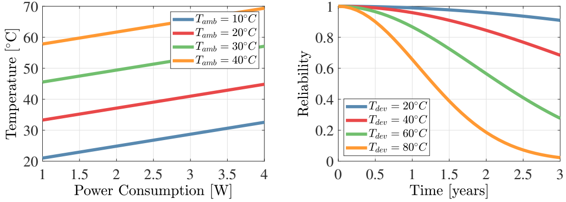
Figure 3.1. (a) Device temperature as a function of power dissipation at different ambient temperatures (b) Device reliability over time
