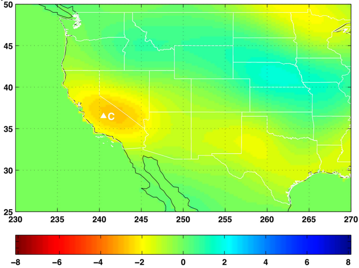
(a) Groundwater Mass Rates (cm/yr), GRACE – WGHM, 2005–2009, 300 km, West US
