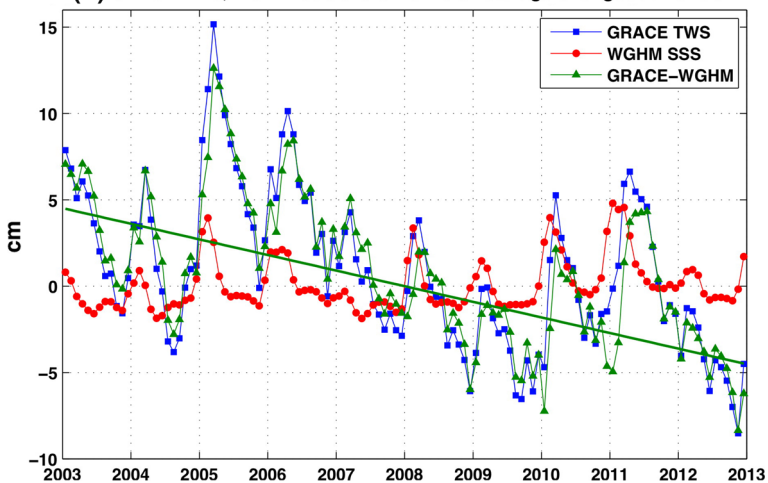
Fig. 3 a Estimated GWS change from GRACE to WGHM (in cm/year of equivalent water height) over the period January 2005–December 2009, same as Fig. 1c, but enlarged for the western and mid-western USA b Comparison of GRACE-observed TWS change, WGHM model estimates of SSS water change, and GWS change from GRACE to WGHM (in cm equivalent water height) for January 2003 through December 2012, for point C marked by white triangle on Fig. 3a
