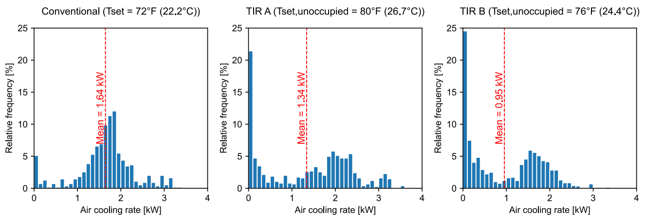
Figure 6 Histogram of air-cooling rate under each control algorithm when the conference room was occupied. TIR control A ( T_{\text{set, unoccupied}} = 80 \text{ }^{\circ}\text{F} ( 26.7 \text{ }^{\circ}\text{C} )) reduced the mean air-cooling rate by about 18% compared to the conventional control, while the TIR control B ( T_{\text{set, unoccupied}} = 76 \text{ }^{\circ}\text{F} ( 24.4 \text{ }^{\circ}\text{C} )) reduced it by 42%.
