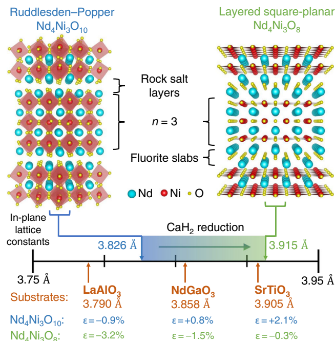
Fig. 1 | Schematic crystal structures of (left) Nd 4 Ni 3 O 10 ( n = 3 , Ruddlesden–Popper) and (right) Nd 4 Ni 3 O 8 ( n = 3 , layered square-planar). Neodymium, nickel, and oxygen atoms are depicted in blue, red, and yellow, respectively. The number line presents the bulk in-plane lattice parameters of Nd 4 Ni 3 O 10 (3.826 Å) 95 and Nd 4 Ni 3 O 8 (3.915 Å) 20 , as well as the pseudocubic lattice parameters of LaAlO 3 (001), NdGaO 3 (110), SrTiO 3 (001). The lattice mismatch between Nd 4 Ni 3 O 10 , Nd 4 Ni 3 O 8 and the three substrates are shown in blue and green, respectively.
