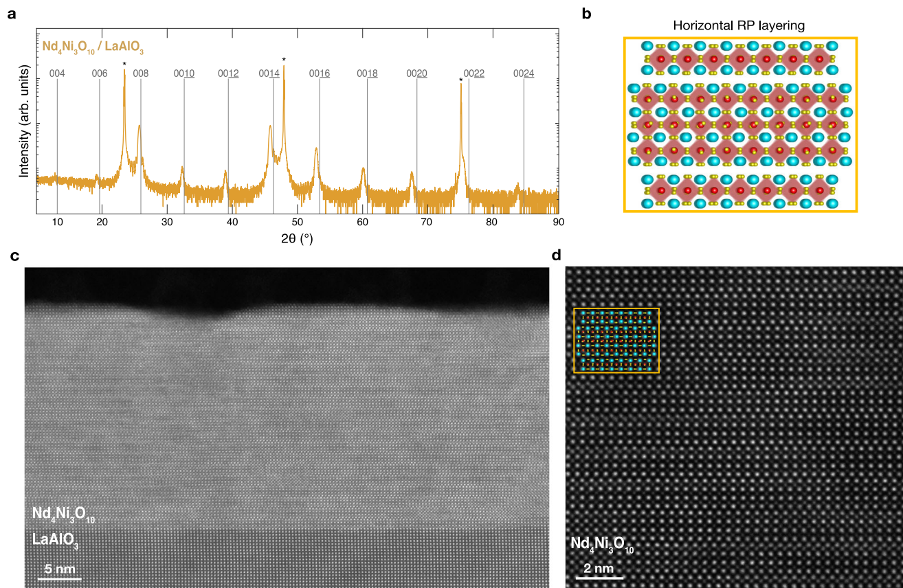
Fig. 4 | Structural characterization of \text{Nd}_4\text{Ni}_3\text{O}_{10}/\text{LaAlO}_3 (001) ( \epsilon = -0.9\% ). a XRD scan of a \text{Nd}_4\text{Ni}_3\text{O}_{10}/\text{LaAlO}_3 film. The asterisks denote substrate peaks and the vertical lines mark the 00l peak positions of bulk \text{Nd}_4\text{Ni}_3\text{O}_{10} 95 . b Schematic crystal structure of well-ordered, horizontal Ruddlesden–Popper layers. c MAADF-
