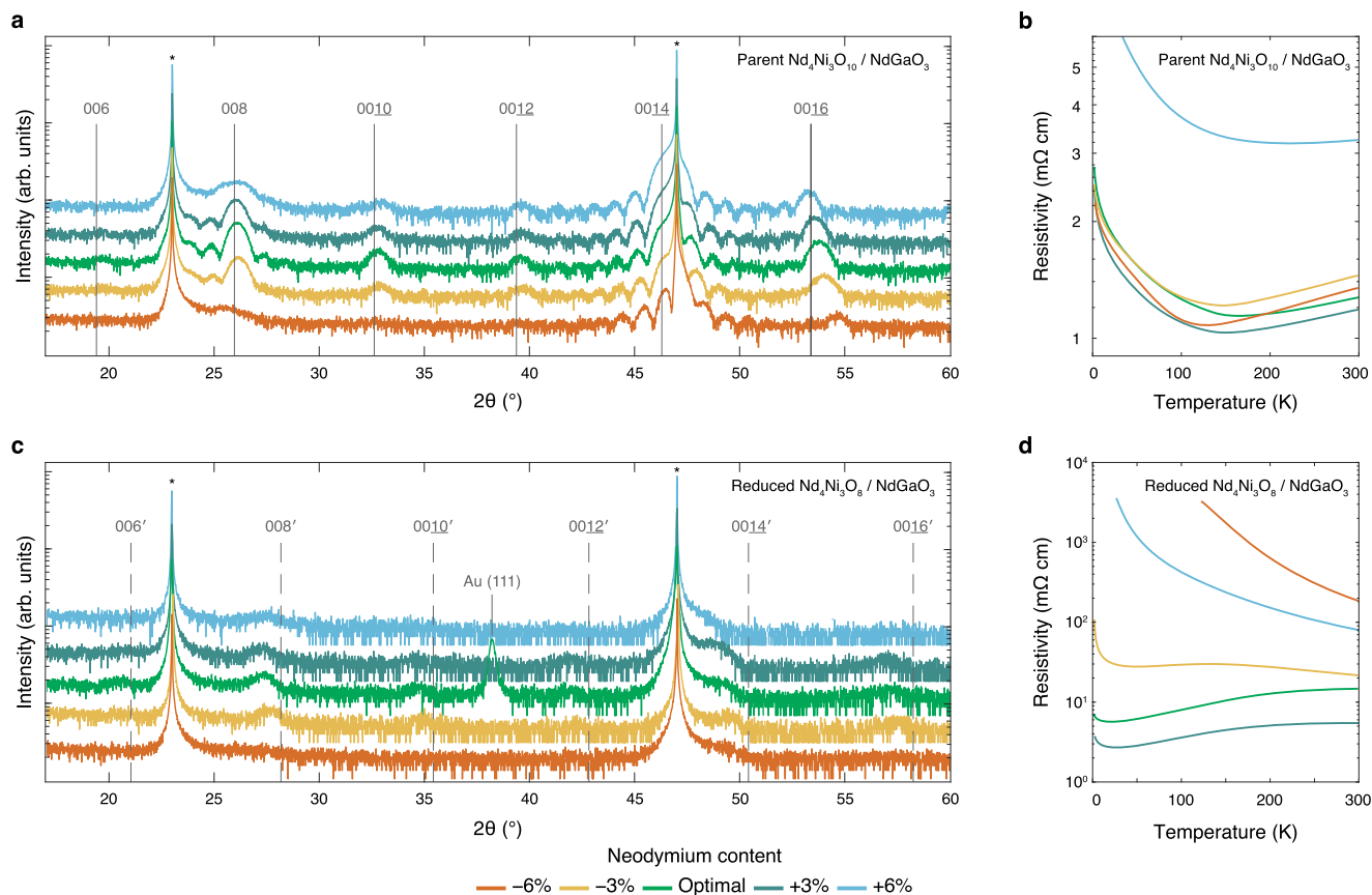
Fig. 10 | Structural and electrical transport characterization of \text{Nd}_4\text{Ni}_3\text{O}_{10} and \text{Nd}_4\text{Ni}_3\text{O}_8 films with varying neodymium content. a XRD and (b) resistivity measurements of the parent \text{Nd}_4\text{Ni}_3\text{O}_{10} films on \text{NdGaO}_3 . c XRD and (d) resistivity measurements of the reduced \text{Nd}_4\text{Ni}_3\text{O}_8 films in (a) . All films are \sim 11.0 nm and reduced for 3 hours at 290^\circ\text{C} . The vertical solid and dashed lines denote 00l peak
