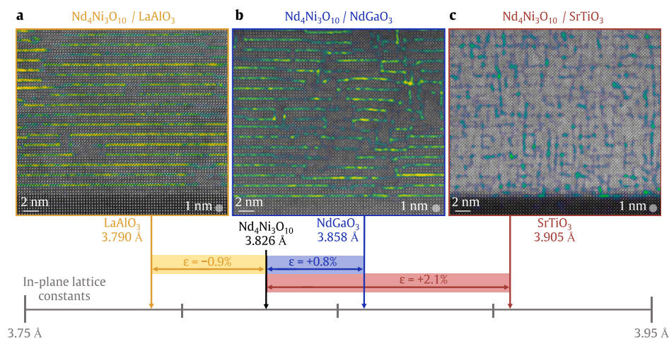
Fig. 5 | Strain-dependent structural characterization of \text{Nd}_4\text{Ni}_3\text{O}_{10} films. Lattice fringe strain maps highlighting the characteristic formation of horizontal and vertical rock salt layers in (a) \text{Nd}_4\text{Ni}_3\text{O}_{10}/\text{LaAlO}_3 (001), (b) \text{Nd}_4\text{Ni}_3\text{O}_{10}/\text{NdGaO}_3 (110), and (c) \text{Nd}_4\text{Ni}_3\text{O}_{10}/\text{SrTiO}_3 (001) films. The number line depicts the in-plane lattice constant of \text{Nd}_4\text{Ni}_3\text{O}_{10} in black and the corresponding strain states on \text{LaAlO}_3 in
