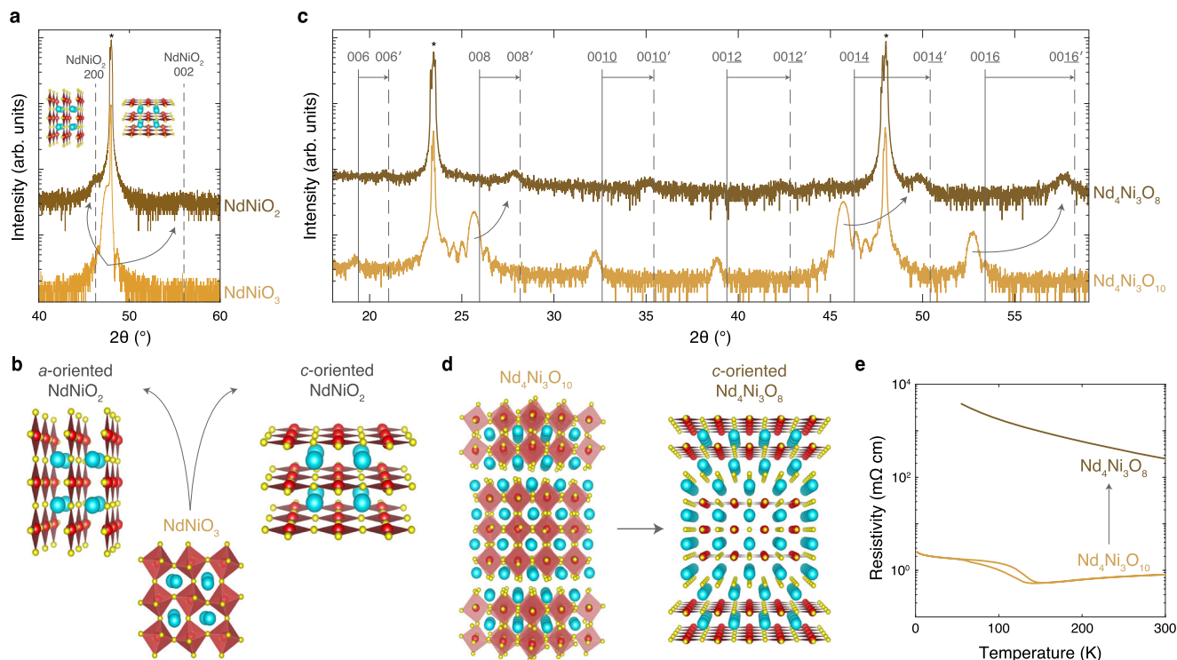
Fig. 6 | Structural and electrical transport characterization of NdNiO 3 and Nd 4 Ni 3 O 10 reductions on LaAlO 3 (001). a XRD scans of a 15.5 nm NdNiO 3 film as-synthesized (bottom) and reduced for 3 hours at 290 °C (top). The vertical dashed lines denote the 200 and 002 peak positions of bulk NdNiO 2 31 . b Schematic crystal structures illustrating the formation of a- and c-axis oriented NdNiO 2 upon reduction of NdNiO 3 . c XRD scans of a 20.0 nm Nd 4 Ni 3 O 10 film as-synthesized
