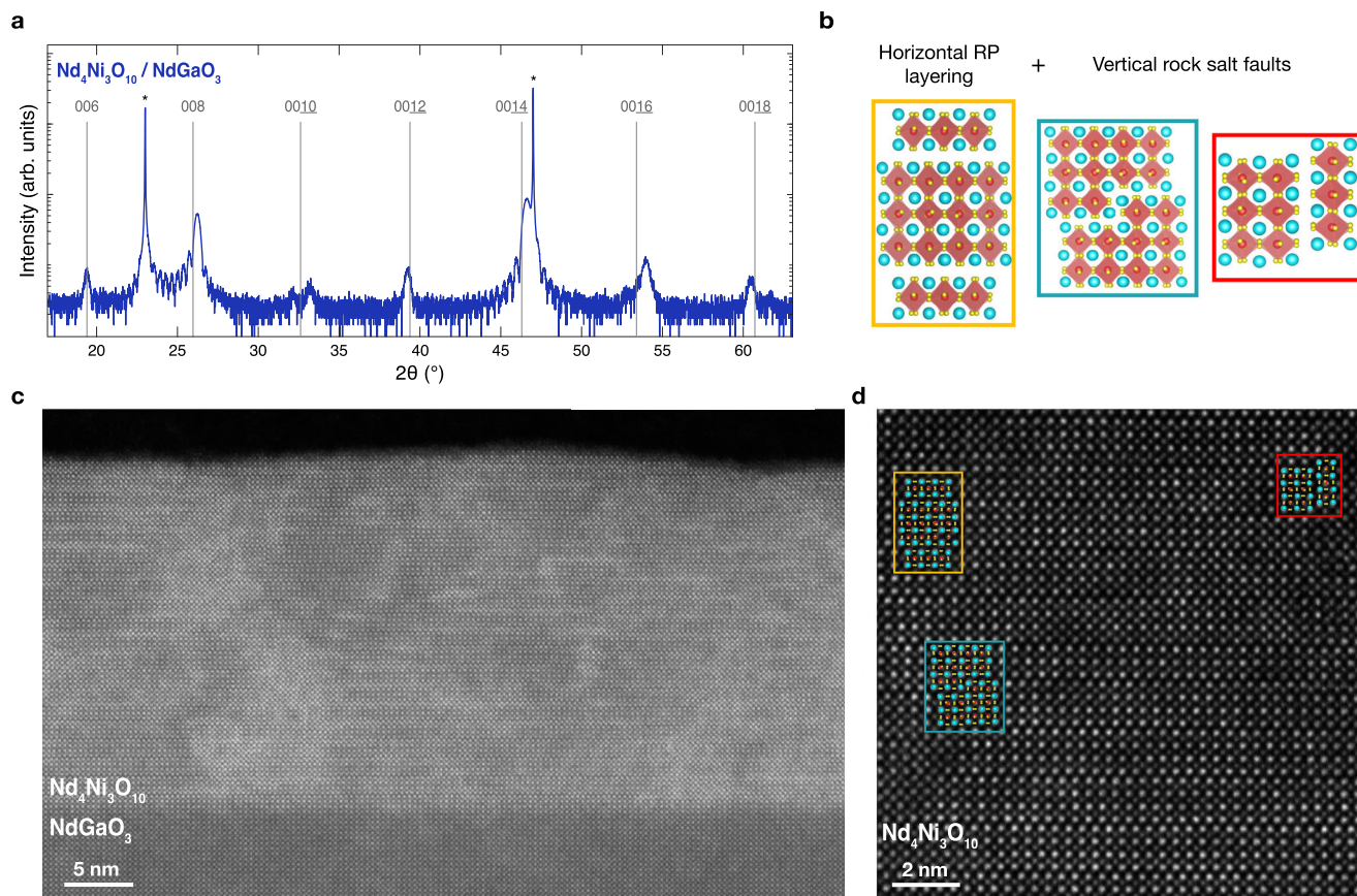
Fig. 3 | Structural characterization of \text{Nd}_4\text{Ni}_3\text{O}_{10}/\text{NdGaO}_3 (110) ( \epsilon = +0.8\% ).
