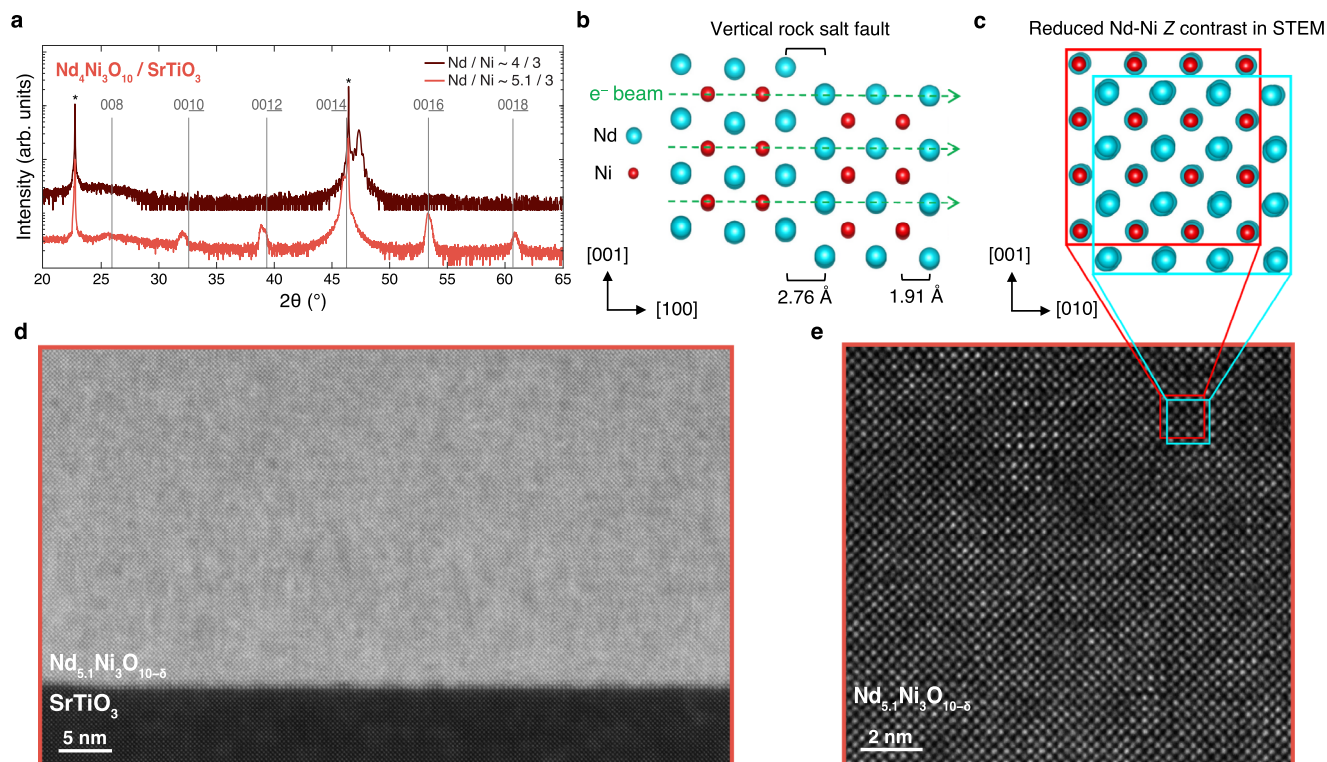
Fig. 2 | Structural characterization of \text{Nd}_4\text{Ni}_3\text{O}_{10}/\text{SrTiO}_3 (001) ( \epsilon = + 2.1\% ). a XRD scans of \text{Nd}_4\text{Ni}_3\text{O}_{10}/\text{SrTiO}_3 with Nd/Ni - 4/3 (nominally stoichiometric) and Nd/Ni - 5.1/3 (27.5% neodymium-rich). These compositions are measured by Rutherford backscattering spectroscopy (RBS). The asterisks denote substrate peaks and the vertical lines mark the 00 l peak positions of bulk \text{Nd}_4\text{Ni}_3\text{O}_{10} 95 . b Schematic crystal structure depicting a vertical rock salt fault. c 90° rotation of the crystal structure in (b) illustrating the origin of the atomic contrast loss in STEM. The green
