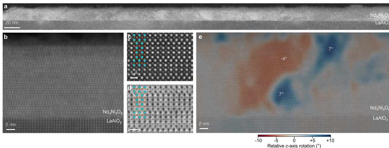
Fig. 7 | Structural characterization of a reduced \text{Nd}_4\text{Ni}_3\text{O}_8/\text{LaAlO}_3 film. a Large field-of-view MAADF-STEM image. b Atomic-resolution HAADF-STEM image of a region exhibiting high-quality layered square-planar structure. c HAADF and (d) ABF-STEM images of a small field of view with an overlaid atomic model of the square-planar structure. The full field-of-view is provided in Supplementary
