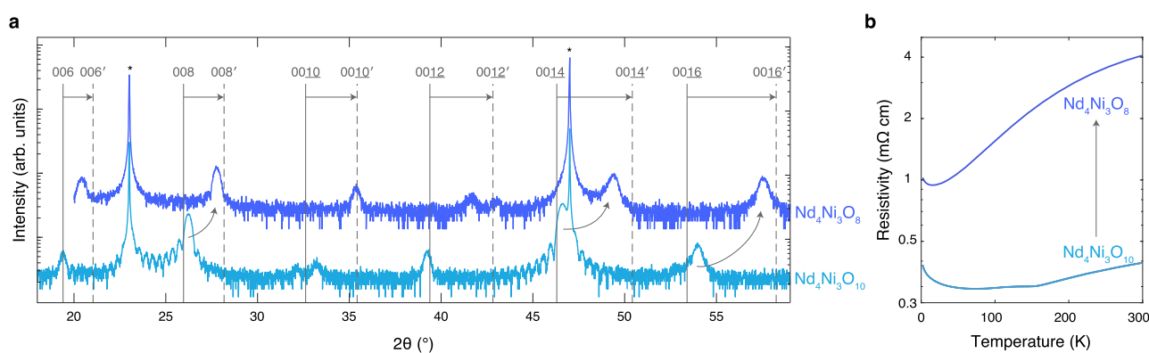
Fig. 8 | Structural and electrical transport characterization of \text{Nd}_4\text{Ni}_3\text{O}_{10} and \text{Nd}_4\text{Ni}_3\text{O}_8 on \text{NdGaO}_3 (110). a XRD scans of an as-synthesized \text{Nd}_4\text{Ni}_3\text{O}_{10} and reduced \text{Nd}_4\text{Ni}_3\text{O}_8 film on \text{NdGaO}_3 . The film is 25.5 nm and reduced for 3 hours at 300 °C. The vertical solid and dashed lines denote the 00 l peak positions of bulk
