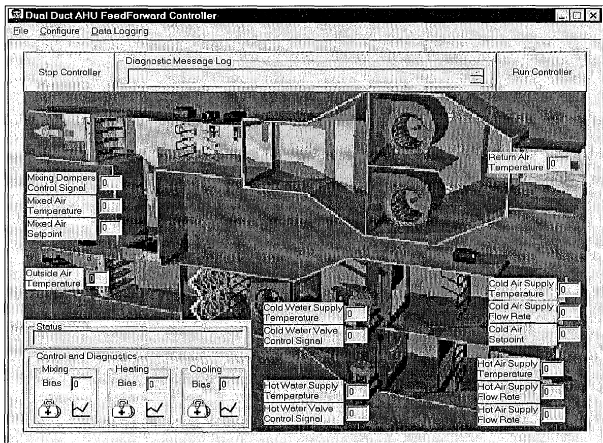
Figure 6. User Interface Showing the Dual-Duct Test Unit
