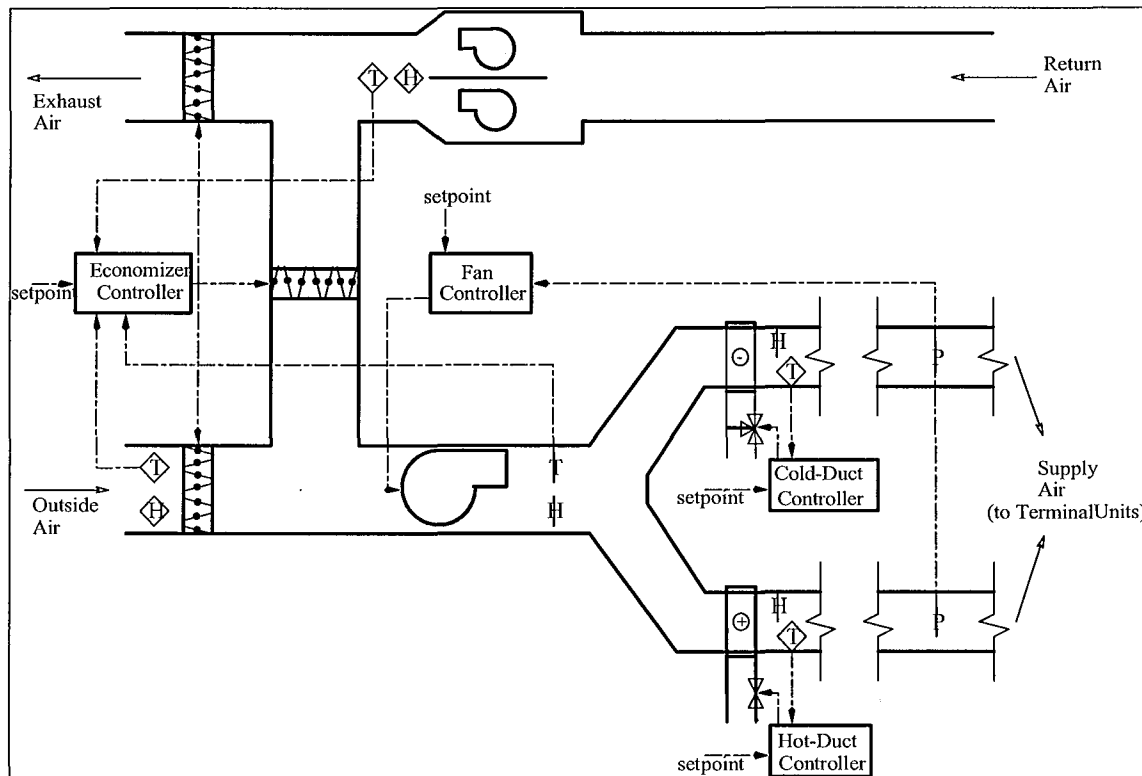
Figure 3. Schematic of the Dual-Duct Air-Handling Unit
