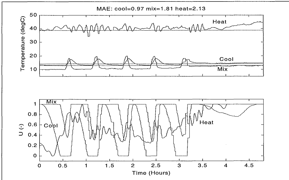
Figure 8. Control Performance
