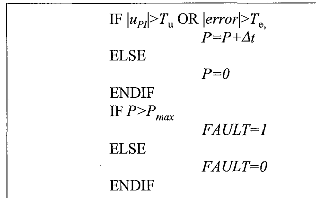
Figure 2. Fault Detection Logic
