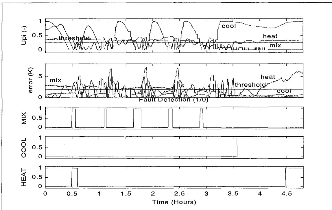
Figure 9. Fault Indicator Variables
