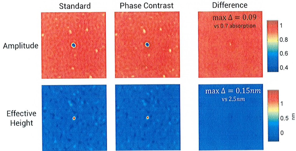
Figure 2. The amplitude and phase extracted from the standard zone plate measurements and the phase contrast zone plate measurements are nearly the same. The minimum amplitude was 0.3 while the maximum difference in the two amplitudes was only 0.09 . The maximum phase (in effective height) was 2.5\ \text{nm} and the maximum difference only 0.15\ \text{nm} . This suggests that the algorithm recovered the true phase and amplitude of the defect, since the datasets going into the algorithm were qualitatively different yet produced nearly the same result.
