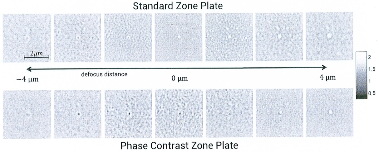
Figure 1. Aerial images of the same through-focus defect taken using a standard zone plate and a phase contrast zone plate produce very different images. Phase contrast causes the phase roughness to produce strong contrast at focus and changes the behavior of the defect through focus, which is described by the WOTF.
