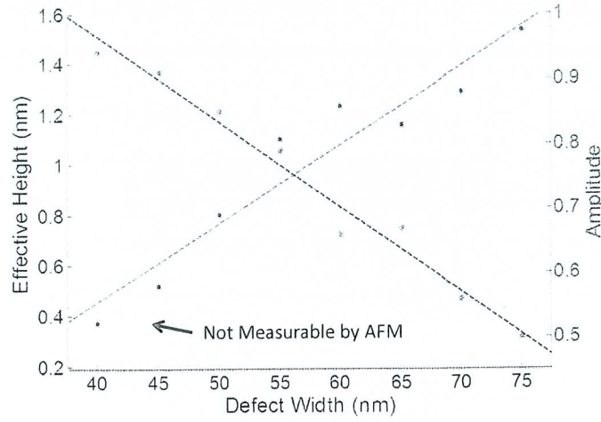
Figure 4. The maximum amplitude and phase (represented as height = phase \cdot \lambda / 4\pi ) of programmed defects relative to the surrounding area is plotted vs. the width of the defect on the substrate. Larger defects showed considerable absorption in addition to phase. Defects smaller than the AFM resolution were visible under imaging.
