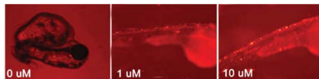
Fig. (6). CLR01 ameliorates \alpha -syn neurotoxicity in zebrafish (ZF). ZF embryos were treated with CLR01 at 8 hpf and were monitored for abnormal appearance and survival. Bright-field and fluorescent overlay images were taken at 72 hpf. For quantitative analysis, see [93].
