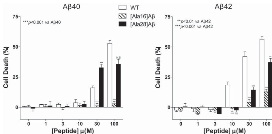
Fig. (1). Toxicity of A \beta 40, A \beta 42, and their A-substituted analogues. A \beta 40, A \beta 42, and their respective K→A analogues were incubated with differentiated PC-12 cells for 48 h and cell death was measured using the lactate dehydrogenase (LDH) release assay. The results are an average of four to six experiments and are presented as mean \pm SEM. Statistical significance was calculated by one-way ANOVA.
