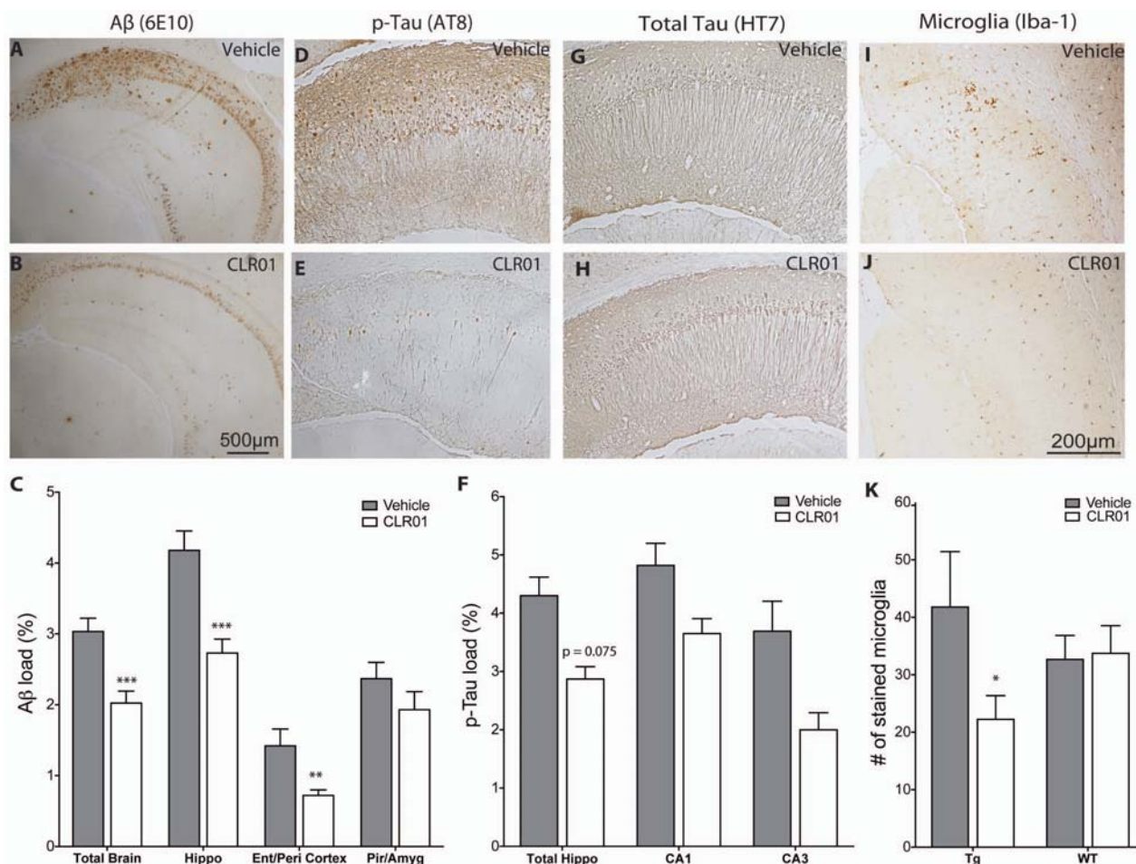
Fig. (8). CLR01 decreases amyloid β-protein and hyperphosphorylated-tau deposition and ameliorates microgliosis in transgenic mouse brain. Triple-transgenic mice were treated with 40 μg/kg/day CLR01 or vehicle. A, D, G, I ) Vehicle-treated transgenic mouse hippocampus. B, E, H, J ) CLR01-treated transgenic mouse hippocampus. A, B ) transgenic mouse brain stained with monoclonal antibody (mAb) 6E10 showing amyloid plaque deposition. C ) % Aβ burden was quantified by calculating the total 6E10-stained area divided by the total area measured (Hippo – hippocampus, Ent – entorhinal, Peri – perirhinal, Pir – piriform cortices, Amyg – amygdala). D, E ) transgenic mouse brain showing mAb AT8-positive neurofibrillary tangles in the CA1 region. F ) % Aggregated hyperphosphorylated tau load was quantified by calculating the total AT8-stained area divided by the total area. G, H ) transgenic mouse brain stained with mAb HT7 for total tau. I, J ) transgenic mouse brain showing Iba1-positive microglia in the subiculum and CA1 region. K ) Number of stained microglia in a 1.14 mm 2 area of hippocampus per treatment condition. The scale bar in panel B applies to both panels A and B . The scale bar in panel J applies to panels D–J . * p < 0.05, ** p < 0.01, *** p < 0.001 compared to vehicle-treated mice using linear mixed effects models for panels C and F and Student’s unpaired t -test for panel K .
