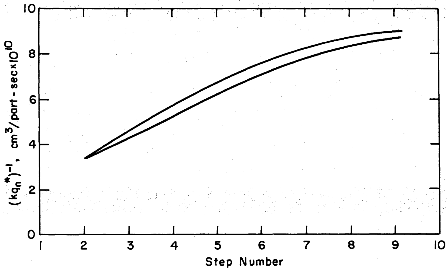
Fig. 27. Graph of (kq_n^*)^{-1} comparing the flat and semiflat spectral distributions. The curve for the flat distribution is shifted one step to lower energy.
