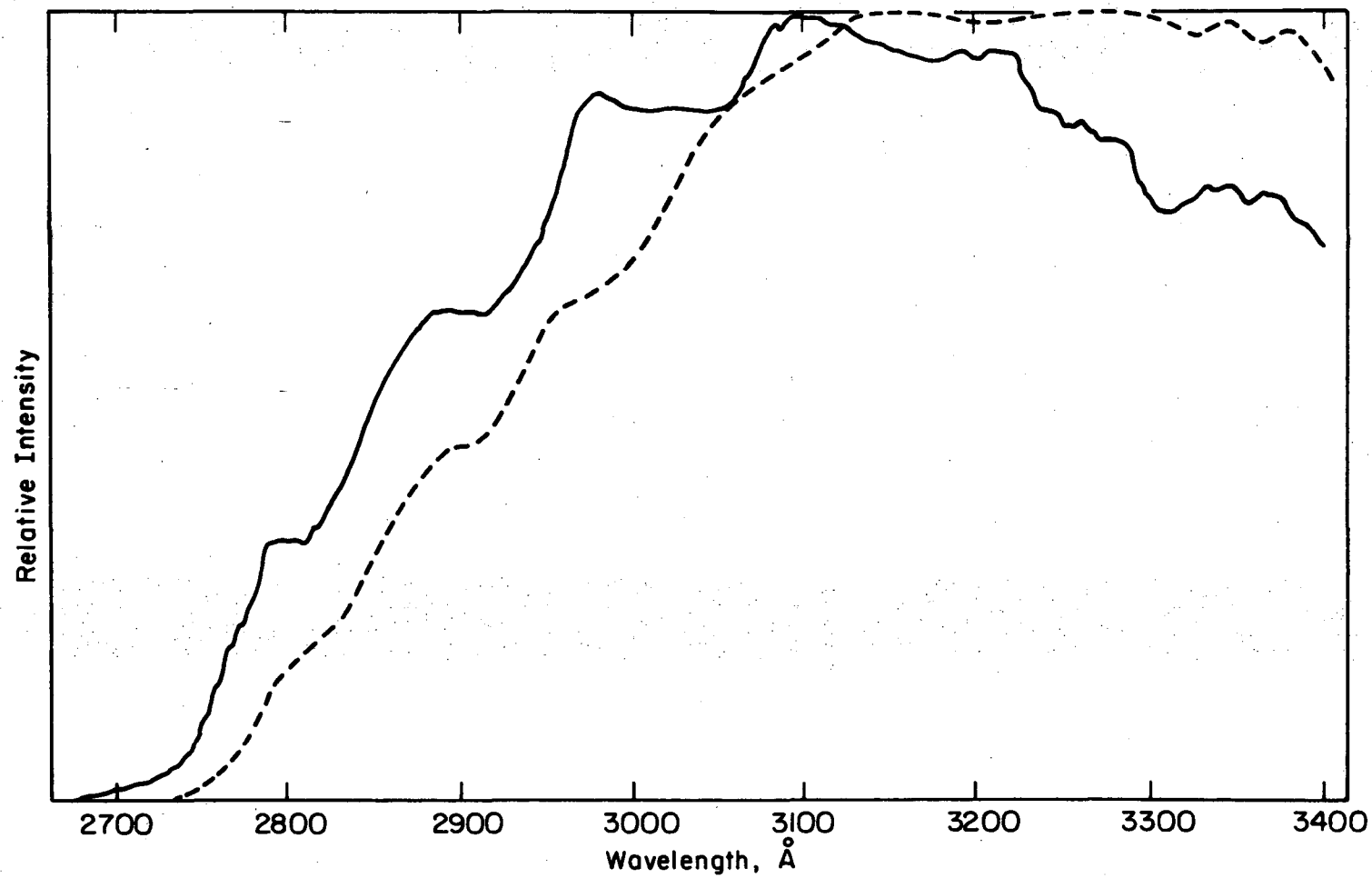
Fig. 13. Emission spectrum at \lambda_{\text{ex}} = 2760 \text{ Å} . Solid line, low pressure; dotted line, high pressure. High pressure spectrum relative intensity is 7.8 times as great as low pressure spectrum.
