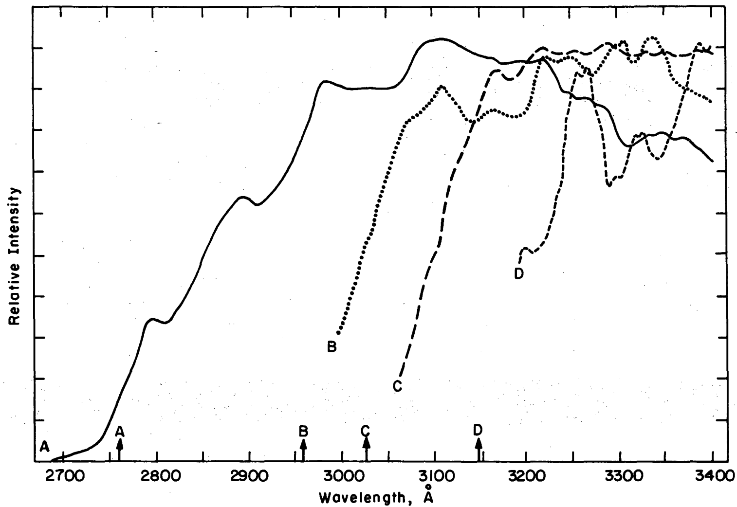
Fig. 17a. Graphs of low pressure spectra normalized to the same relative intensity. A, \lambda_{\text{ex}} = 2760 \text{ Å} , solid line; B, \lambda_{\text{ex}} = 2960 \text{ Å} , dotted line; C, \lambda_{\text{ex}} = 3023 \text{ Å} , long dashes; D, \lambda_{\text{ex}} = 3147 \text{ Å} , short dashes.
