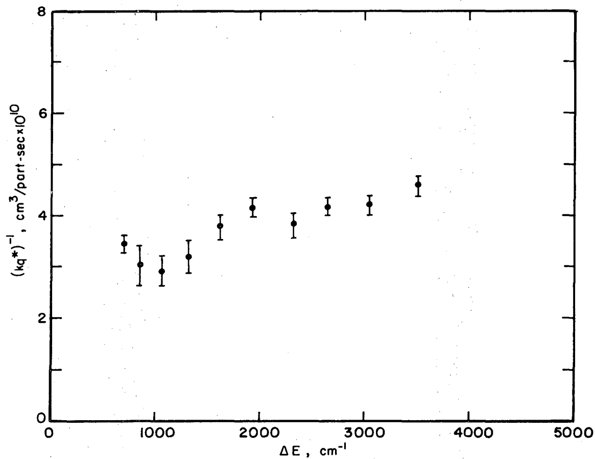
Fig. 31. Graph of experimental values of (k_q^*)^{-1} for excitation at 3023 Å. Error bars represent two standard deviations of the slopes from which each value of (k_q^*)^{-1} was calculated.
