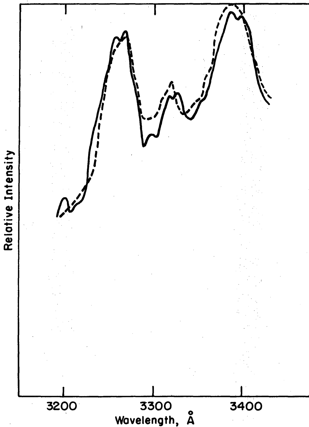
Fig. 16. Emission spectrum at \lambda_{\text{ex}} = 3147 \text{ Å} . Solid line, low pressure; dotted line, high pressure. High pressure spectrum relative intensity is 1.2 times as great as low pressure spectrum.
