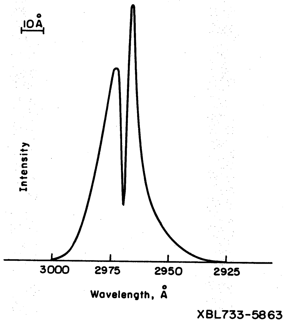
Fig. 7. Excitation profile at "2962" Å.
