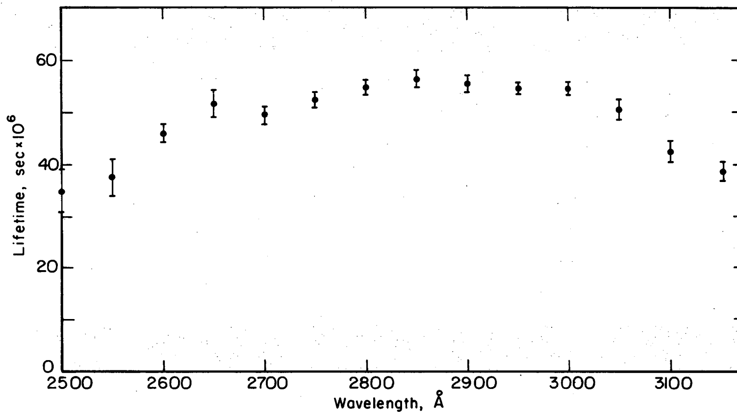
Fig. 18. Fluorescence lifetime of SO 2 at pressures less than 0.2 mTorr. Error bars represent two standard deviations determined from several experiments.
