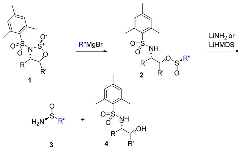
Scheme 1. Senanayake's Sulfinyl Transfer Approach
