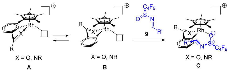
Figure 1. Stereochemical model consistent with sense of induction
