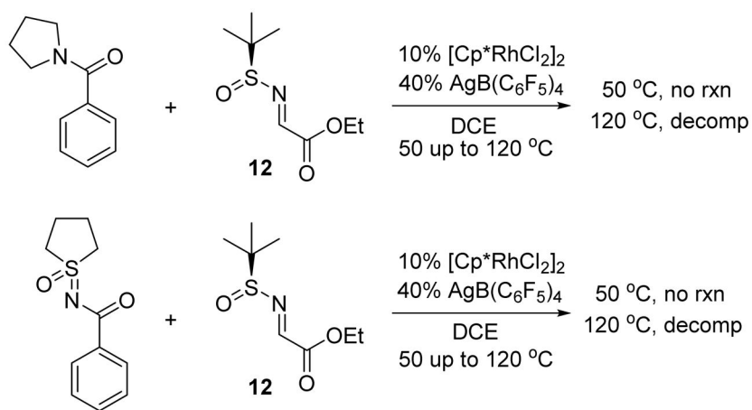
Scheme 3. Attempted C–H Additions to N - tert -Butanesulfinyl Imino Ester 12
