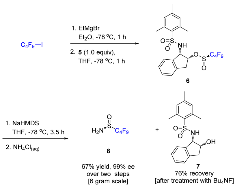
Scheme 2. A Practical Asymmetric Synthesis of Perfluorobutanesulfinamide.
