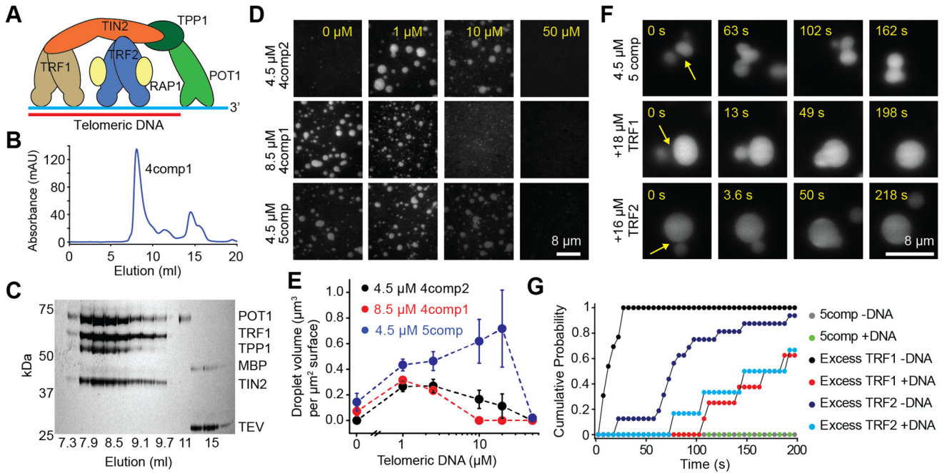
Figure 4. The shelterin complex phase separates in vitro . A. A schematic of the human shelterin complex. TRF1 and TRF2 are homodimers that bind to dsTEL, and POT1/TPP1 binds to ssTEL. TIN2 interconnects TRF1, TRF2, and TPP1, and RAP1 binds to TRF2. B-C. UV absorbance (B) and denaturing gel (C) show that 4comp1 elutes as a single complex from a gel filtration column. D. 4comp2 and 5comp exhibit reentrant responses to increasing DNA concentration similar to TRF2 droplets, while 4comp1 is inhibited by increasing DNA concentration similar to TRF1 droplets. E. The total volume of shelterin droplets settled per micron squared area on the coverslip under variable 8ds3ss concentration (mean \pm SD, n = 20 with two technical replicates). F. In the presence of 2.5 \mu M 8ds3ss, 5comp droplets do not fuse on relevant time scales, whereas the addition of excess TRF1 or TRF2 reduces the fusion time. G. Cumulative probability of 5comp droplet fusion in the presence and absence of excess TRF1 or TRF2 after forming a contact at t = 0 s (n = 7, 4, 13, 16, 15 and 7 events from top to bottom). See also Figure S4 and Movie S4.
