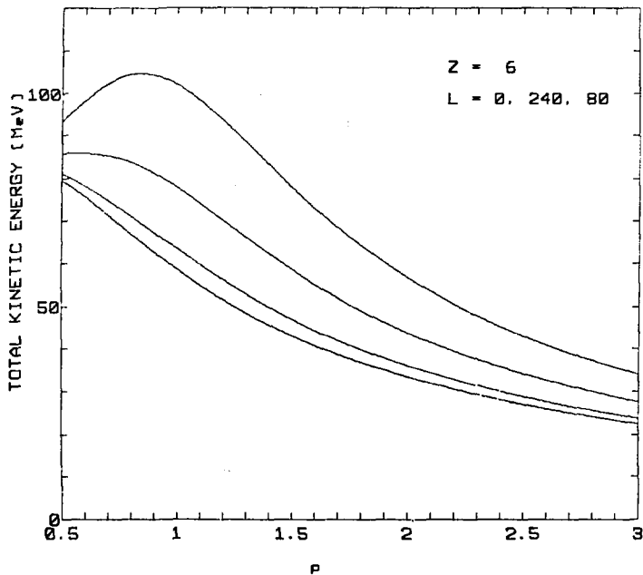
Fig. 16 Calculated total center of mass kinetic energy versus fragment deformation for atomic number 6, at four angular momenta: 0, 80, 160 and 240 \hbar . Angular momentum increases from lower to upper curves.
