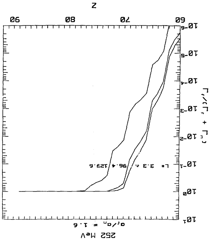
Fig. 33.9 Same as Fig. 33.3. LPR = 1.6 . 252 MeV projectile energy.
