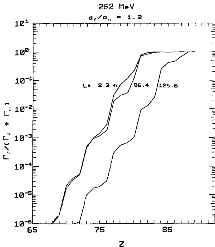
Fig. 33.7 Same as Fig. 33.3. LDPR = 1.2. 252 MeV projectile energy.
