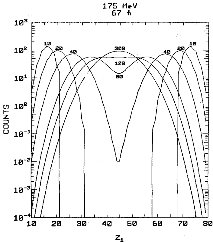
Fig. 31 Calculated distribution of elements at six different times, based on diffusion model. 175 MeV projectile energy.
