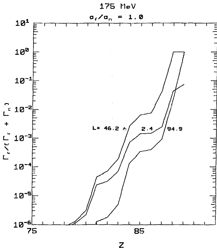
Fig. 33.3 Calculated multi-chance fission probability for heavy elements, at 3 incident angular momenta. LDPR = 1.0. 175 MeV projectile energy.
