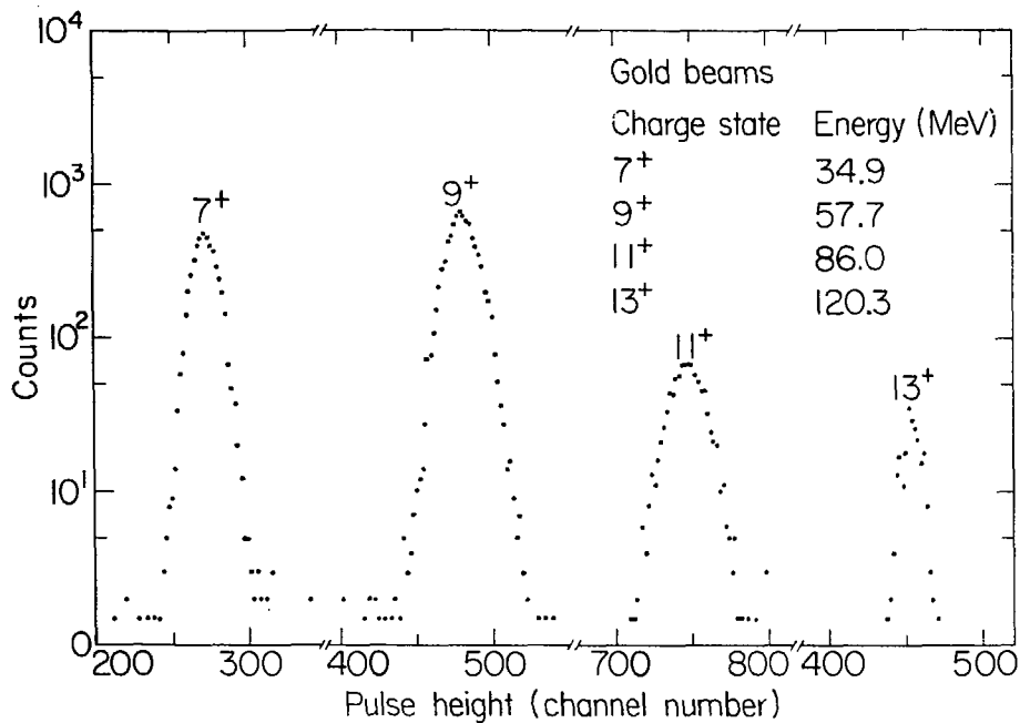
Fig. 43 Pulse height spectrum of counts vs. energy for \text{Au}^{7+} , \text{Au}^{9+} , \text{Au}^{11+} , and \text{Au}^{13+} beams. Note the near absence of background events.
