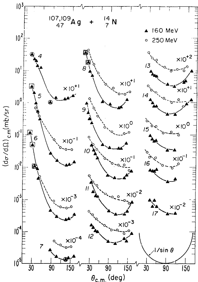
Fig. 34 Experimental center of mass angular distributions for the reaction N + Ag (Mo 75a).
