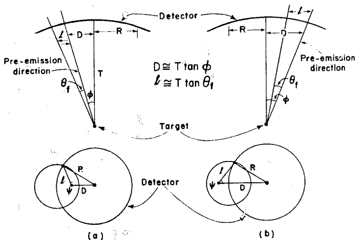
Fig. 42 Explanation of angles used in Eq. (22) for Appendix I.3.
