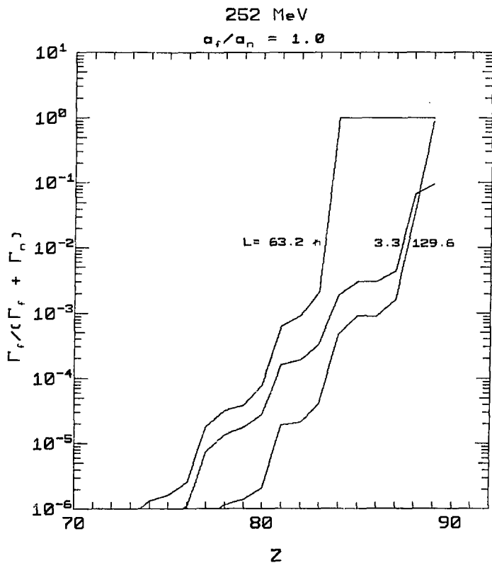
Fig. 33.6 Same as Fig. 33.3. LDPR = 1.0. 252 MeV projectile energy.
