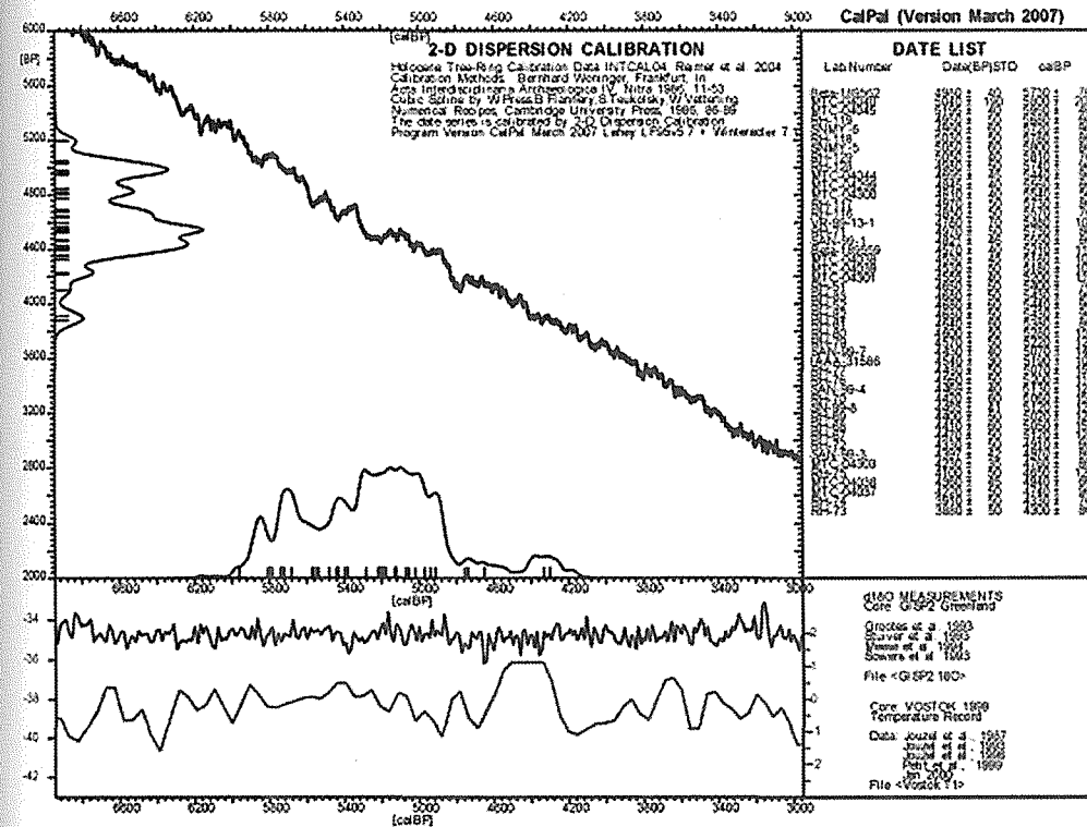
Figure 4.1. Distribution of radiocarbon determination for Sannai Maruyama and data for climate change. The top section shows radiocarbon data from Kobayashi (2004) and Tsuji (2006). The bottom section shows climate data. The top line in the section shows oxygen isotope data from the Greenland Ice Sheet Project 2 (GISP2). The bottom line is temperature data from the Vostok ice core.
