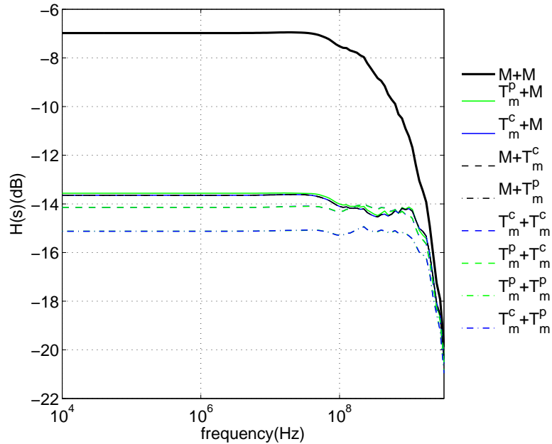
Figure IV.12: Transfer functions of solutions in Table IV.4
