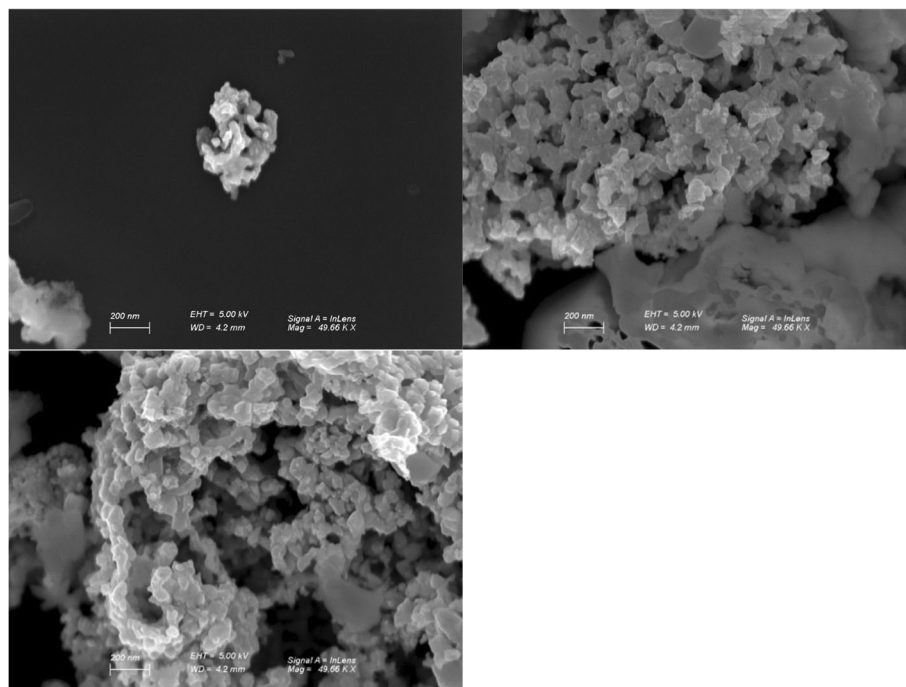
Fig. 1 SEM image of LSM physical characteristics. The single particle size was around 35 nm in diameter and the aggregation of LSM size varied from 200 nm to a few \mu\text{m}
