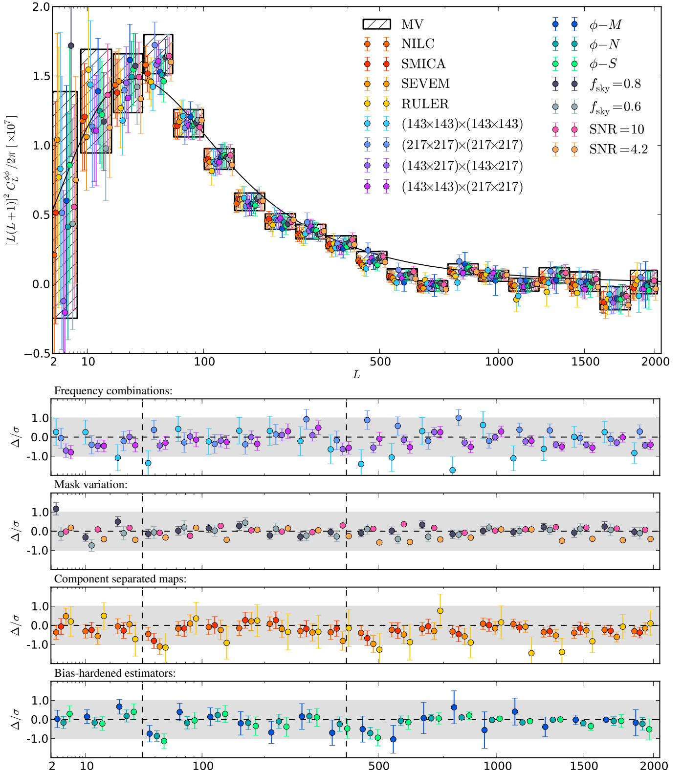
Fig. 18. Summary of internal consistency tests between our fiducial minimum-variance (MV) reconstruction and a set of alternatives designed to test sensitivity to potential issues. The top panel shows C_L^{\phi\phi} estimates, with measurement error bars. The bottom panels show the residual with respect to the MV reconstruction in units of the MV measurement uncertainty. The grey band marks the 1\sigma deviation uncertainty of the MV reconstruction. The error bar on each data point in the lower panels gives the standard deviation of the scatter between each result and the MV, determined from Monte-Carlo simulations that account for the correlated CMB, noise and foreground power between estimators. Comparison of the uncertainty on the scatter points and the grey band gives an indication of how constraining each test is. The various tests are described in more detail in subsections of Sect. 7.
