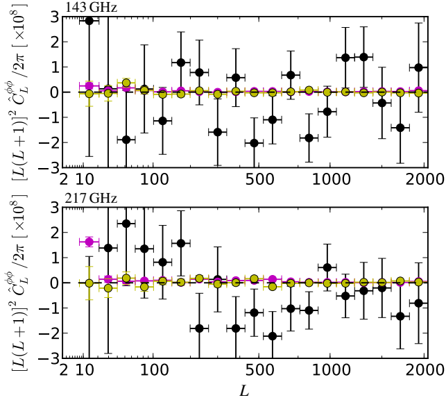
Fig. A.1. Survey consistency null tests at 143 GHz and 217 GHz. Solid black points show difference of \hat{C}_L^{\phi} estimated separately on the two six-month surveys of the nominal mission. Magenta points show the auto-spectrum of \hat{\phi} obtained from maps made by taking the half-difference of the two surveys (S1 - S2) \times (S1 - S2) . Yellow points show the cross-spectrum of \hat{\phi} obtained on half-difference and half-sum maps (S1 - S2) \times (S1 + S2) . The scatter on the tests that contain difference maps is very small because (as can be seen in Fig. 6) most of the lens reconstruction “noise” is due to primary CMB fluctuations, which is nulled in these tests.
