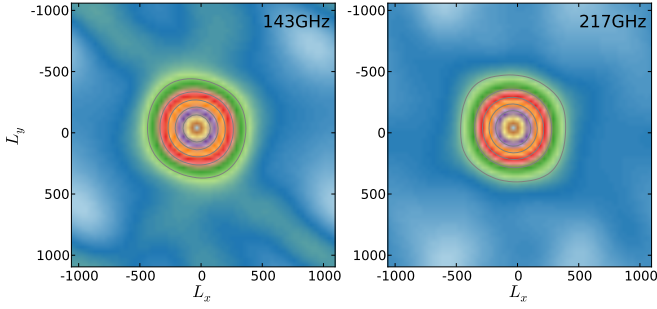
Fig. A.4. Bi-dimensional deflection power spectrum obtained by stacking the individual Fourier amplitude obtained on patches, after \Delta C_{L, \text{NSO}}^{\phi\phi} subtraction and smoothing for the 143 and 217 GHz channels.
