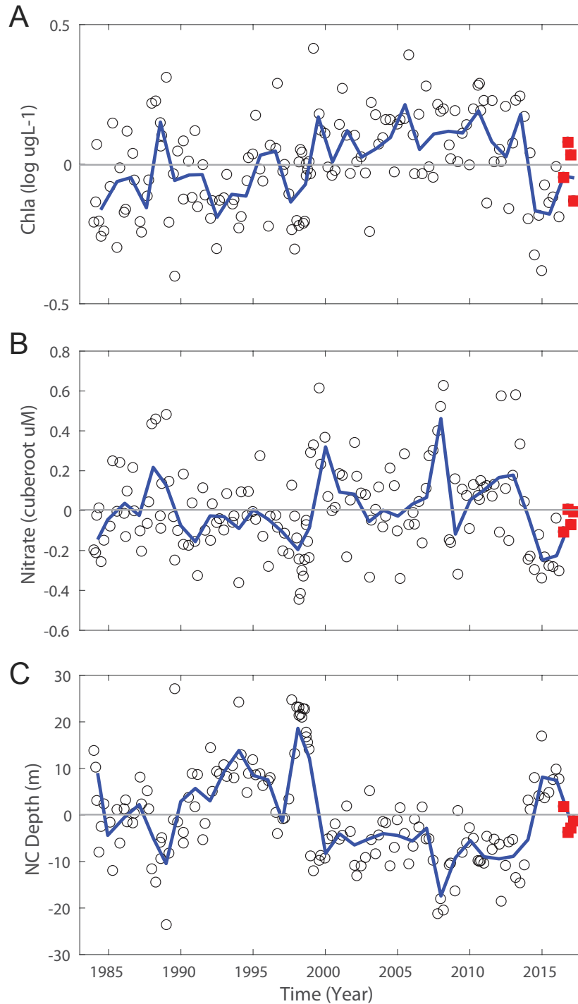
Figure 17. Cruise averages of properties for a depth of 10 m for the CalCOFI standard grid plotted as anomalies relative to the mean of the time series. A) The log 10 of chlorophyll a, B) the cube root of nitrate, and C) nitracline depth.
