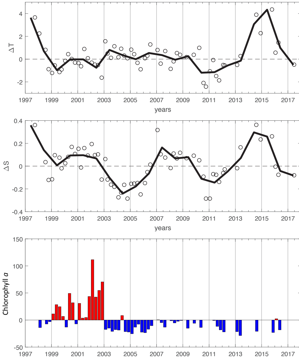
Figure 18. Interannual variability of the mixed layer temperature anomalies (°C) and salinity anomalies in the IMECOCAL region for the period 1997–2017 (white circles) and the mean of each year (thick line). Depth-integrated (0–100 m) chlorophyll a anomalies ( \text{mg m}^{-2} ) in the IMECOCAL region.
