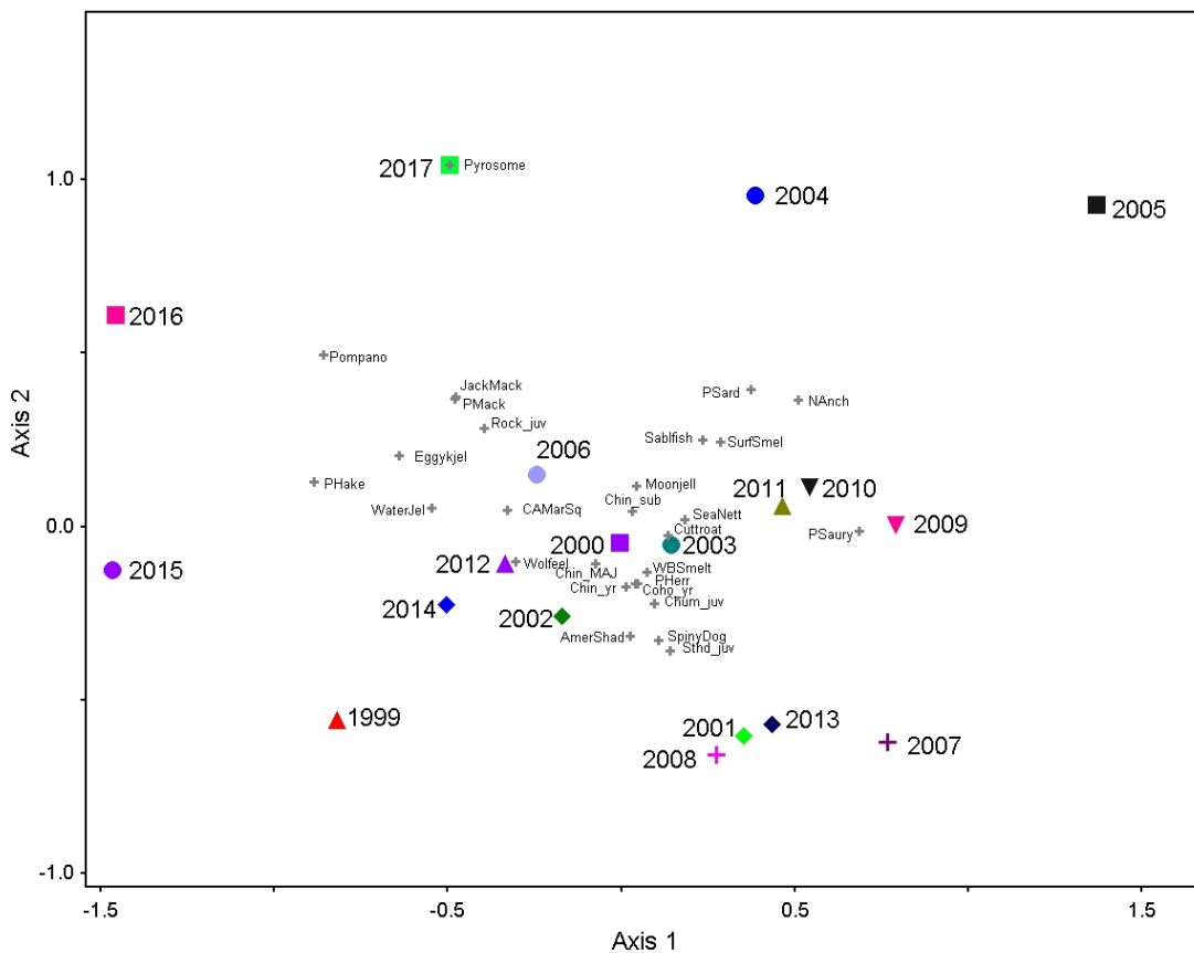
Figure 23. NMDS ordination of northern California Current pelagic assemblages. The NMS ordination explained 80.8% of the total variability in the first two dimensions. Pelagic fish and invertebrate catch data were collected by the NWFSC NOAA/Bonneville Power Administration surveys using surface trawls on standard stations along transects between northern Washington and Newport, OR, in June from 1999 to 2016. All tows were made during the day at predetermined locations along transects extending off the coast to the shelf break (Brodeur et al. 2005).
