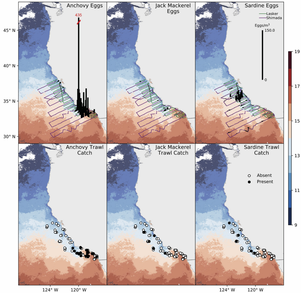
Figure 30. Density of eggs of northern anchovy, jack mackerel, and sardine collected with the continuous underway fish egg sampler (CUFES) during the spring 2017 CalCOFI and coastal pelagic fish cruises overlaid on satellite sea surface temperatures (°C). Lower panels represent trawls in which anchovy, jack mackerel, and sardine were absent or present.
