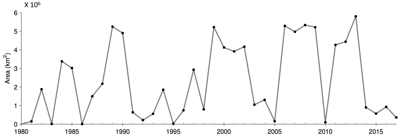
Figure 6. The area of high atmospheric pressure of the North Pacific High averaged over January and February each year (Schroeder et al. 2013). The area is the areal extent of the 1020 hPa isobar located in the eastern North Pacific.
