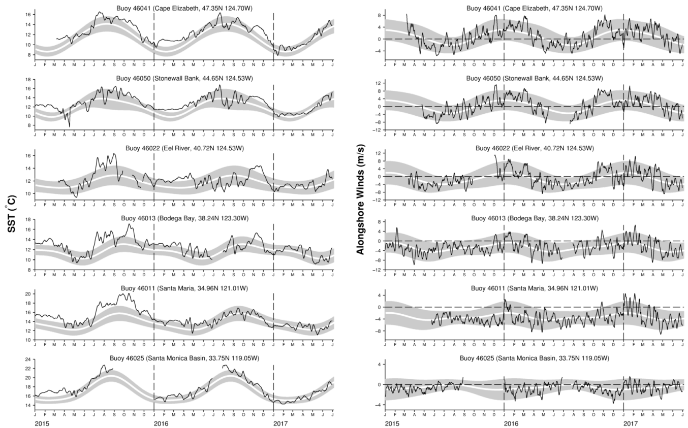
Figure 7. Time series of daily sea surface temperatures (left) and alongshore winds (right) from various National Data Buoy Center (NDBC) coastal buoys along the CCS for January 2015 to June 2017. The wide white line is the biharmonic annual climatological cycle at each buoy. Shaded areas are the standard errors for each Julian day. Series have been smoothed with a 7-day running mean. Data provided by NOAA NDBC. Additional buoy information can be found at http://www.ndbc.noaa.gov/ .
