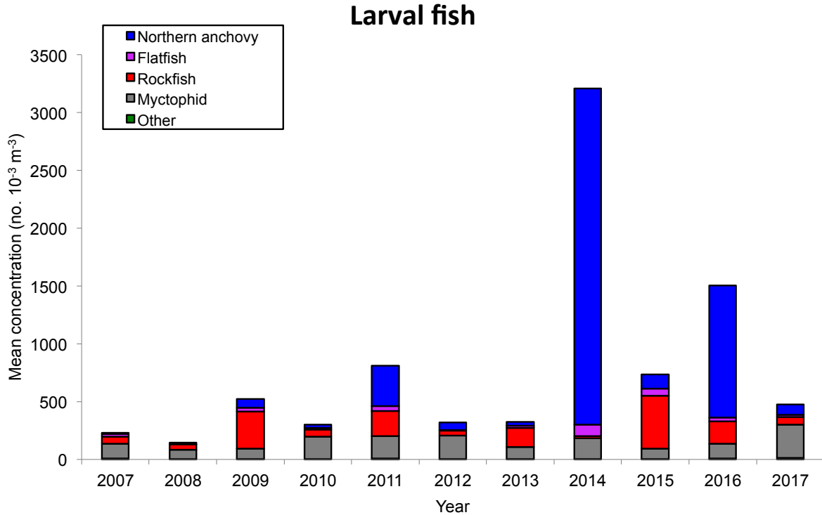
Figure 20. Mean concentrations (no. 10 -3 m -3 ) of the dominant larval fish taxa collected during June–July in 2007–17 along the Newport Hydrographic (NH; 44.65°N, 124.35–125.12°W) and Columbia River (CR; 46.16°N, 124.22–125.18°W) lines off the coast of Oregon.
