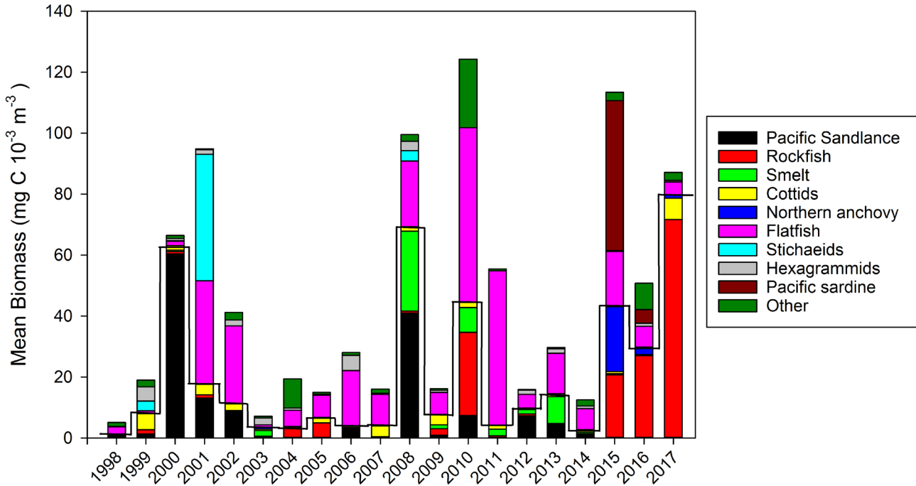
Figure 25. Annual mean biomass ( \text{mg C } 10^{-3} \text{ m}^{-3} ) of the five important salmon prey taxa (below solid line) and five other dominant larval fish taxa (above solid line) collected during winter (January–March) in 1998–2017 along the Newport Hydrographic line off the coast of Oregon (44.65°N, 124.18–124.65°W). Figure expanded from one presented in Daly et al. (2013).
