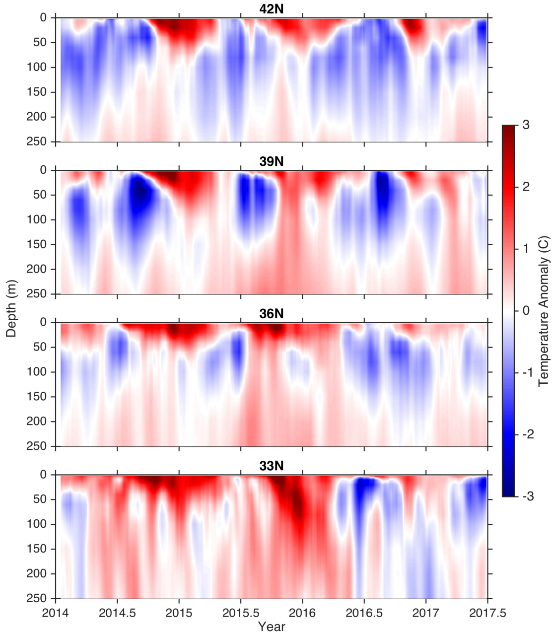
Figure 8. Temperature anomalies relative to the 1999–2011 climatology, derived from a data assimilative ocean reanalysis of the California Current System ( http://oceanmodeling.ucsc.edu/ccsrt/ ), are shown at four latitudes off the US West Coast. Temperatures are averaged from the coast to 100 km offshore and smoothed with a 30-day running mean.
