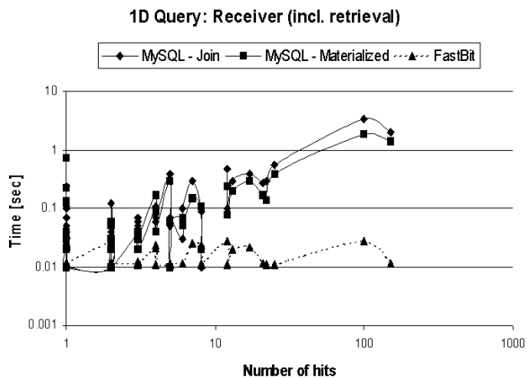
Figure 2. Performance of query: “Retrieve the senders of all emails that were received by person P ”.
