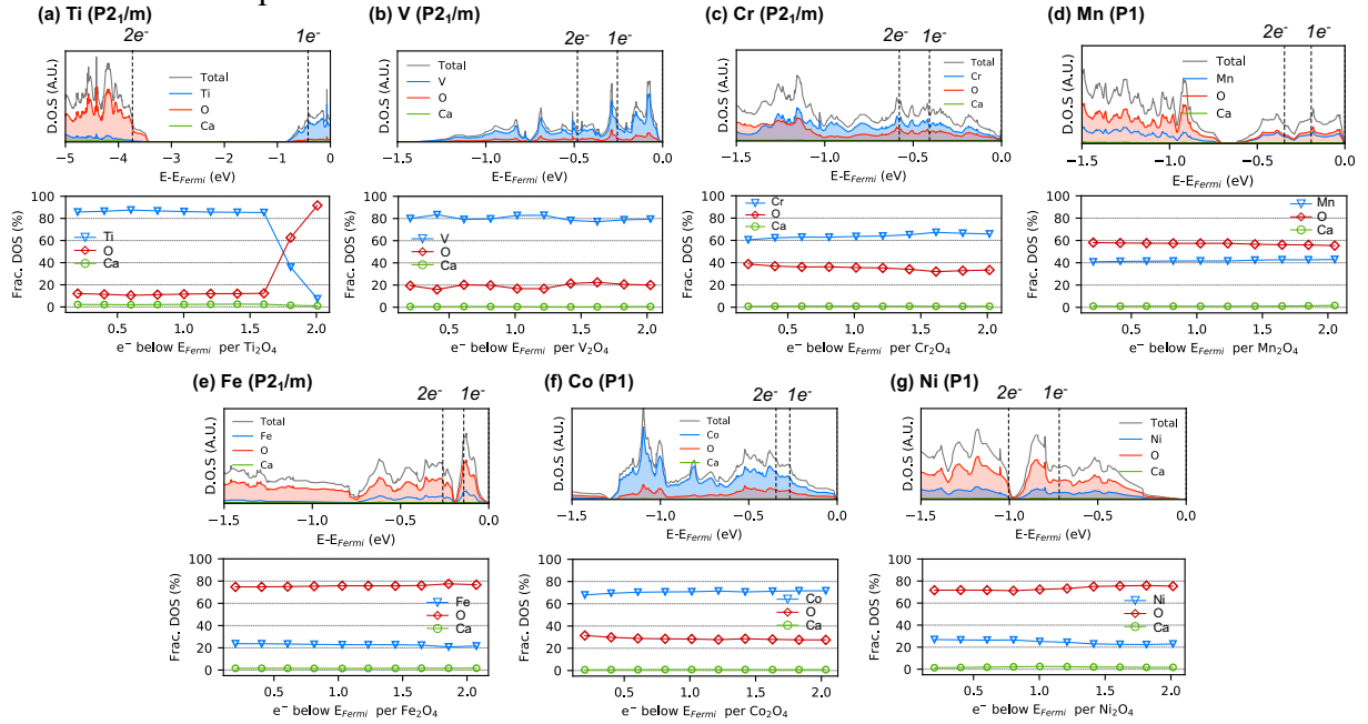
Figure 4. Atom-projected density of state (PDOS) and the contribution of each species to total density of state (DOS) of the various TM((a)Ti, (b)V, (c)Cr, (d)Mn, (e)Fe, (f)Co, (g)Ni) substituted \text{CaTM}_2\text{O}_4 . In the PDOS plot, the grey, blue, red, and green represent the total DOS, TM PDOS, O PDOS, and Ca PDOS, respectively. The DOS is in an arbitrary unit (A. U.). The dashed lines indicate the energy levels where the total number of electrons from Fermi energy are one and two, respectively. The contribution of PDOS to the total DOS was sampled approximately every 0.2e^- and the fraction of each species in total DOS is plotted below the PDOS plot.
