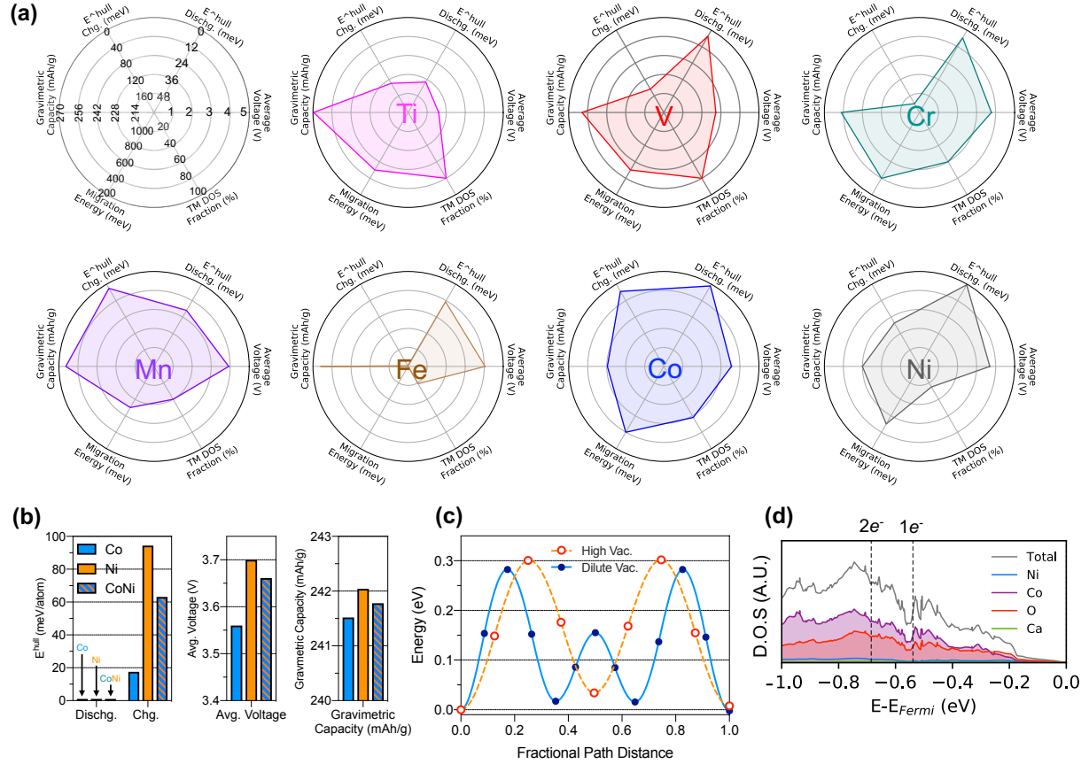
Figure 5. (a) Radar plots of the calculated battery-related properties of layered-CaTM 2 O 4 . (b) Energy above hull, average intercalation voltage, and gravimetric capacity of layered-CaCoNiO 4 , CaCo 2 O 4 , and CaNi 2 O 4 compounds. (c) The minimum energy pathways for Ca migration in the layered-CaCoNiO 4 at dilute vacancy limit. (d) Partial density of states plot of layered-CaCoNiO 4 compound.
