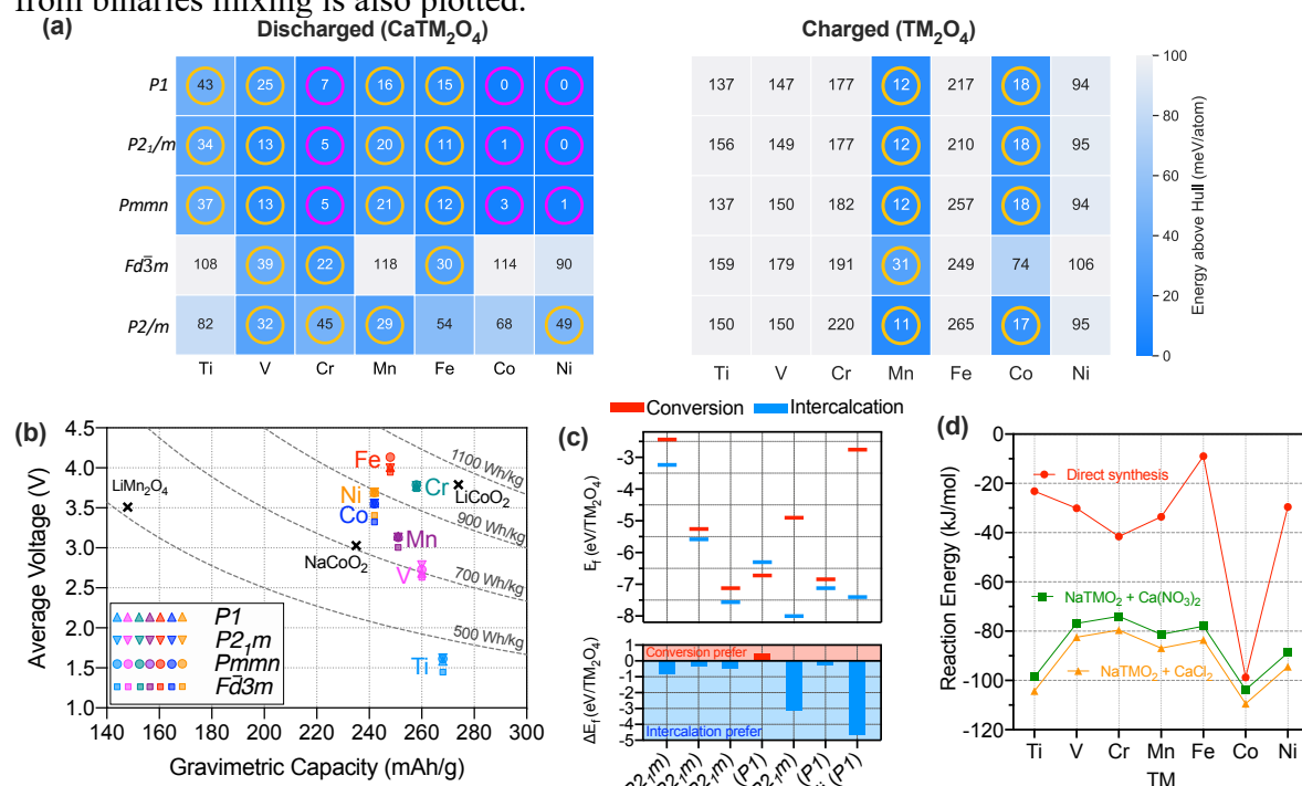
Figure 2. (a) Energy above the convex hull ( E^{\text{hull}} ) of various layered type \text{CaTM}_2\text{O}_4 and \text{TM}_2\text{O}_4 . The color and the annotation of each square in the heatmap represents E^{\text{hull}} of layered- \text{CaTM}_2\text{O}_4 or \text{TM}_2\text{O}_4 , where the type of layer and the TM specie correspond to the ordinate and the abscissa, respectively. The magenta and yellow circles on the heatmap indicate the compound with E^{\text{hull}} within 10meV/atom and 50meV/atom, respectively. (b) The computed average voltage versus gravimetric capacity for intercalation of Ca in various layered type of \text{TMO}_2 . The color and the marker shape of data point convey the information of redox specie and the structure type, respectively. (c) The preference between intercalation and conversion reaction upon Ca insertion into layered- \text{TMO}_2 . The horizontal blue and red lines represent the free energy of intercalation and conversion reaction, respectively. The free energy difference between two reactions is shown at the bottom, where positive value (blue area) and the negative value (red area) signify the preferential intercalation and conversion reaction, respectively. (d) Formation energy for producing \text{CaTM}_2\text{O}_4 by mean of ionic exchange between \text{NaTMO}_2 and \text{CaCl}_2 or \text{Ca}(\text{NO}_3)_2 . The formation energies of \text{CaTM}_2\text{O}_4 from binaries mixing is also plotted.
