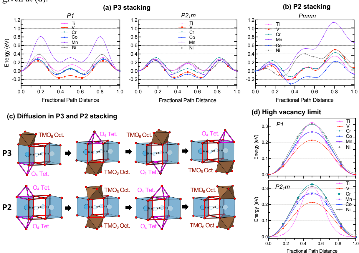
Figure 3. The minimum energy pathways for migration of Ca ion at the dilute vacancy limit in the various TM substituted layered- \text{CaTM}_2\text{O}_4 with (a) P3 stacking (space group: P1 , P2_1/m ) and (b) P2 stacking (space group: Pmmn ). (c) Environments for Ca hopping in the layered- \text{CaTM}_2\text{O}_4 with P3 and P2 stackings. Blue and red triangular prisms represent initial/final states and intermediate transition states, respectively. Brown octahedron (oct.) and magenta tetrahedron (tet.) illustrate TM and \text{O}_4 environments of the ends of triangular prims, respectively. The Ca migration barriers at the high vacancy limit in P3 stacking structures are given at (d).
