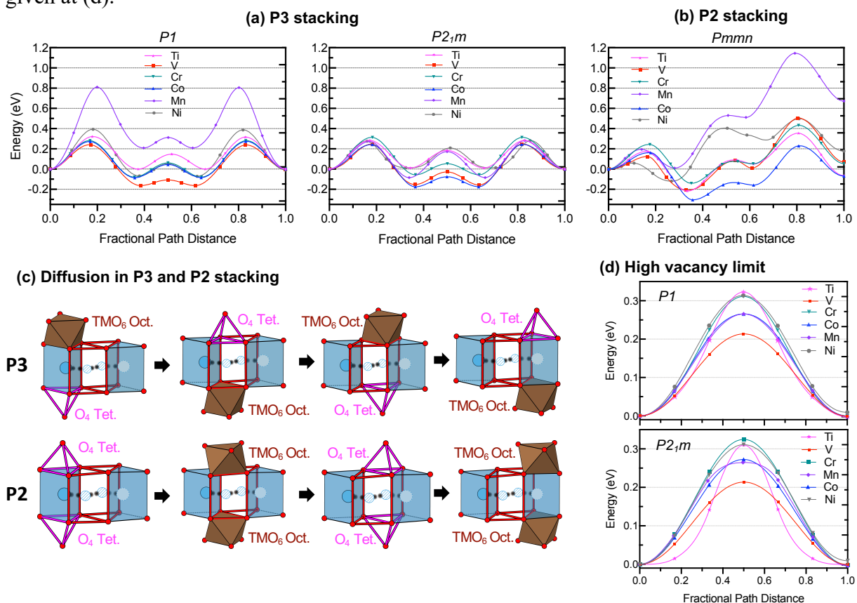
Figure 3. The minimum energy pathways for migration of Ca ion at the dilute vacancy limit in the various TM substituted layered-CaTM 2 O 4 with (a) P3 stacking (space group: P1, P2 1 /m) and (b) P2 stacking (space group: Pmmn). (c) Environments for Ca hopping in the layered-CaTM 2 O 4 with P3 and P2 stackings. Blue and red triangular prisms represent initial/final states and intermediate transition states, respectively. Brown octahedron (oct.) and magenta tetrahedron (tet.) illustrate TM and O 4 environments of the ends of triangular prims, respectively. The Ca migration barriers at the high vacancy limit in P3 stacking structures are given at (d).
