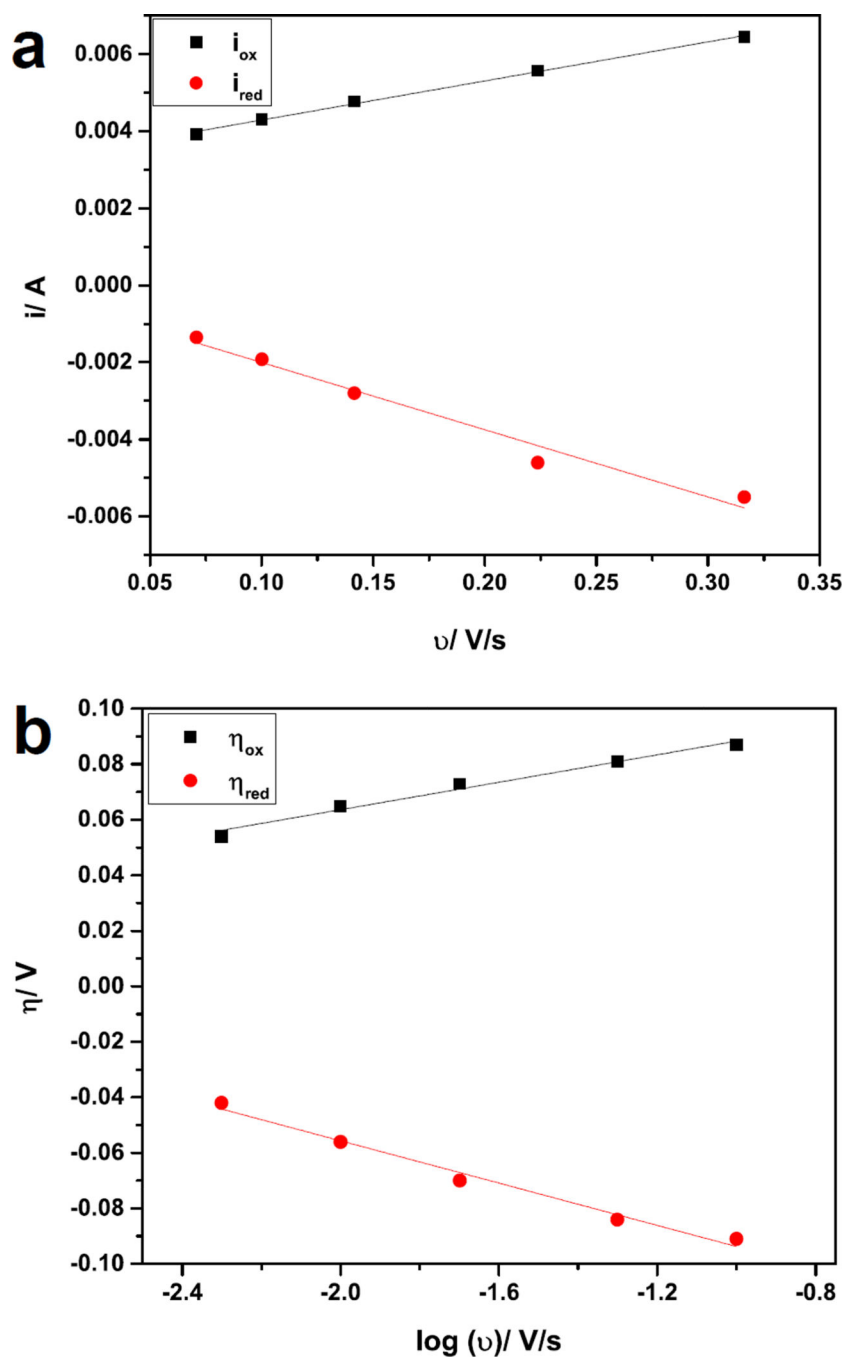
Figure 5. Representative current-scan rate dependence graph (a) and Laviron plot (b) for -N(CH_3)_3^+ modified gold electrode.
