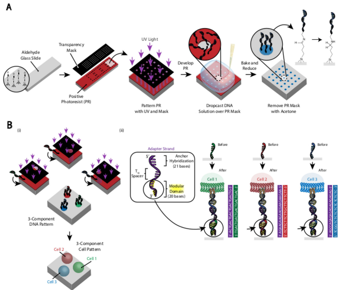
Figure 3: Photolithography is used to create the DNA-patterned slides that will ultimately dictate the placement of cells.
