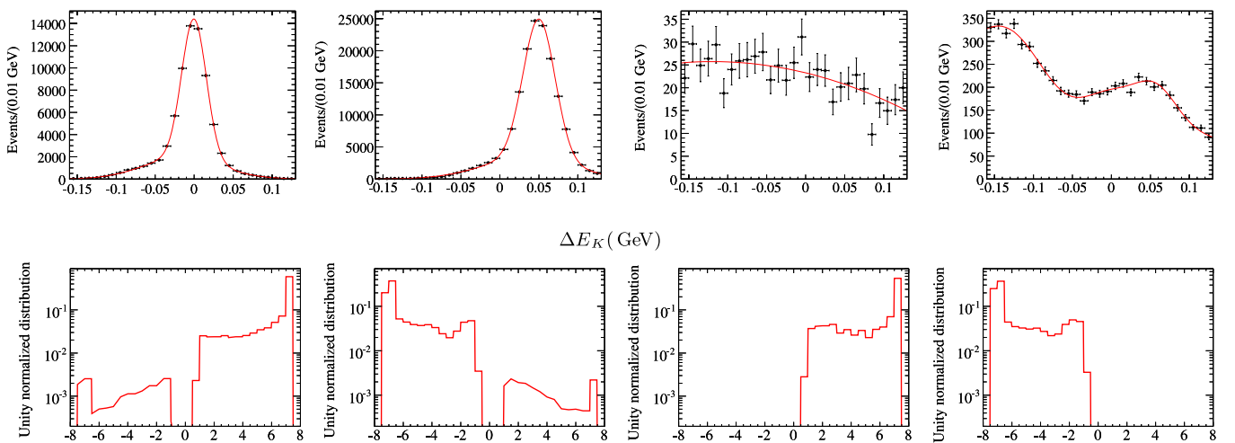
FIG. 1 (color online). Distributions of \Delta E_K (upper plots) and the PID variable \mathcal{T}_R (lower plots) from MC simulations of the categories (from left to right) D^*K , D^*\pi , B_K , and B_\pi (the latter two from B^+B^- , B^0\bar{B}^0 , and q\bar{q} MC samples), for the mode D^* \rightarrow D\pi^0 , D \rightarrow K^\pm\pi^\mp . In the upper plots, the dots represent the MC sample spectrum, and the curves show the PDFs. Note the vertical log scale in the lower plots.
