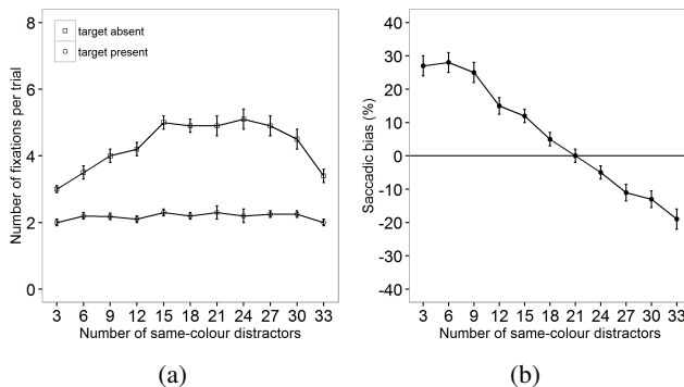
Figure 2: (a) Average number of fixations per trial as a function of the number of distractors sharing colour with the search target in target-absent trials and target-present trials for high discriminability condition. (b) Saccadic bias (the difference between the observed frequency and chance performance) as a function of the number of same-colour distractors in target-absent trials for high discriminability condition (Shen et al., 2003)
