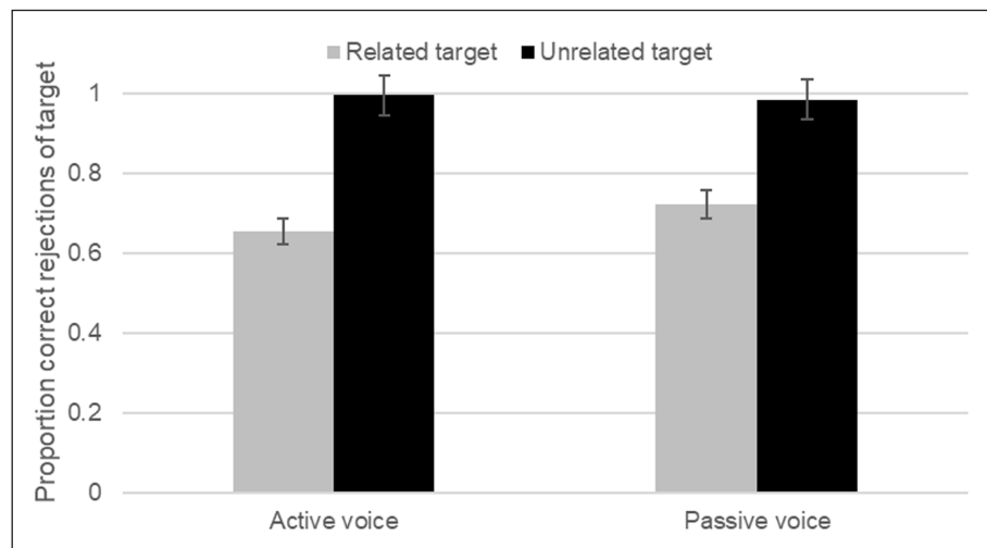
Figure 1: Proportions of correct rejections of the target in active voice and passive voice conditions (related target in grey bars, unrelated target in black bars). Error bars indicate 95% C.I.s.
