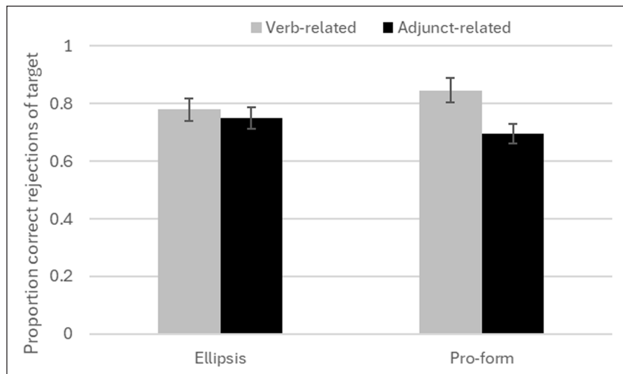
Figure 2: Proportions of correct rejections of the target in ellipsis and pro-form conditions (target related to the verb in grey bars, target related to the adjunct in black bars). Error bars indicate 95% C.I.s.
