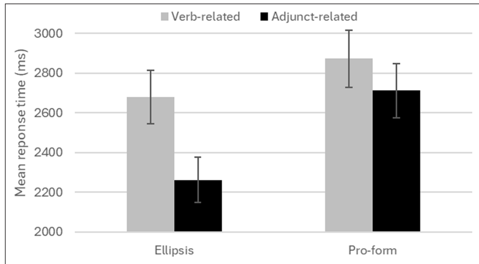
Figure 3: Mean response times for correct rejections of the target in ellipsis and pro-form conditions (verb-related target in grey bars, adjunct-related target in black bars). Error bars indicate 95% C.I.s.
