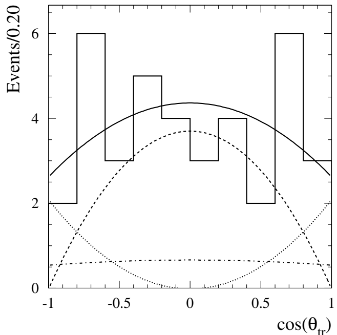
FIG. 2. The \cos\theta_{tr} distribution from the unbinned ML fit, superimposed on the histogram of the B^0 \rightarrow D^{*+} D^{*-} candidates in the signal region. The solid line represents the \cos\theta_{tr} distribution from the unbinned ML fit for the selected events. The dotted and dashed lines represent the fitted CP -odd and CP -even components, respectively, for the signal. The dot-dashed curve represents the fitted background component.
