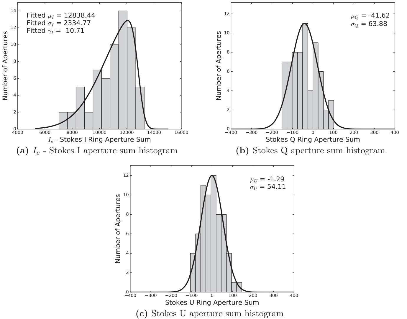
Figure 2. Histograms of the summed counts in the Stokes comparison apertures. The aperture size is equal to the full width at half maximum of the companion (3.44 pixels, or 0''.049 ). The Stokes I histogram (a) has an excess of higher values due to speckle noise. Because HD 19467 A is an unpolarized star, there is little flux at the companion’s separation in the Q and U frames. The large spread in Q and U values is due in part to the small number of apertures used (66).
