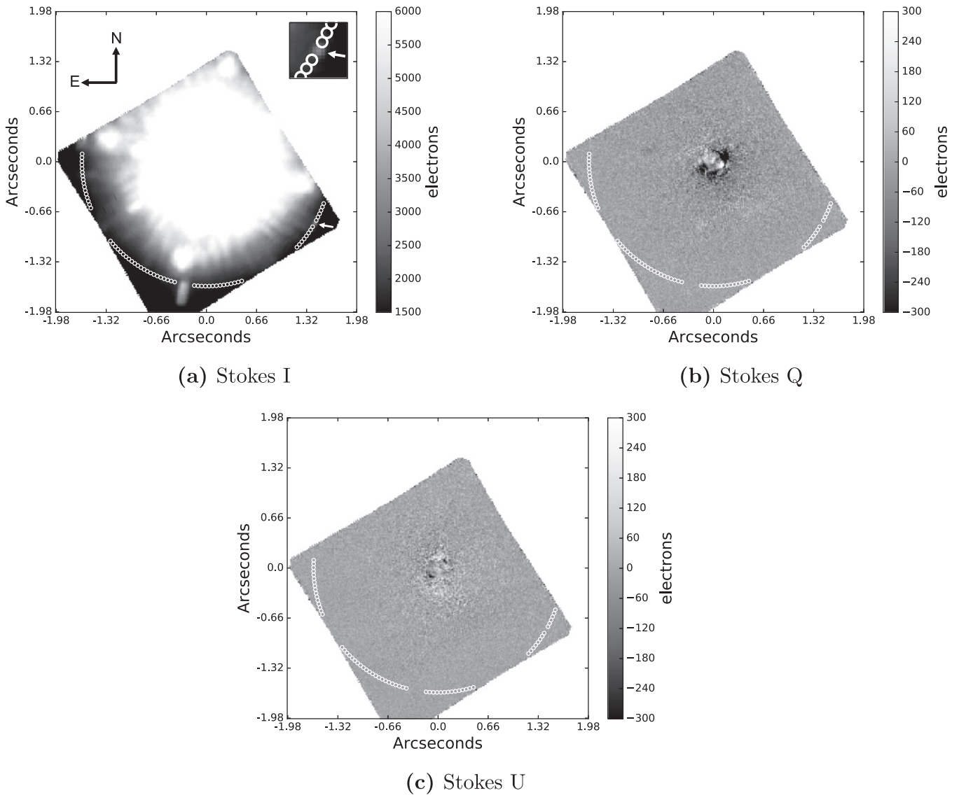
Figure 1. Reduced Stokes images with the ring of comparison apertures superimposed (the white arrow indicates the companion in Stokes I ). The companion’s S/N (Equation (1)) is 7.4 in Stokes I , but S/N < 1.0 in Stokes Q and U . Hence, no polarized radiation is detected from the companion.
