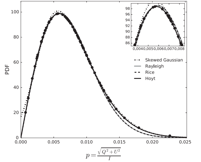
Figure 3. Probability density function of p = \frac{\sqrt{Q^2 + U^2}}{I} , via Equation (6). The four fits are to skewed Gaussian, Rayleigh, Rice, and Hoyt distributions. All but the skewed Gaussian are special cases of Equation (4) for different values of the means and standard deviations of Q and U . The best fit is the Hoyt distribution.
