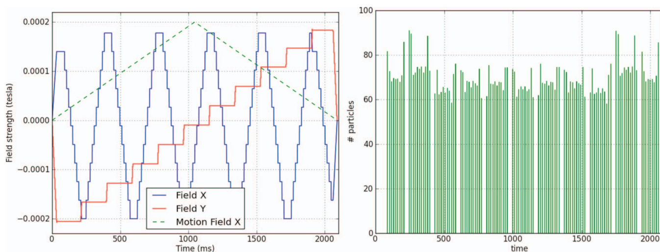
FIG. 15. Time dependence of X and Y dipole magnet fields, and triangular modulation of X field to compensate for patient motion (left). Number of particles simulated each time interval (right).
