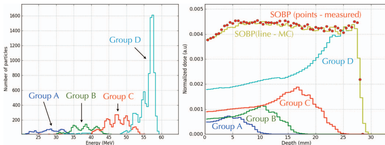
FIG. 9. Energy spectra of primary protons at isocenter grouped according to time as described in the text, averaged over a 1 \times 1 \text{ cm}^2 area (left). The partial SOBP for the full phase space from each time group is shown along with the summed SOBP for the 24 mm propeller (right). The dose was averaged over a 1 \text{ cm} \times 1 \text{ cm} \times 0.05 \text{ cm} volume. The published measurement for this propeller is also shown (Ref. 48).
