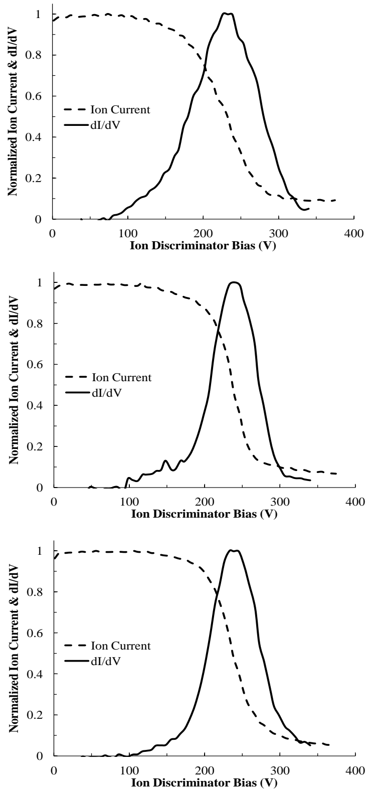
Figure A-2. Normalized ion current and dI/dV as a function of RPA ion discriminator potential for operation of the MaSMi-60 at 250 V and 250 W (top), 400 W (middle), and 550 W (bottom).
