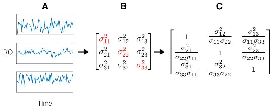
Figure 2: Relations between the calculation of FC and BV. Time series for three ROIs (A) are used to compute the covariance matrix (B) where \sigma_{ij}^2 represents the covariation between ROIs i and j and the red diagonal entries represent BV. The covariance (B) can be used to compute the Pearson correlation matrix (C), where the ij -th entry of the matrix is \sigma_{ij}^2/(\sigma_{ii}\sigma_{jj}) . FC can refer to either the covariance matrix, which explicitly includes BV, or the correlation, which indirectly includes information about the variance. FC is traditionally computed as the correlation and the diagonal of ones is discarded.
