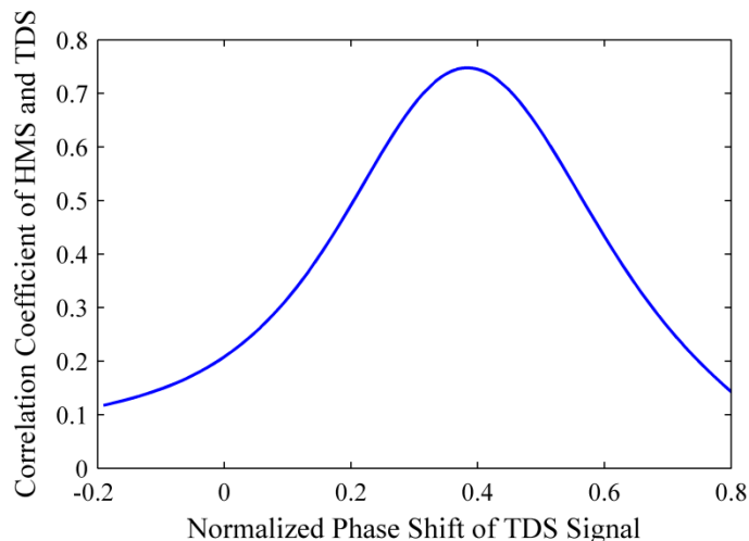
Fig. 2.4.5 Correlation coefficient between HMS and TDS signal with different phase shift
