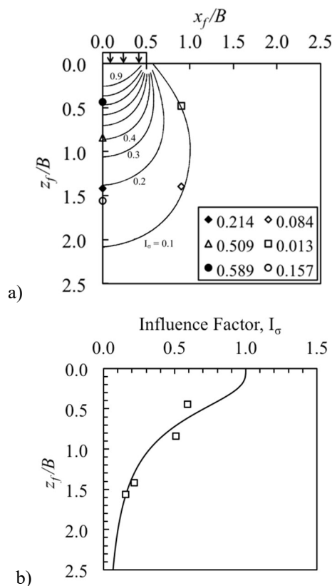
Figure 12. Comparison of measured results with Newmark's solutions for square footings (Newmark 1935): a) Two dimensional stress bulbs; b) Influence factors directly beneath footing
