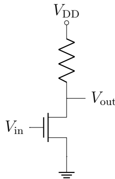
Figure 3.6: Schematic of nmos input common source (CS) amplifier
