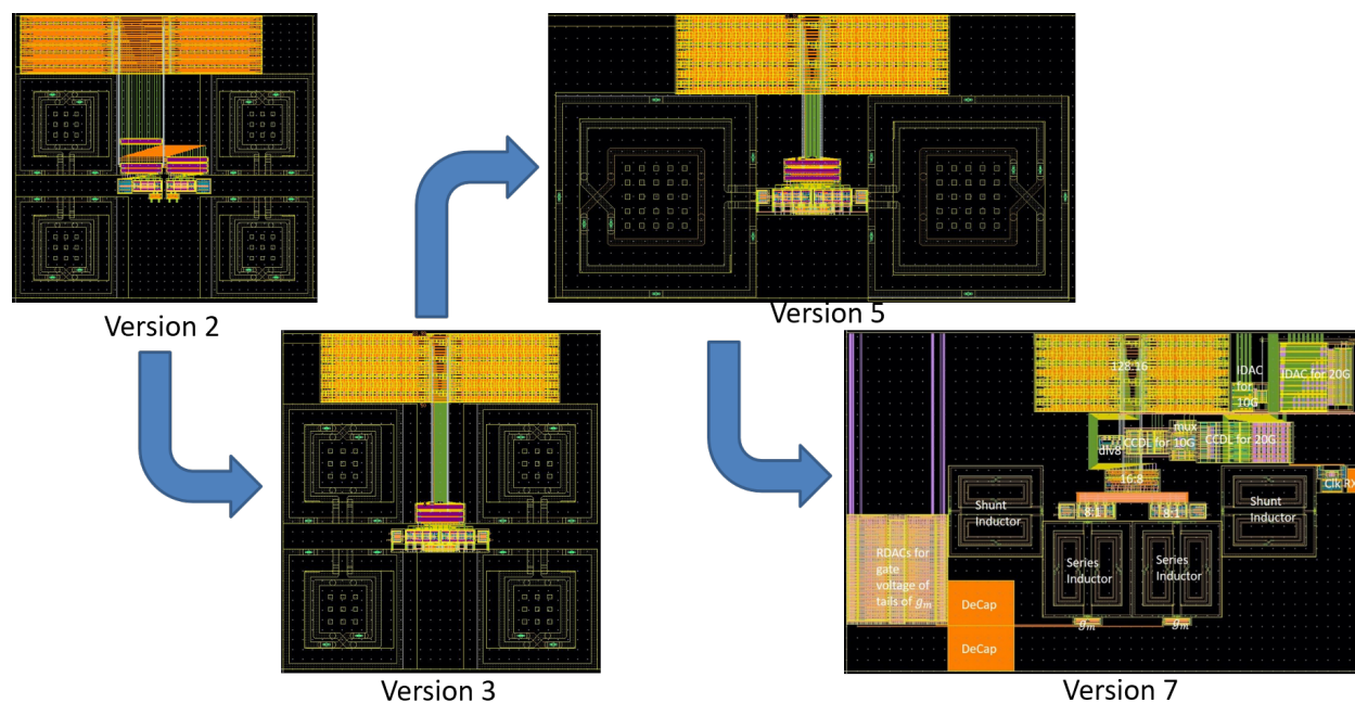
Figure 6.5: TX Datapath Floorplan Iterations in BAG 3++
