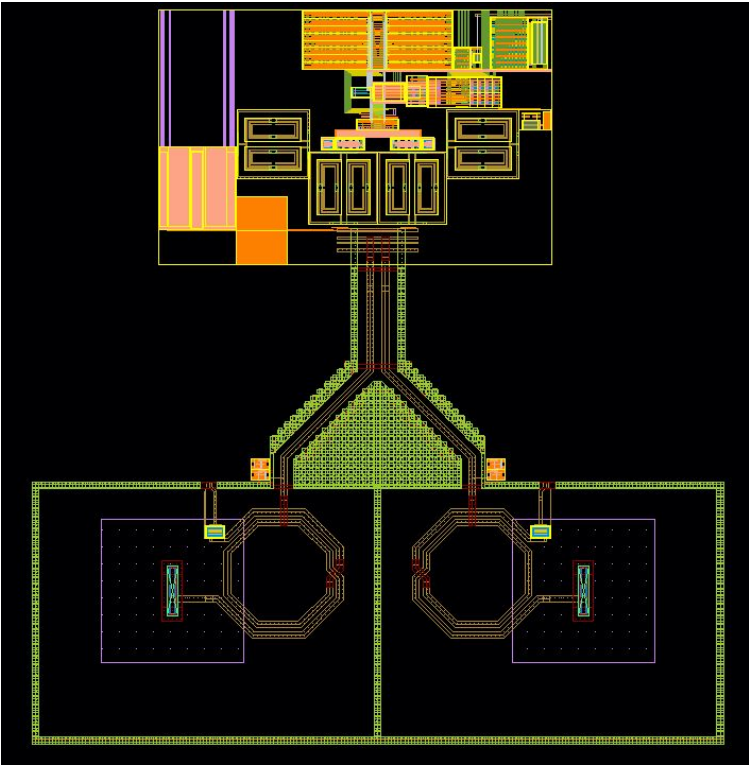
Figure 3.11: Manually Integrated Transmitter Datapath Top Level Layout
