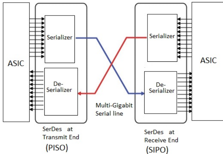
Figure 3.1: Overview of SerDes
