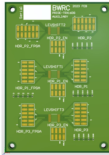
Figure 7.3: 3D view of Auxiliary PCB from Altium Designer
