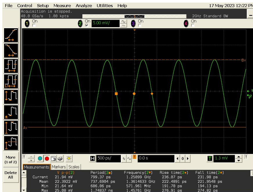
Figure 7.7: Output Divided Clock (20 GHz Injection)
