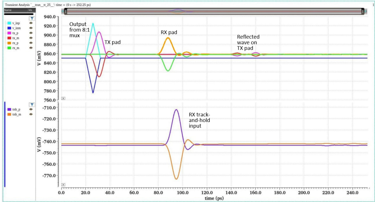
Figure 6.2: Waveforms from Transmitter Output Driver Simulation
