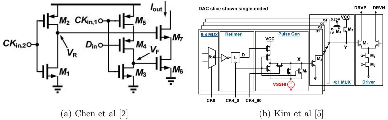
Figure 4.1: 1 UI Pulse Generator Architecture Options
