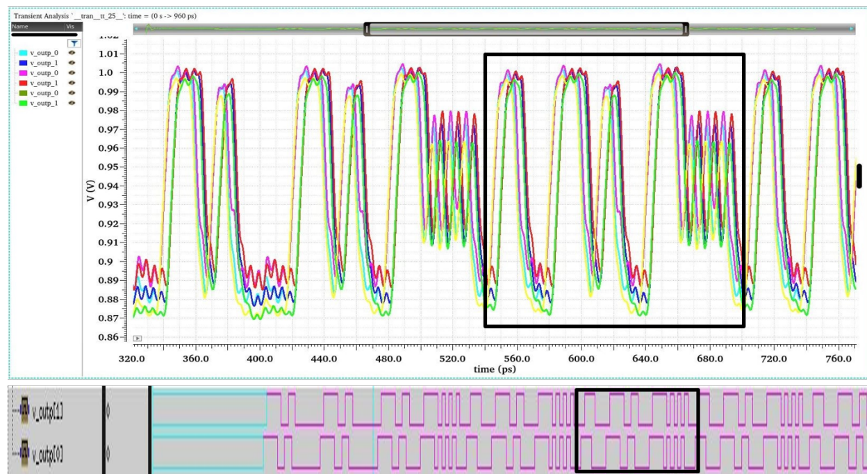
Figure 6.4: TX Logic Verification from Extracted (top) and Behavioral (bottom) Simulations
