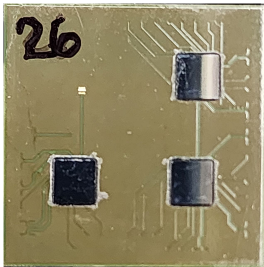
(a) Photograph of Die attached Package
