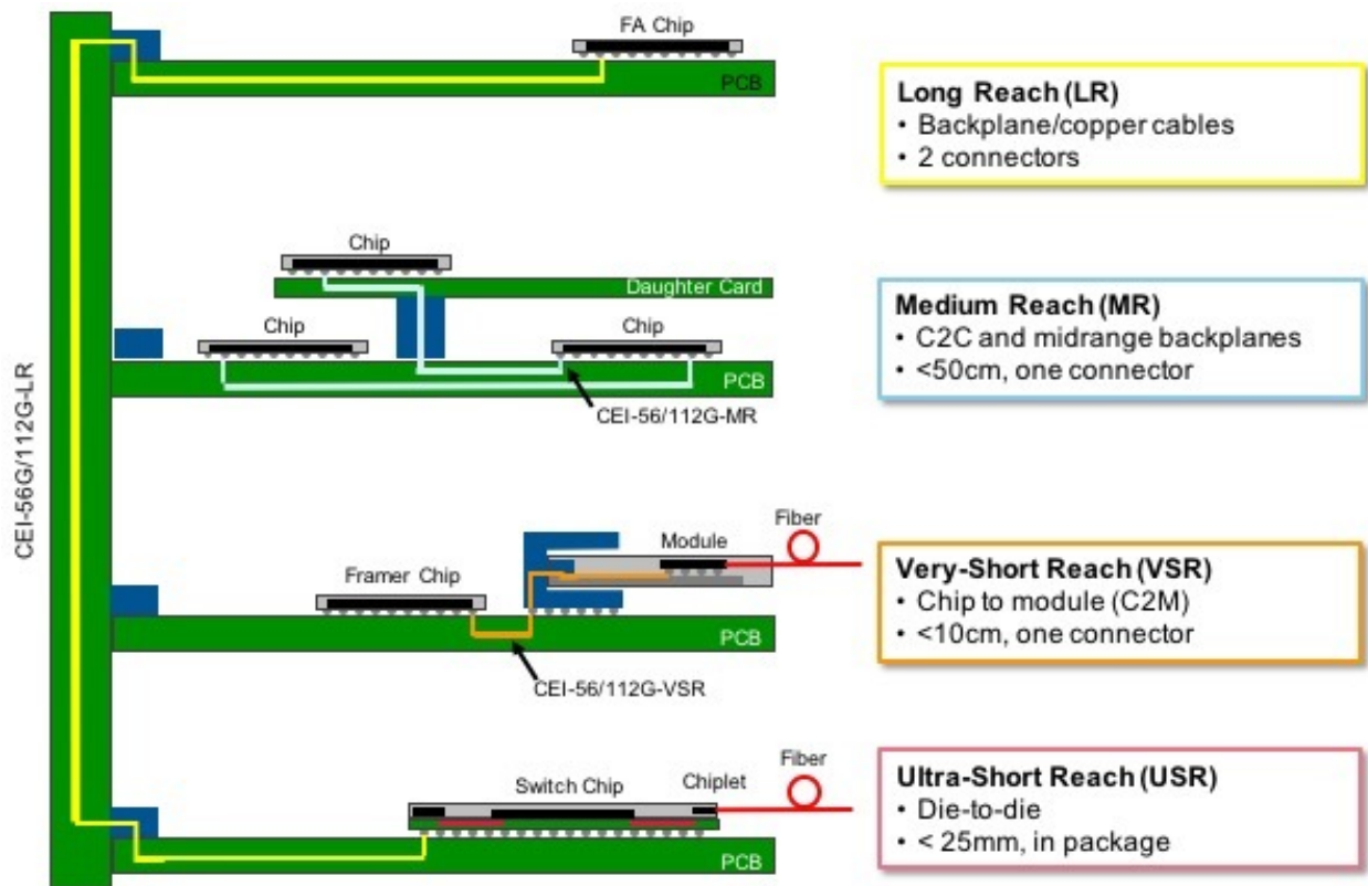
Figure 3.2: Different SerDes Reaches
