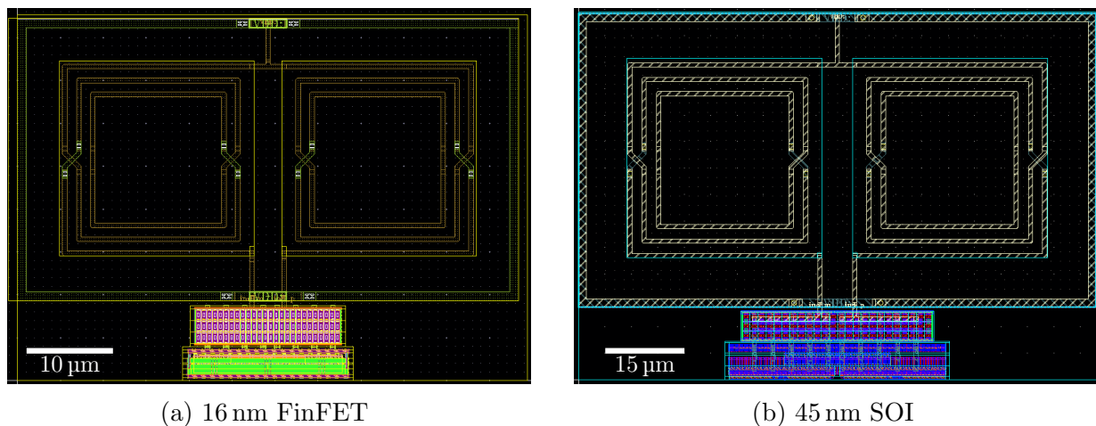
Figure 2.5: Optimal layouts based on Table 2.2
