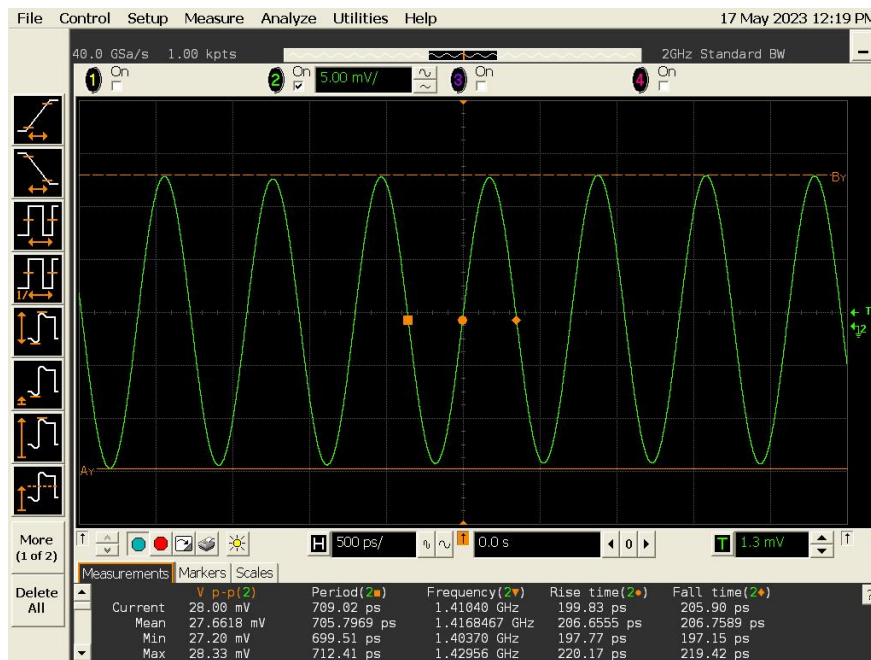
Figure 7.6: Output Divided Clock (Free Running)
