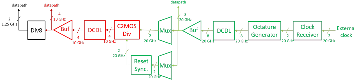
Figure 3.9: Complete Transmitter Clock Network Architecture
