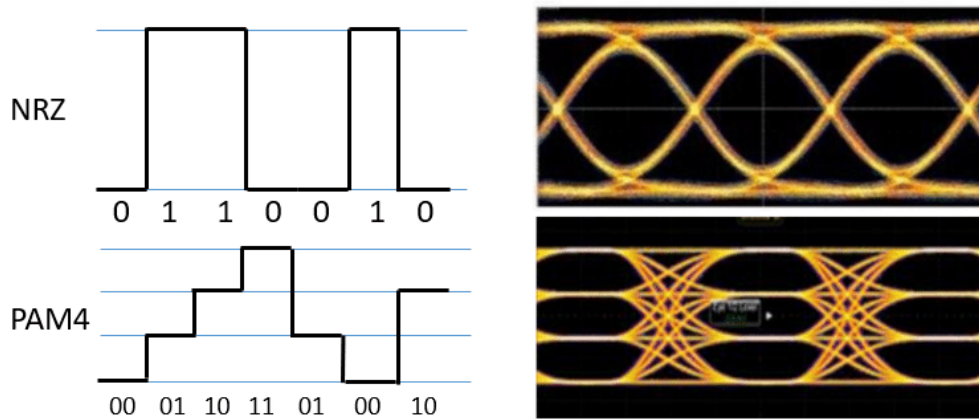
Figure 3.5: NRZ and PAM4 signalling waveforms and eye diagrams
