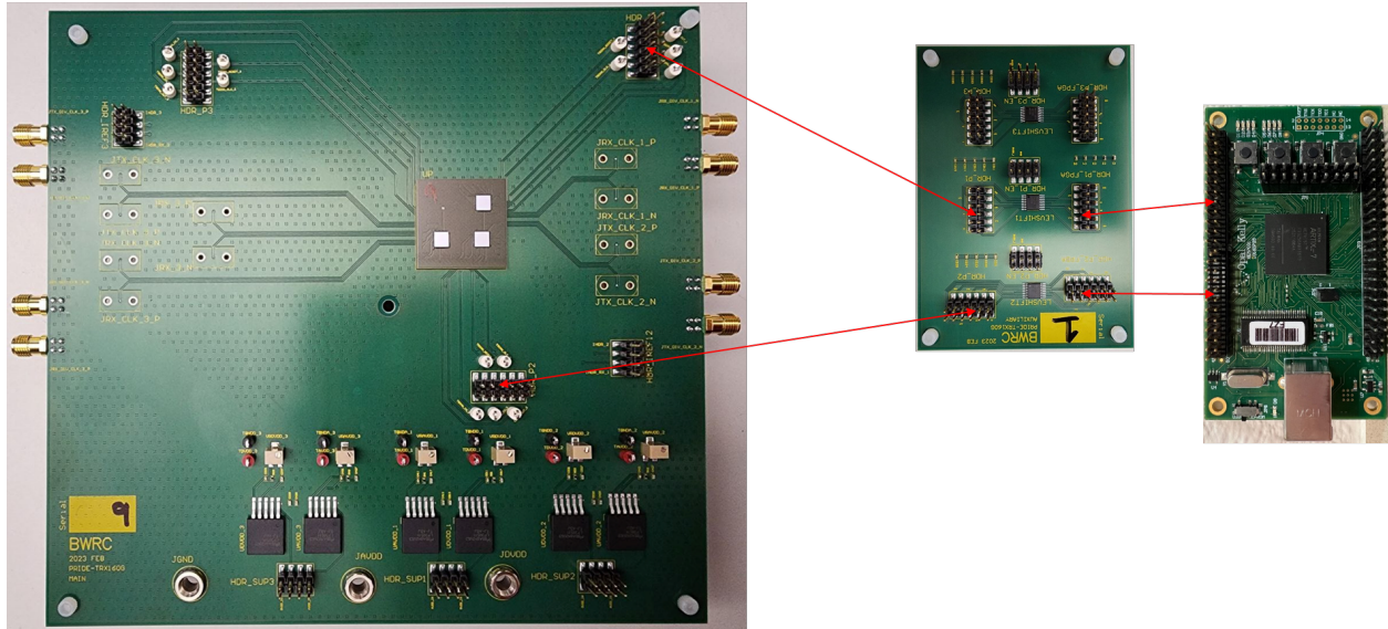
Figure 7.5: Setup of PCBs and FPGA for loopback testing
