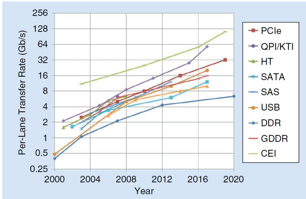
Figure 3.4: Wireline I/O trends [3]
