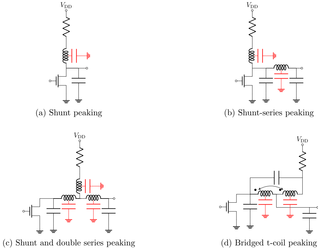
Figure 4.2: Common Peaking Topologies
