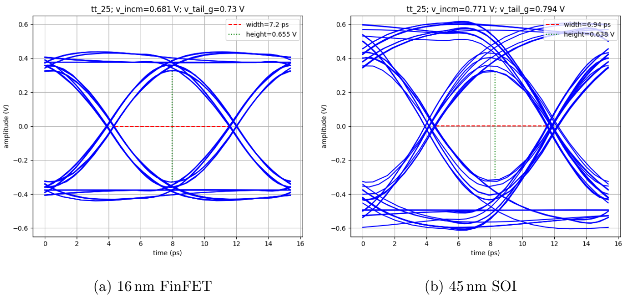
Figure 2.6: Eye diagrams for TT@25°C corner based on Table 2.2
