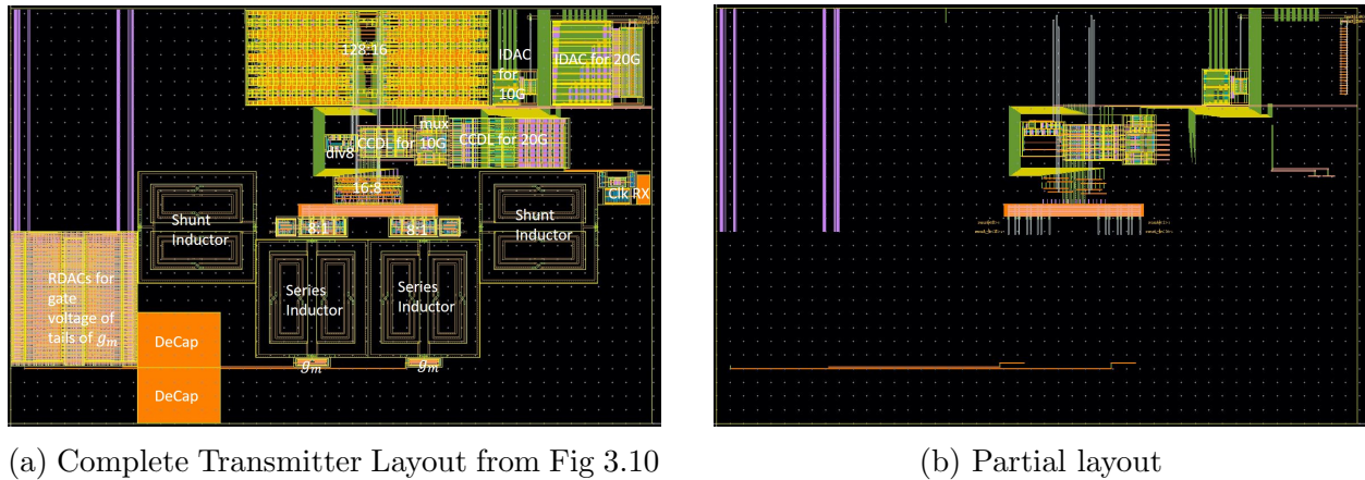
Figure 5.3: Partial Layout for Datapath Timing Verification at Clock Crossing Interface
