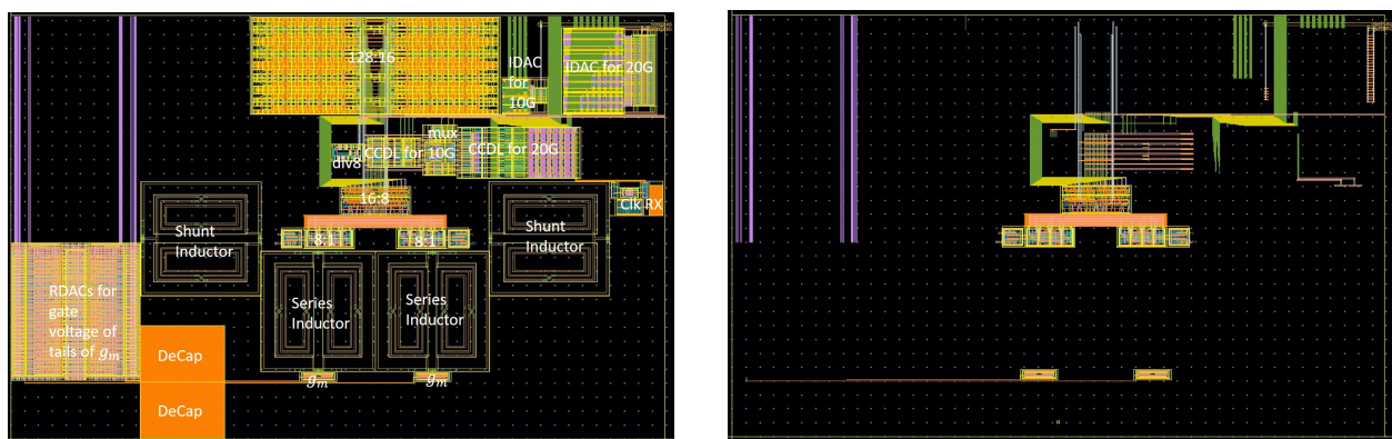
(a) Complete Transmitter Layout from Fig 3.10
