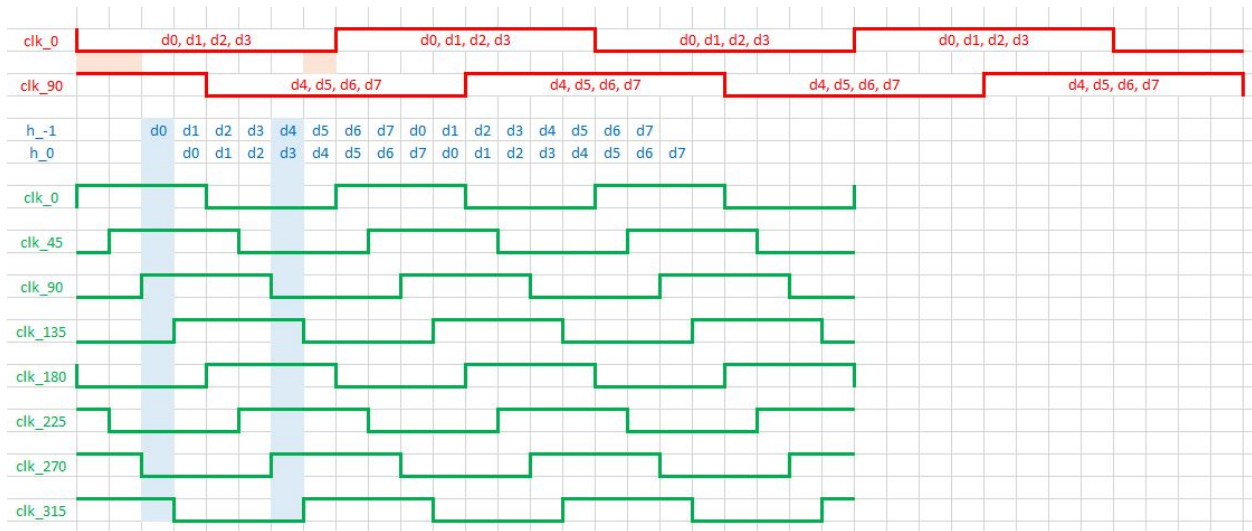
Figure 5.1: Timing diagram at clock crossing interface: Ideal scenario
