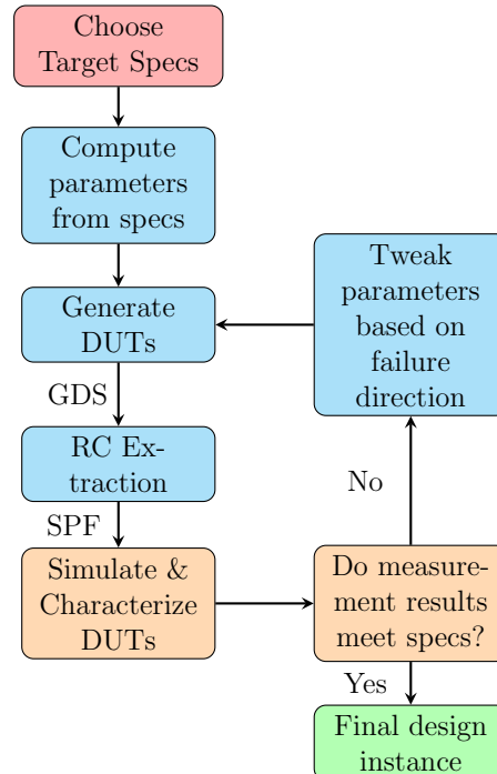
Figure 1.2: Flowchart for Iterative / Serial Design Script
