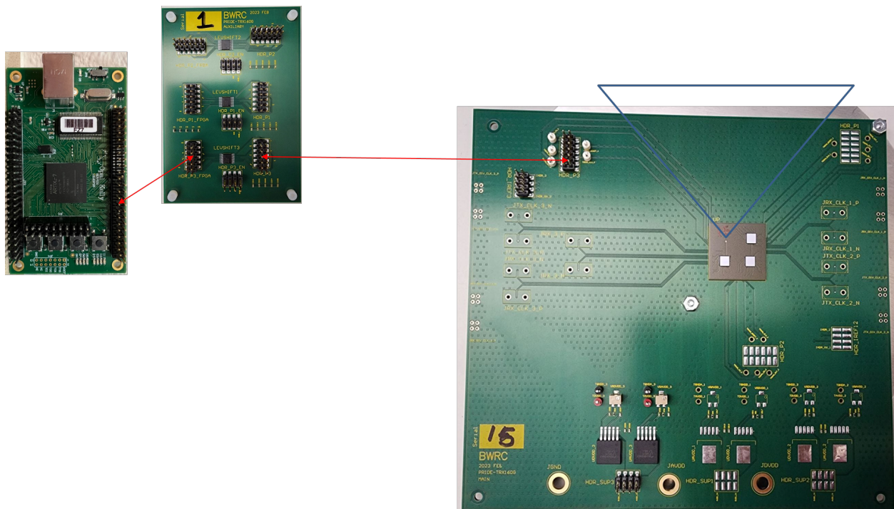
Figure 7.4: Setup of PCBs and FPGA for stand-alone TX probing
