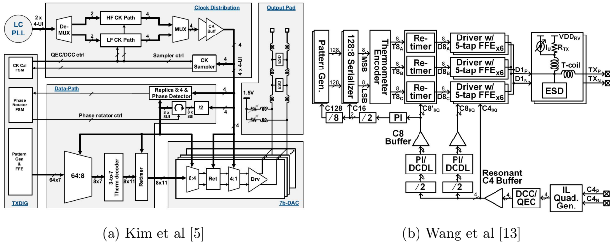
Figure 3.7: Comparison of State-of-the-Art Transmitter Architectures
