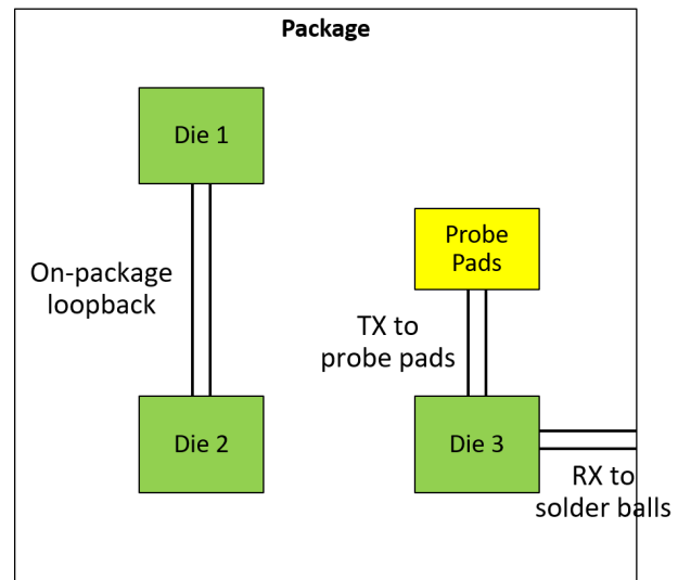
(b) Balls-up overview of the MCP
