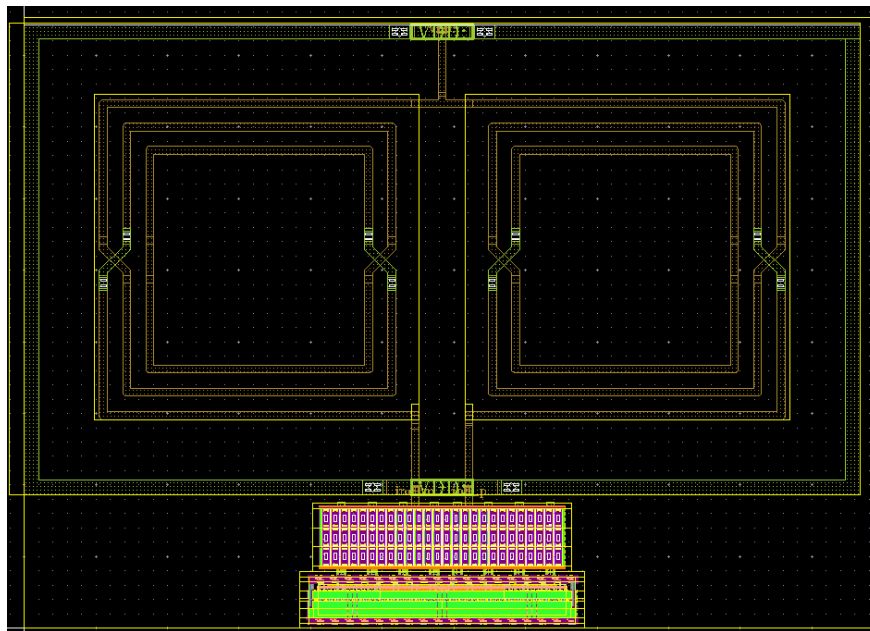
Figure 2.3: Full layout of the Output Driver DUT from Fig 2.2
