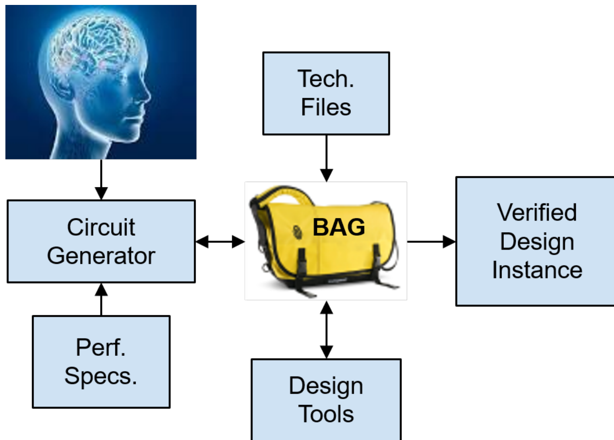
Figure 1.1: Overview of Berkeley Analog Generator (BAG) framework
