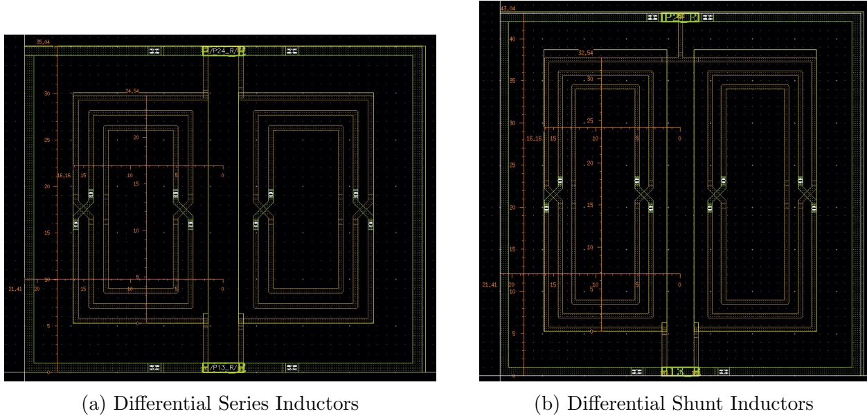
Figure 4.4: Optimized BAG 3++ generated layouts of inductors for peaking of 8:1 mux
