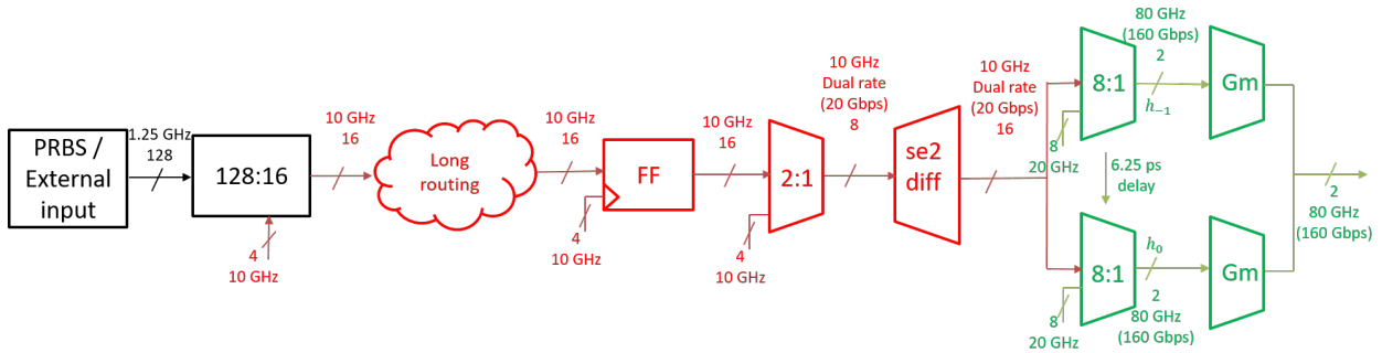
Figure 3.8: Complete Transmitter Datapath Architecture
