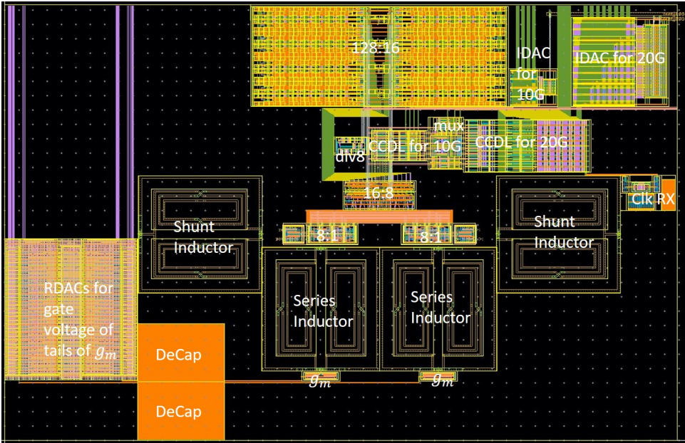
Figure 3.10: BAG 3++ Generated Transmitter Layout with annotated components
