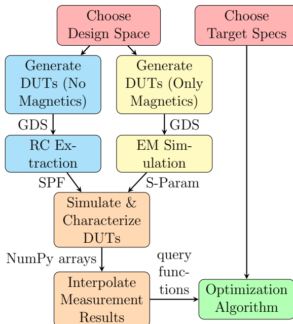
Figure 2.1: OptDesigner co-optimization loop
