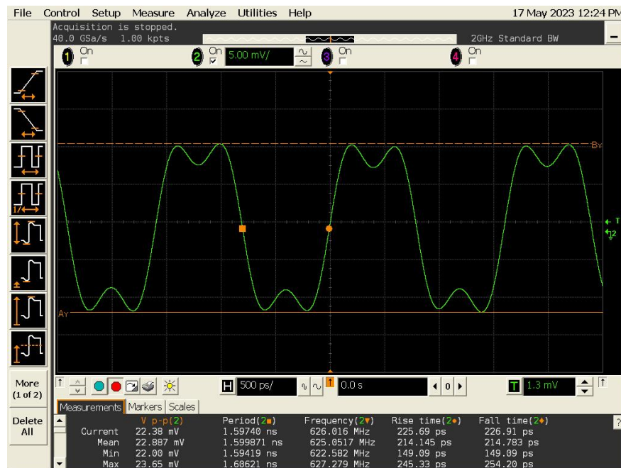
Figure 7.8: Output Divided Clock (10 GHz Injection)
