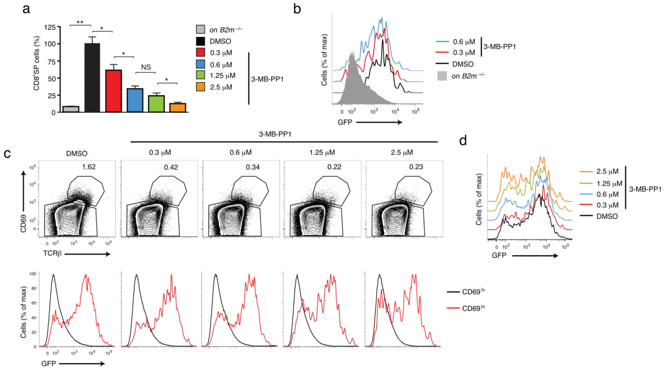
Figure 5. Invariant Zap-70 dependent signal threshold for positive selection (a) Pre-selection OT-I Zap-70(AS)-Nur77-GFP DP cells were cultured on WT thymic slices for 72 hours in the presence of the indicated concentrations of 3-MB-PP1. Graph displays the average percentage of CD8 + SP (± s.e.m.) from technical triplicate samples detected at 72 hours, normalized to the average of the DMSO only control samples. (b) Histograms show GFP expression by the CD8 + SP populations from indicated inhibitor treatment conditions. Closed gray histogram shows the GFP expression on DP cells cultured on non-selecting B2m -/- thymic slices. (c) Zap-70(AS)-Nur77-GFP thymic lobes were cultured for 7 days in the presence of the indicated concentrations of 3-MB-PP1. Flow cytometry plots are gated on DP cells and the numbers indicate the percentage of cells within the TCRβ hi CD69 + population (top). Histograms show GFP expression of TCRβ - CD69 - DP cells (black) versus TCRβ hi CD69 + cells (red) (bottom). (d) GFP expression of the TCRβ hi CD69 + cells from Zap-70(AS)-Nur77-GFP FTOC. Data from (a,b) are representative of 2 independent experiments. Data from (c,d) are representative of 3 independent experiments. * P < 0.05, ** P < 0.0005, NS not significant (Student's t -test).
