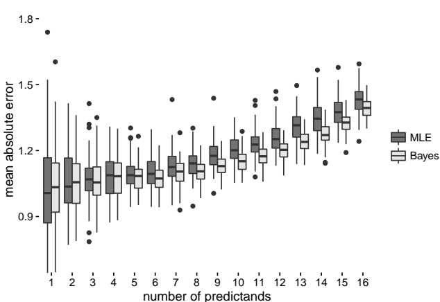
Fig. 4. Tobamovirus data, comparing the Grassmann manifold Bayesian model to standard MLE model. The 18 elements of the hold-out vector are assigned to be predictors and predictands, with the displayed prediction error an average over 100 random assignments. As the number of predictands increases (and number of predicting elements decreases) element-wise errors increase, and the Bayesian implementation outperforms amid greater uncertainty.
