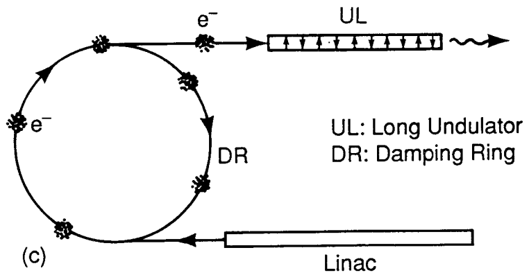
Fig.1 Storage ring FEL configurations in the (a) small and moderate gain oscillator mode, (b) high-gain bypass mode and (c) high-gain single pass mode.
