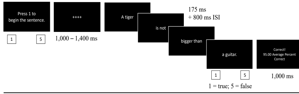
Figure 1: Trial structure.
