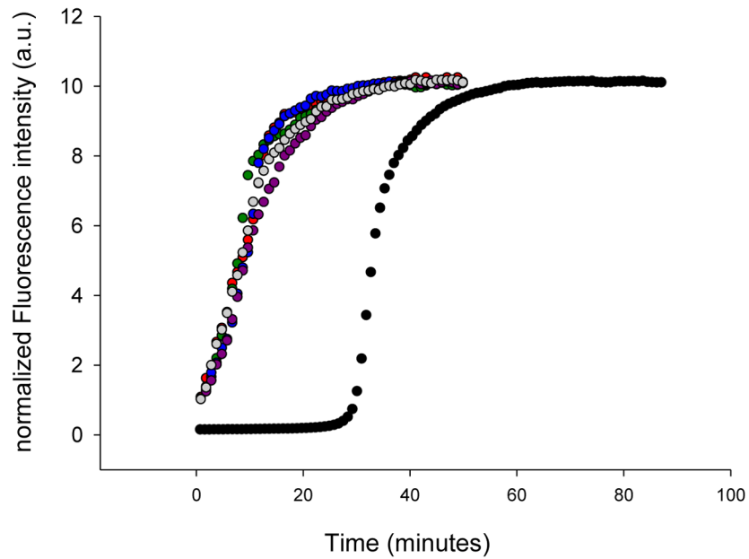
Figure 8. The position-15 variants effectively seed amyloid formation by wild-type IAPP. The results of thioflavin-T fluorescence monitored seeding experiments are shown. Black, unseeded wild-type IAPP amyloid formation; grey, wild-type IAPP seeded by wild-type IAPP amyloid fibrils; red, wild-type IAPP seeded by F15L-IAPP amyloid fibrils; blue, wild-type IAPP seeded by F15NLe-IAPP amyloid fibrils; green, wild-type IAPP seeded by F15I-IAPP amyloid fibrils; purple, wild-type IAPP seeded by F15TLe-IAPP amyloid fibrils.
