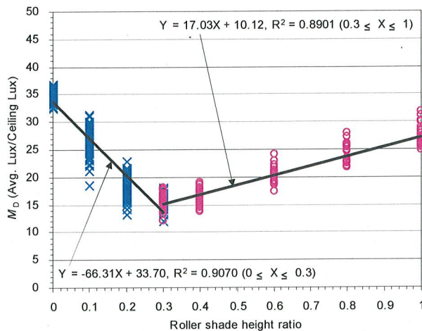
Fig. 10. Linear relationship of M_D to roller shade height on the 60^\circ photosensor.
