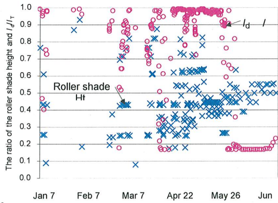
a) Improved closed-loop proportional with roller shade height
