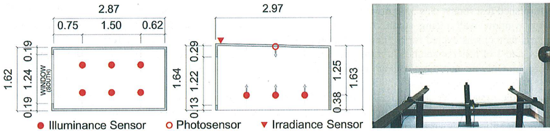
Fig. 2. Floor plan and section for the sensors' positions, and interior view of the test room for the half-scale testbed. Dimensions are given in meters.
