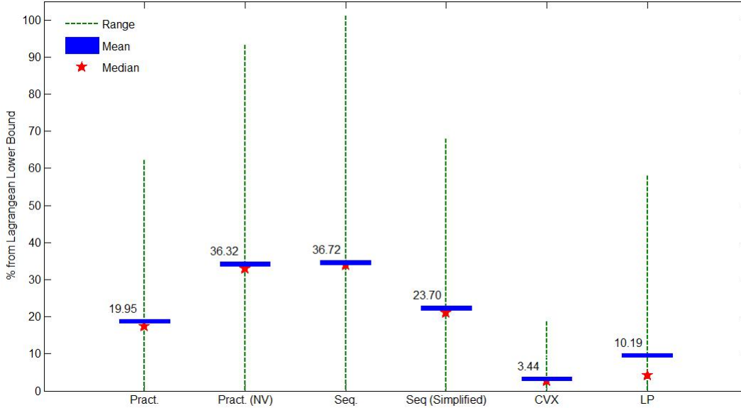
Figure 2: Suboptimality Gap
