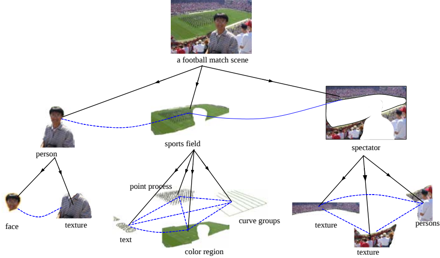
Fig. 1. Image parsing example. The parsing graph is hierarchical and combines generative models (downward arrows) with horizontal connections (dashed lines), which specify spatial relationships between the visual patterns. See Figure 4 for a more abstract representation including variables for the node attributes.
