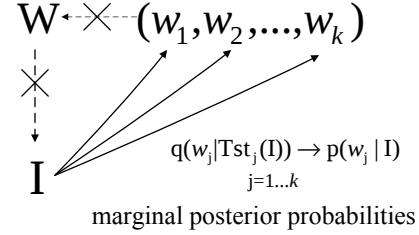
Fig. 3. Comparison of two inference paradigms: Top-down generative methods versus bottom-up discriminative methods. The generative method specifies how the image \mathbf{I} can be synthesized from the scene representation W . By contrast, the discriminative methods are based by performing tests \text{Tst}_j(\mathbf{I}) and are not guaranteed to yield consistent solutions, see crosses explained in the text.
