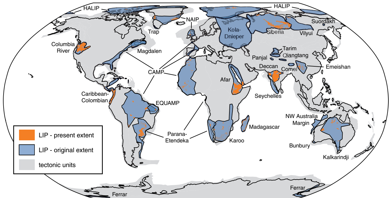
Figure 7.1. Map of current surface extent of volcanic lithologies associated with LIPs that erupted between 520 Ma and the present, as well as the estimates of the initial LIP surface extent used in the area analysis (modified slightly from Ernst & Youbi, 2017, and Ernst et al., Chapter 1 this volume, to ensure that all currently exposed volcanic lithologies are encapsulated by the initial LIP surface area polygons).
