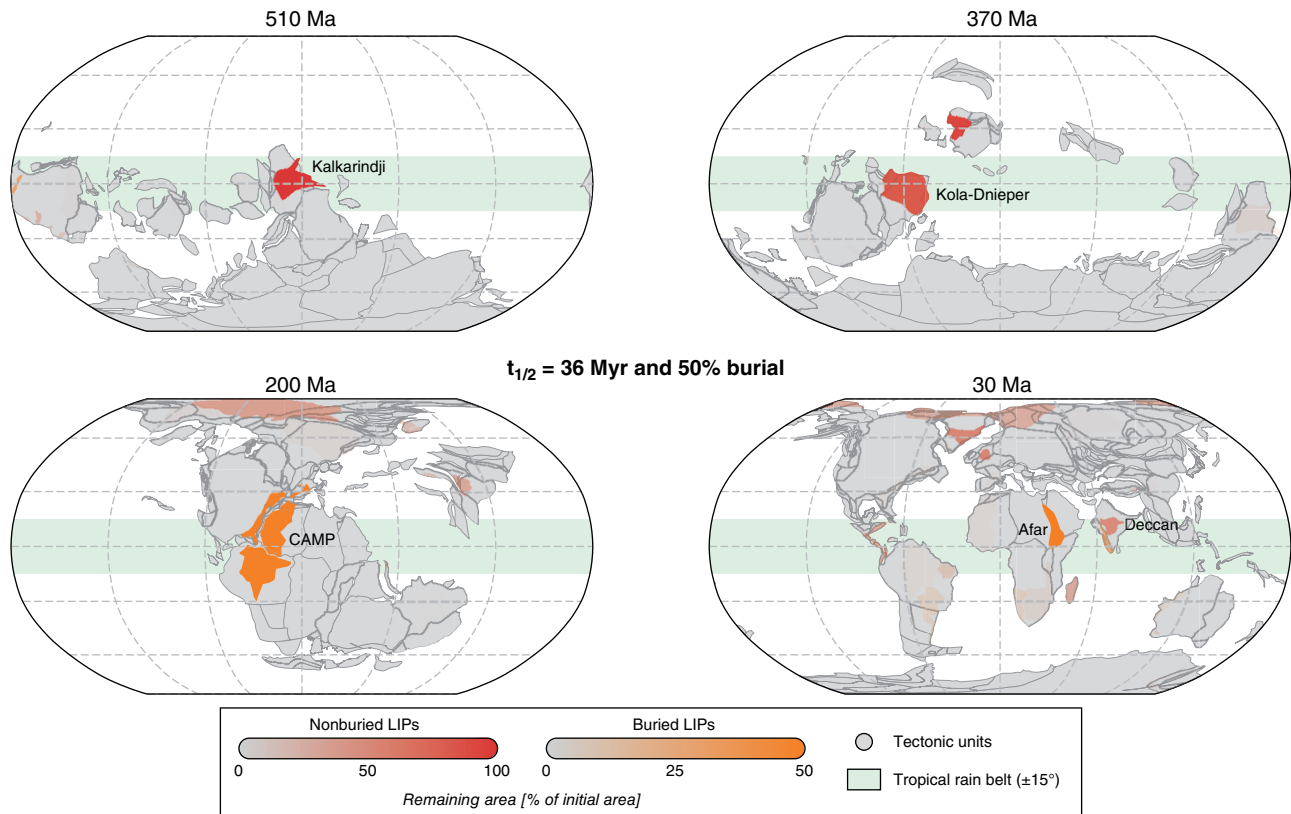
Figure 7.5 Paleogeographic reconstructions for times that correspond to peaks of LIP area in the tropics (Fig. 7.4c). The opacity of LIP polygons indicates their parameterized remaining area at the time of the reconstruction as a percentage of initial LIP area, under the preferred post-emplacement scenario of t_{1/2} = 36 Myr + 50% burial.
