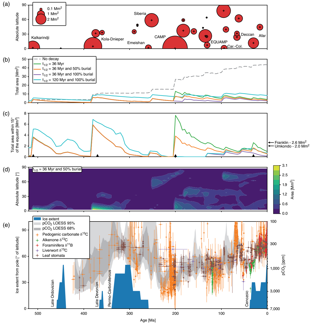
Figure 7.4 (a) LIPs included in this analysis. The size of each circle reflects the initial surface area estimate of each LIP. The + indicates the timing and absolute paleolatitude of the centroid of each LIP at the time of emplacement. Car.-Col. = Caribbean-Colombian. (b) Total LIP area through time for the different post-emplacement scenarios. Only the “no decay” scenario excludes pre-Phanerozoic LIPs. (c) Tropical LIP area through time for the different post-emplacement scenarios. The arrows to the right indicate reconstructed tropical LIP area at the time of emplacement for the ca. 720 and 1,109 Ma Franklin and Umkondo LIPs. The triangles show the paleogeographic reconstruction times in Figure 7.5. (d) Contour plot showing the latitudinal distribution of LIP area for one of the post-emplacement models. (e) Latitudinal extent of land ice away from the poles (Macdonald et al., 2019) and compilation of p\text{CO}_2 proxies (Foster et al., 2017) ( p\text{CO}_2 y-axis reversed, and in log-scale). Error bars indicate standardized uncertainties, and grey bands indicate 68% and 95% confidence intervals for Monte Carlo resampled LOESS fits to the p\text{CO}_2 proxy data (Foster et al., 2017). Note that there are p\text{CO}_2 proxy estimates <100 ppm that are cut off in this plot.
