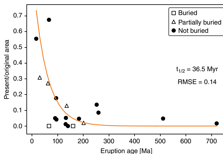
Figure 7.2 LIP erosion through time. The ratio of estimates of the present-day surface area to that of the original surface area are shown for 19 basaltic LIPs. An exponential fit is made to the 13 basaltic LIPs that are interpreted to not have been buried after emplacement (Table 7.1), which yields a half-life of ~36 Myr. RMSE = root mean square error.
