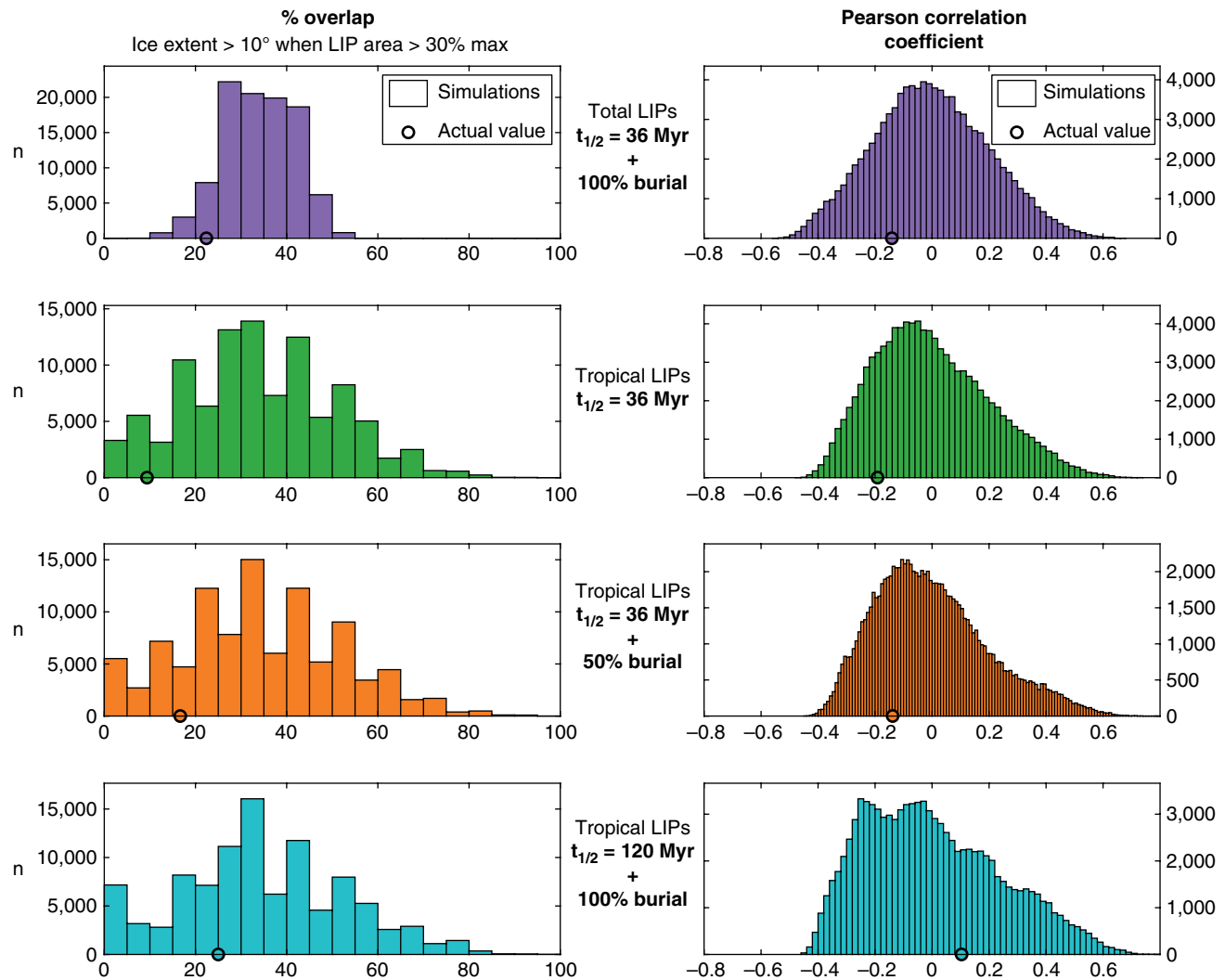
Figure 7.6 The percent (%) overlap and Pearson correlation coefficients between LIP area and the actual ice-extent record are shown with circles. These values are compared with histograms that show the range of values that arise when comparing the LIP area record to glacial intervals that have been shifted randomly in time 100,000 times. The fraction of randomly timed glacial interval simulations that correlate/overlap better with LIP area than the actual ice-extent record is the p-value shown in Table 7.2.
