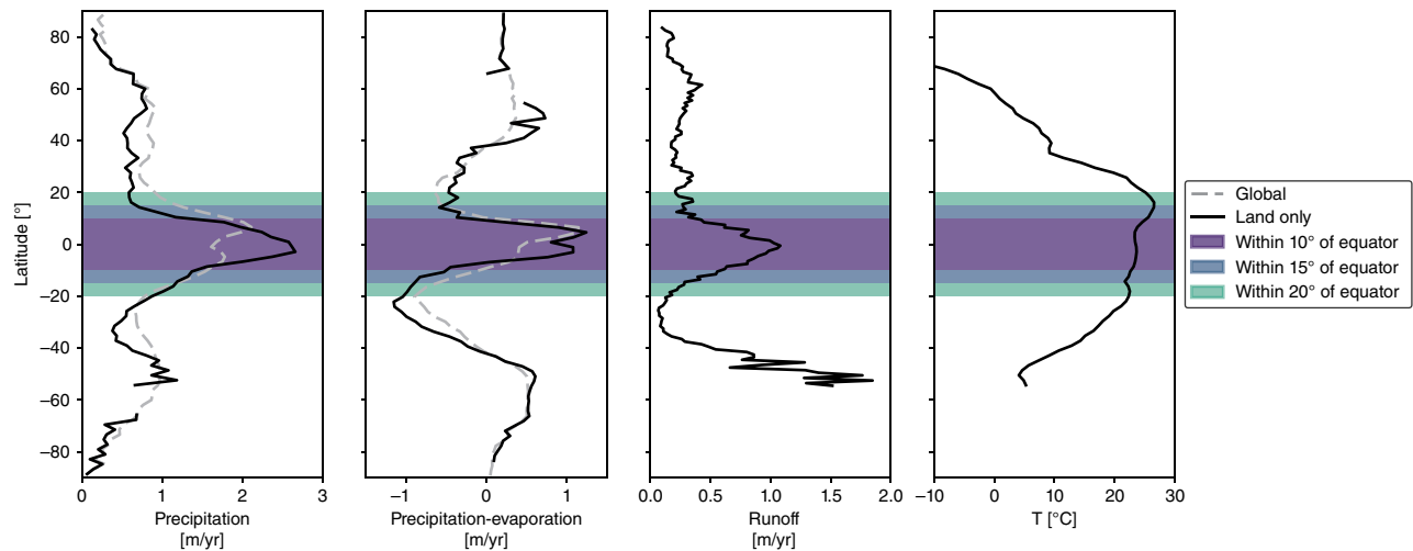
Figure 7.3 Zonally averaged modern climatological data used to define the tropical rain belt. The global precipitation (Kalnay et al., 1996) and precipitation minus evaporation (Trenberth et al., 2011) data include land and ocean pixels; global temperature data (Kalnay et al., 1996) are from land only; and runoff data (Fekete et al., 1999) are from land only excluding Antarctica. The peak in runoff \sim 50^\circ is due to anomalously high orographically induced runoff in the southern Andes, which represents almost all of the land in that latitude belt. Temperature data for Antarctica are off scale. Precipitation, precipitation minus evaporation, and runoff all increase sharply between \pm 10^\circ and \pm 15^\circ .
