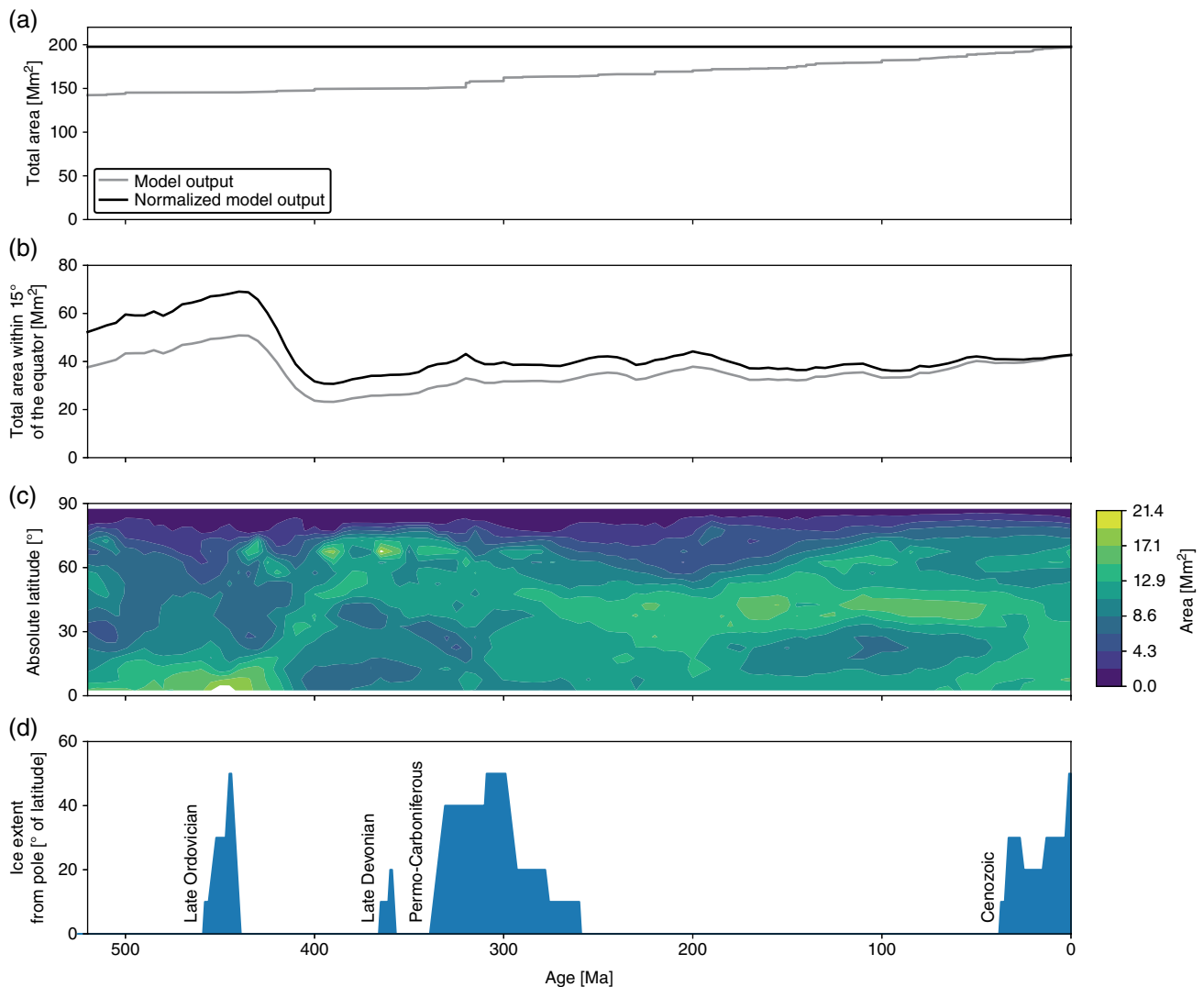
Figure 7.7 (a) Total continental area through time. In the paleogeographic model used in this study, tectonic units (Torsvik & Cocks, 2016) are progressively added to the model, leading to a net increase in total continental area in the model of \sim 33\% over the Phanerozoic. However, estimates of continental crust growth (e.g., Pujol et al., 2013) suggest that the continental area was roughly constant through the Phanerozoic. We therefore normalize the total continental area curve in our model by assuming (a) fixed continental area through the Phanerozoic. (b) Tropical continental area through time: we normalize the tropical continental area curve using the normalization ratio implied in (a). (c) Contour plot showing the latitudinal distribution of continental area. (d) Latitudinal extent of land ice away from the poles (Macdonald et al., 2019).
