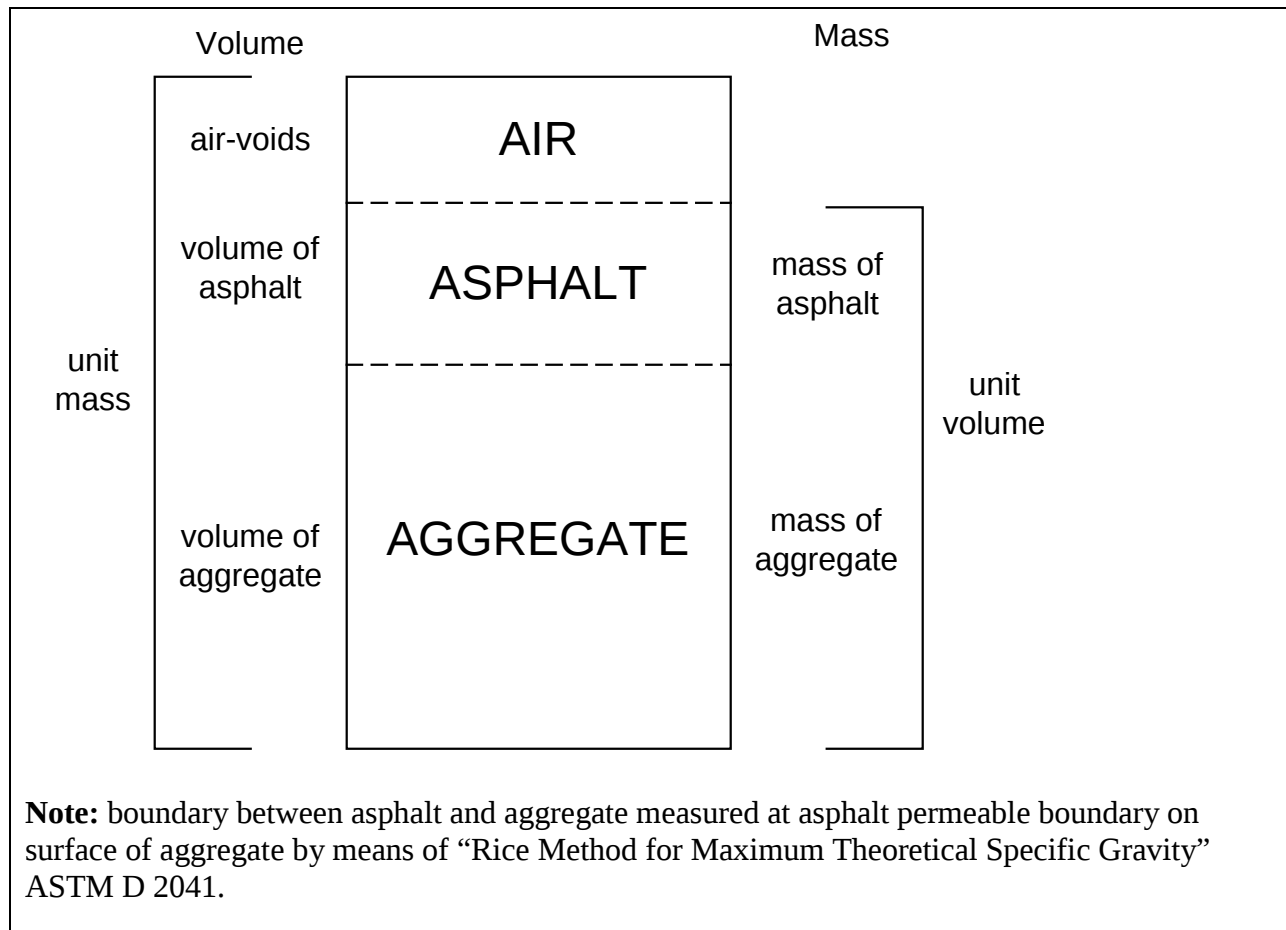
Figure 1. Volumetric Components of Asphalt Concrete, and Measurement of Degree of Compaction.
