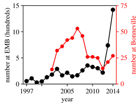
Figure 1. Columbia River and incidence of California sea lions at East Mooring Basin (EMB) and Bonneville Dam. The maximum California sea lions observed at EMB (black) and average daily number of Bonneville foragers in each year (red). (Online version in colour.)
