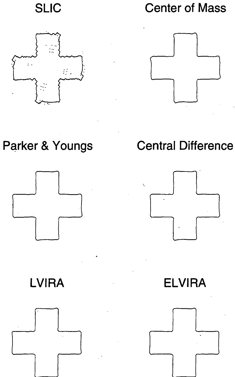
Figure 4.2 A cross that has been rotated one revolution using the operator split advection algorithm and the various interface reconstruction methods. Notice that only the SLIC algorithm produces flotsam.
