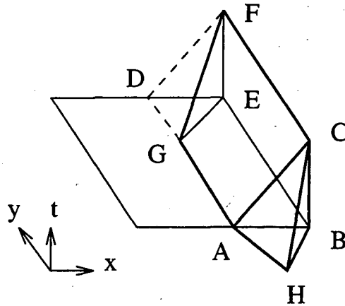
Figure 5.1 In this space-time diagram, the fluid inside the solid fluxes through the right cell edge.
