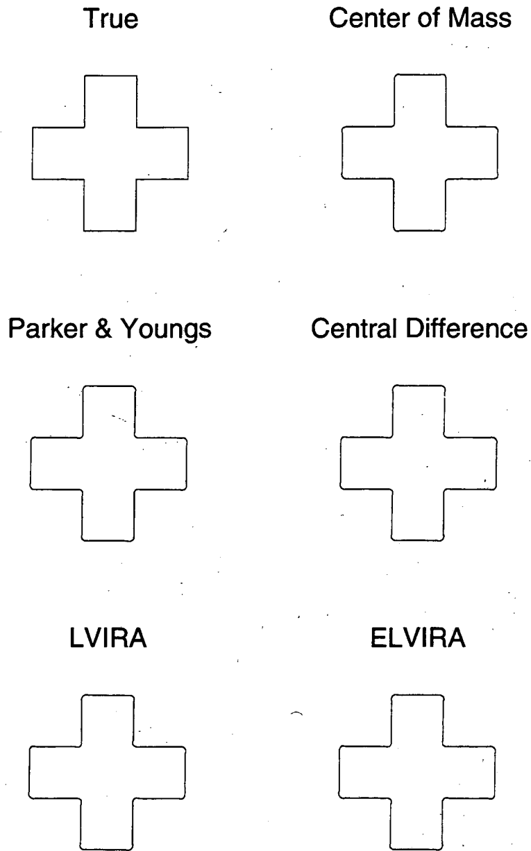
Figure 5.4 A cross that has been rotated one revolution with the usplit advection algorithm and various reconstruction methods. By comparing the results shown here with those shown in Fig. 4.2, one can see that the unsplit advection algorithm produces noticeably better resolution of the corners.
