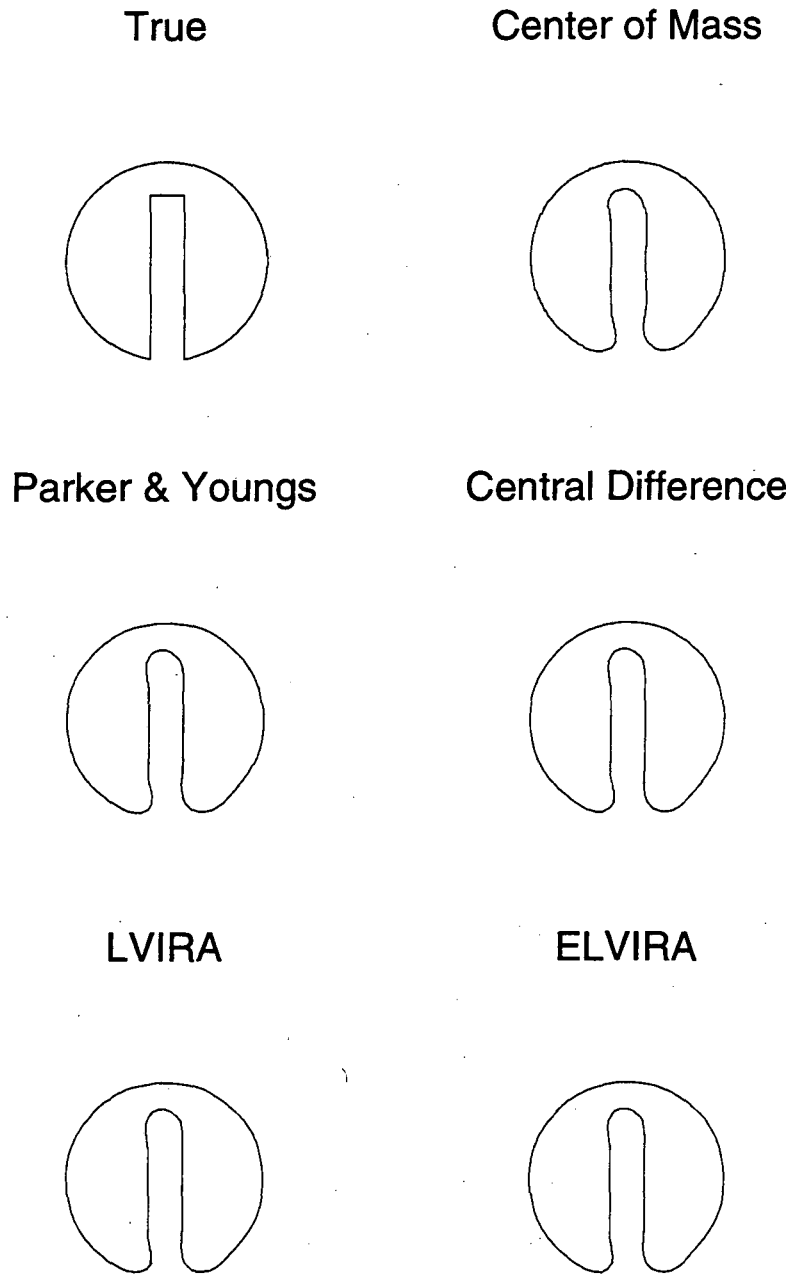
Figure 5.5 Here we present the results of using the unsplit advection algorithm and the various reconstruction methods to compute Zalesak's test problem. Note that the computations shown here and in Fig. 4.3 were conducted on the very coarse grid shown in Fig. 3.1. Consequently one cannot detect the increased resolution at the corners expected from the unsplit advection algorithm. Higher resolution computations of this problem do exhibit better resolution with unsplit algorithm.
