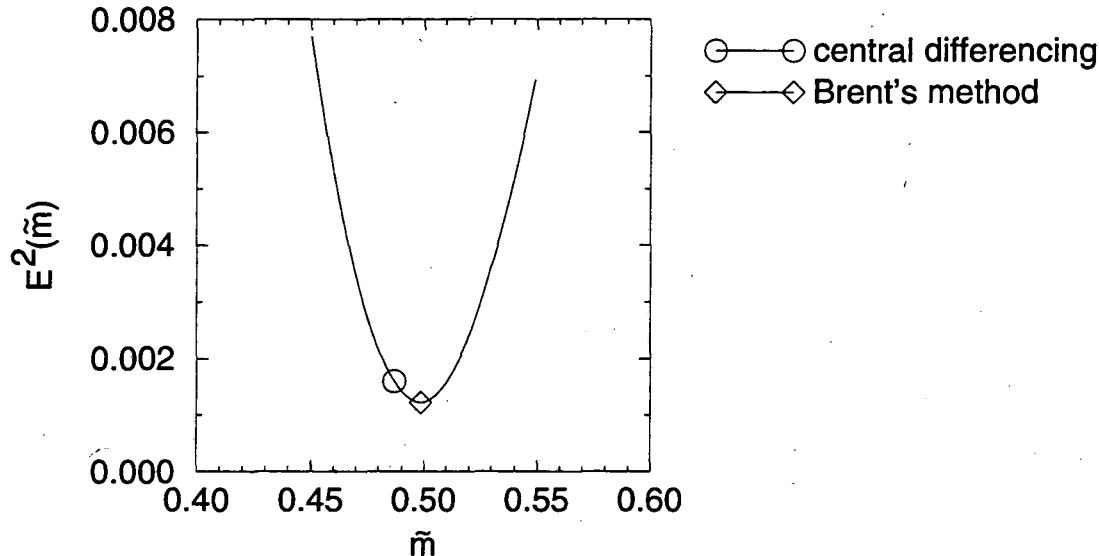
Figure 2.6 We use the centered difference algorithm to obtain a starting point for Brent's method, which we then use to find the minimum of the curve shown in Figure 2.5.
