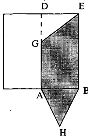
Figure 5.2 Domain of dependence for characteristics passing through the right edge of the cell (i, j) .
