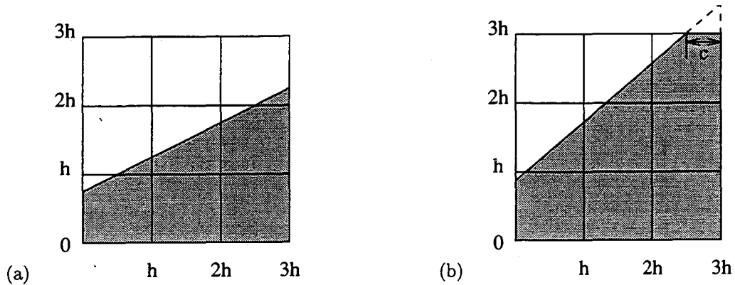
Figure 2.2 (a) Center differences will exactly reconstruct a line that cuts opposite sides of a 3 \times 3 block of cells. (b) It will not exactly reconstruct a line that cuts adjacent sides of a 3 \times 3 block of cells.
