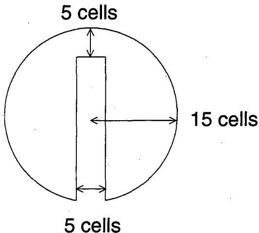
Figure 3.1 The notched circle, first introduced by Zalesak to study the accuracy of advection algorithms, which we use in several of our test problems.
