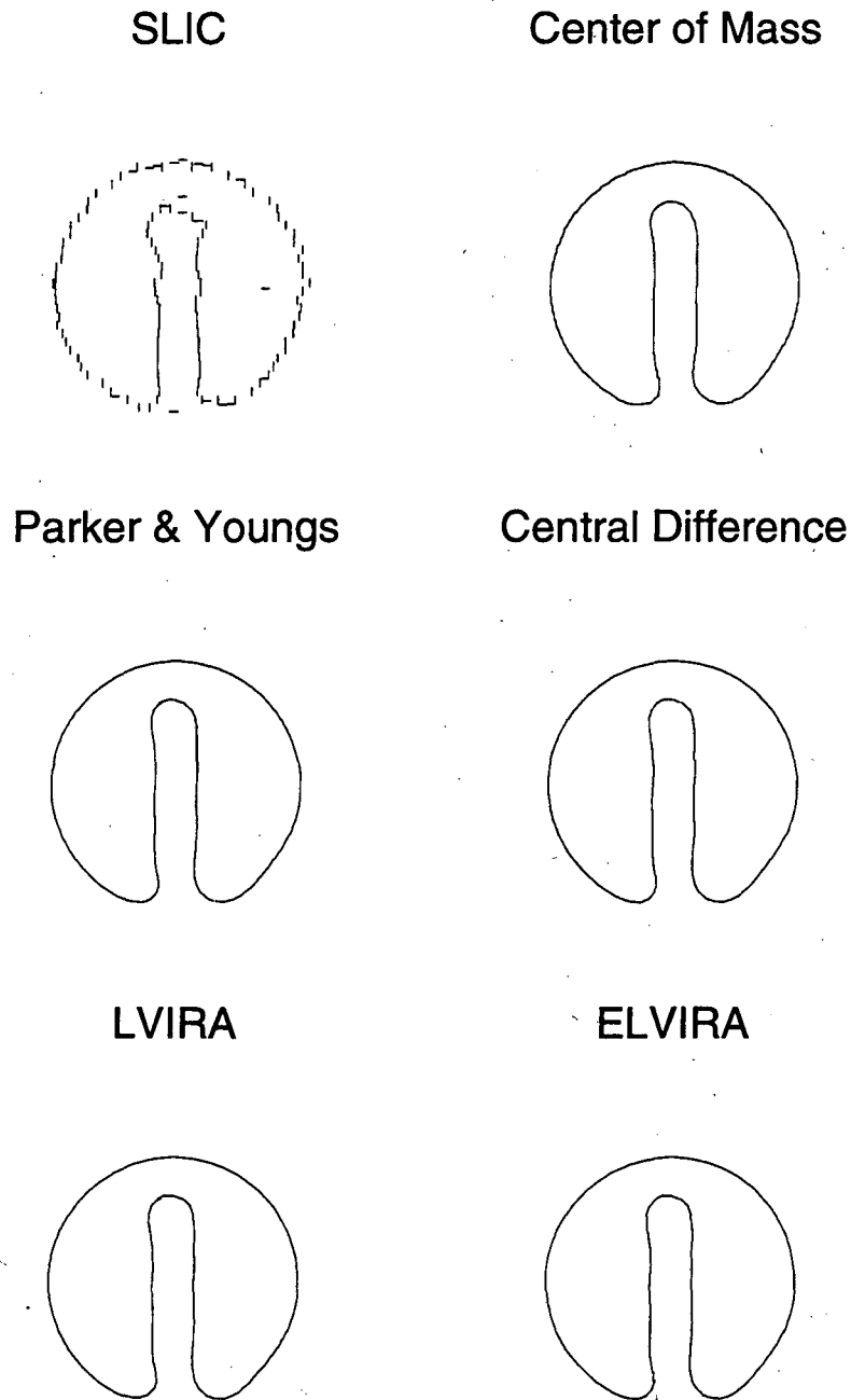
Figure 4.3 The result of using the operator split advection algorithm and the various interface reconstruction methods on Zalesak's test problem. Again notice that only the SLIC algorithm produces flotsam.
