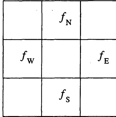
Figure 2.3 The stencil that Parker and Youngs use to determine \nabla f .
