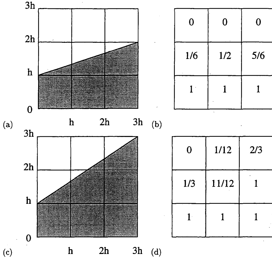
Figure 2.4 (a) Parker and Youngs' method will reconstruct this line exactly only if \alpha = 2 . (b) The volume fractions associated with the line shown in (a). (c) Parker and Youngs' method does not reconstruct this line exactly for \alpha = 2 . Thus it does not reproduce all linear interfaces exactly, and so we conclude it is a first-order method. (d) The volume fractions associated with the line shown in (c).
