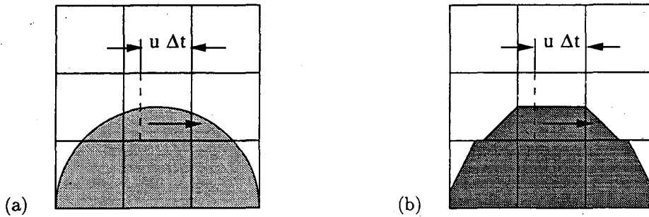
Figure 4.1 (a) In operator split advection, the fluid to the right of the dotted line crosses the right cell edge. (b) In a volume-of-fluid method, we use the reconstructed interface to determine the amount of fluid that crosses each edge.
