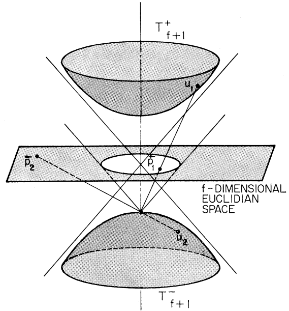
FIG. 1. Stereographic projection of an f -dimensional space to the unit hyperboloid in f+1 dimensions.
